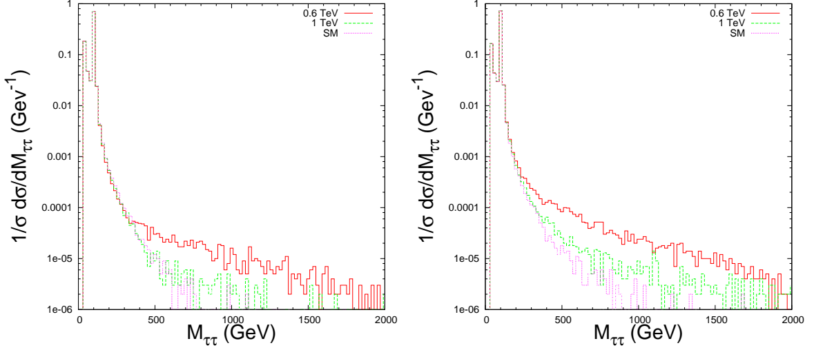
FIG. 8: Dilepton invariant mass distributions for the scenarios LQ-1 and LQ-2 at the LHC with \sqrt{S} = 14 TeV for M_{LQ} = 0.6 and 1 TeV.
