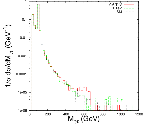
FIG. 4: Dilepton invariant mass distributions for the Z' -model at the LHC with \sqrt{S} = 14 TeV for M_{Z'} = 0.6 and 1 TeV.
