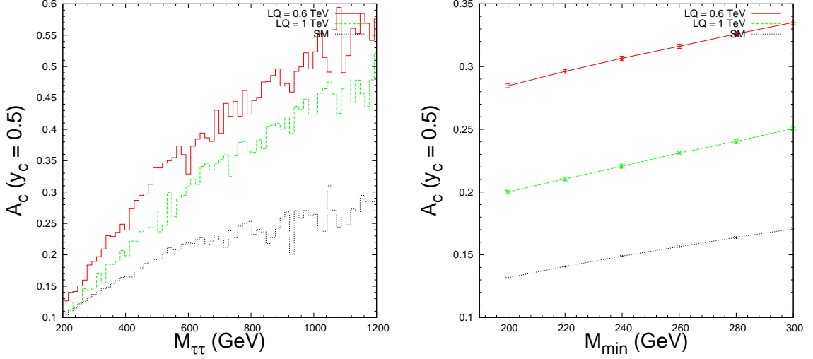
FIG. 10: Integrated charge asymmetry for the lepto-quark model 2 (LQ-2) for M_{LQ} = 0.6, 1 TeV vs M_{\tau\tau} (left) and integrated over M_{\tau\tau} \geq M_{min} (right).
