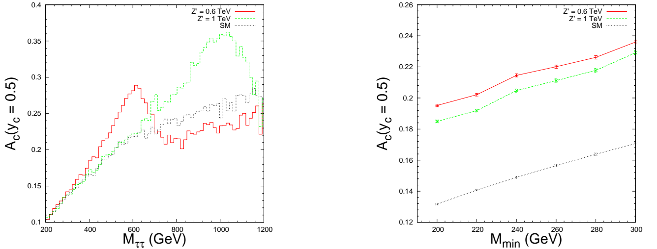
FIG. 5: Lepton charge asymmetry in the Z' model for M_{\tau\tau} > 200 GeV, y_c = 0.5 and M_{Z'} = 0.6 and 1 TeV vs M_{\tau\tau} (left) and integrated over M_{\tau\tau} \geq M_{min} (right). This model has only non-zero couplings as c_R^\tau , and c_R^u such that c_R^\tau \cdot c_R^u = 1/3 .
