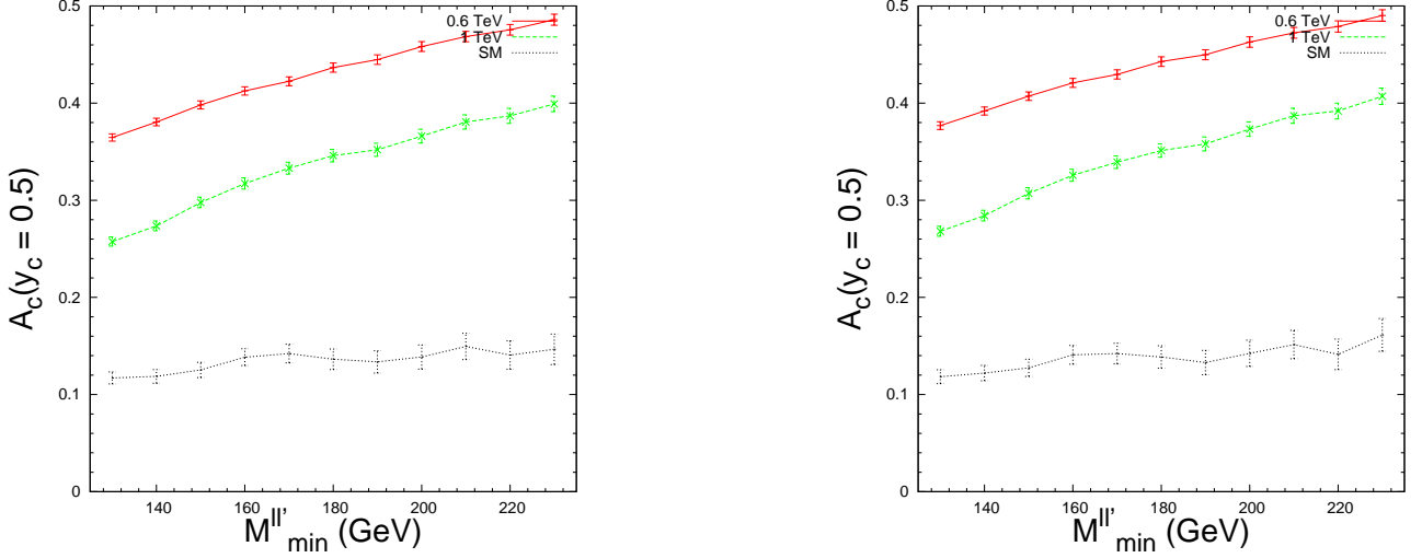
FIG. 12: Charge asymmetry in the dilepton mode with different lepton flavor pair for the SM and the LQ-2 model with two different lepto-quark masses as a function of a minimal M_{\ell\ell'} cut without (left) and with (right) an additional requirement of missing E_T as described in the text. In these plots, \ell = \mu^+, \ell' = e^- .
