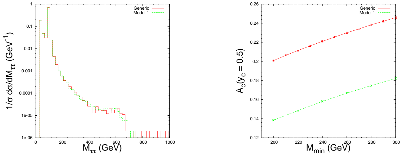
FIG. 6: Comparison of two Z' models with M_{Z'} = 600 GeV in invariant mass distribution M_{\tau\tau} (left) and integrated charge asymmetry (right). The model labeled ‘Generic’ has only non-zero couplings c_R^\tau , and c_R^u such that c_R^\tau \cdot c_R^u = 1/3 . The model labeled ‘Model 1’ is that of Ref. [2].
