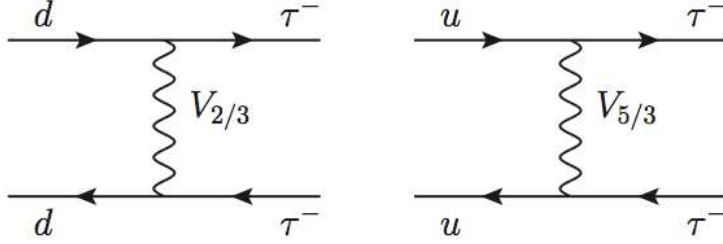
FIG. 7: Feynman diagram for dilepton production through lepto-quark exchange in lepto-quark Model 1 (Left) and 2 (Right).
