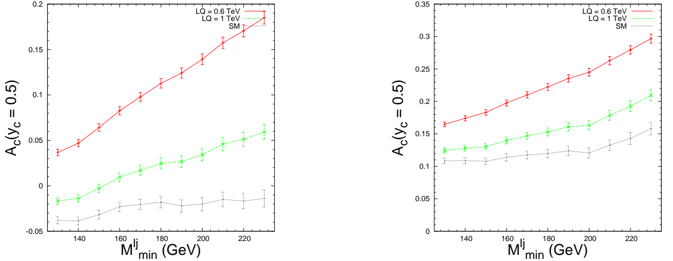
FIG. 13: Charge asymmetry A_{ij} with a missing E_T requirement. The results for \ell^+ j and \ell^- j are shown respectively in the left-side and right-side plots. In both cases \ell^\pm = e^\pm, \mu^\pm and the jet is discussed in the text.
