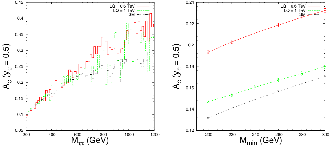
FIG. 9: Integrated charge asymmetry for the lepto-quark model 1 (LQ-1) for M_{LQ} = 0.6, 1 TeV vs M_{\tau\tau} (left) and integrated over M_{\tau\tau} \geq M_{min} (right).
