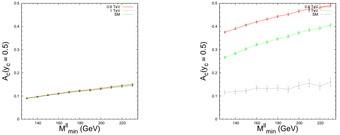
FIG. 11: Charge asymmetry in the dilepton mode with same lepton flavor pair for the SM and the LQ-2 model with two different lepto-quark masses as a function of a minimal M_{\ell\ell} cut without (left) and with (right) an additional requirement of missing E_T as described in the text.
