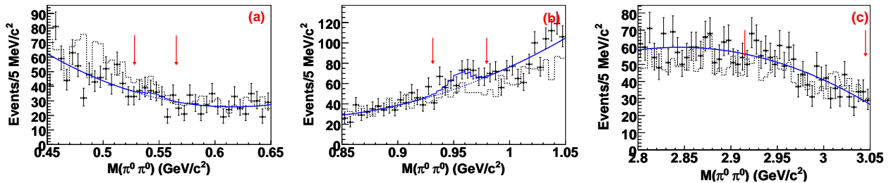
FIG. 2: (a)-(c): The \pi^0\pi^0 invariant mass distributions of the final candidate events in the \eta , \eta' and \eta_c mass regions, respectively. The dots with error bars are data, the solid lines are the fit described in the text, and the dashed histograms are the sum of all the simulated normalized backgrounds. The arrows show mass regions which contain around 95% of the signal according to MC simulations.
