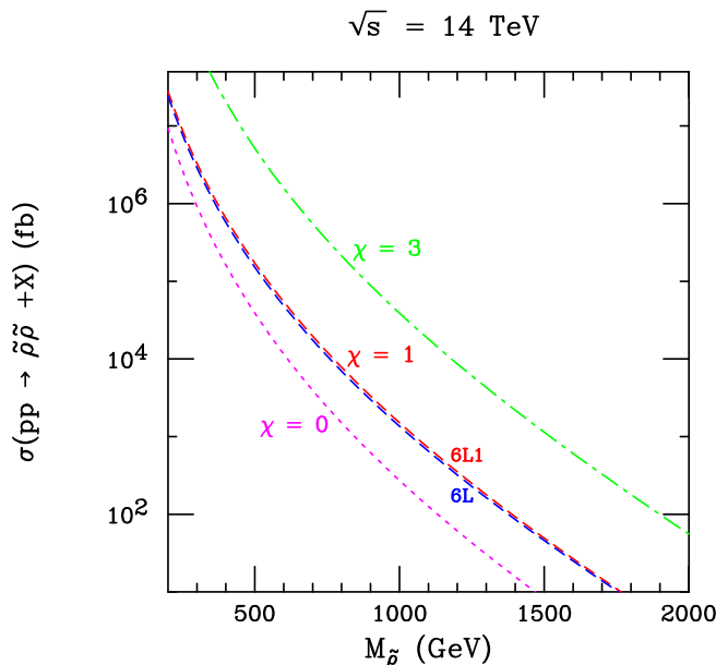
FIG. 8: The cross section of pp \rightarrow \tilde{\rho}\tilde{\rho} + X , as a function of M_{\tilde{\rho}} , for \chi = 1, 0 , and 3.
