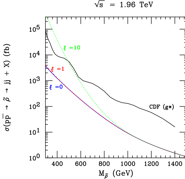
FIG. 10: The cross section of pp \rightarrow \tilde{\rho} \rightarrow jj + X for \xi = 0, 1 , and 10 , compared to exclusion bounds at the Tevatron CDF detector.
