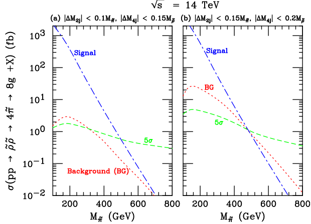
FIG. 16: The cross section for pp \rightarrow \tilde{p}\tilde{p} \rightarrow 4\tilde{\pi} \rightarrow 8g + X (blue dot-dashed line) as a function of M_{\tilde{\pi}} with acceptance cuts on p_T , \eta , and \Delta R . We have applied two sets of fixed mass cuts: (a) |M_{2j} - M_{\tilde{\pi}}| < 0.10M_{\tilde{\pi}} and |M_{4j} - M_{\tilde{\rho}}| < 0.15M_{\tilde{\rho}} , or (b) |M_{2j} - M_{\tilde{\pi}}| < 0.15M_{\tilde{\pi}} and |M_{4j} - M_{\tilde{\rho}}| < 0.20M_{\tilde{\rho}} . This figure differs from Fig.15 in that the p_T cuts used here are p_T(j_1) > 1.5M_{\tilde{\pi}} , p_T(j_2) > 1.2M_{\tilde{\pi}} , p_T(j_3) > M_{\tilde{\pi}} , p_T(j_4) > 0.8M_{\tilde{\pi}} , p_T(j_5, j_6, j_7, j_8) > 50 \text{ GeV} . Also shown are the SM background cross section ( \sigma_b ) (red dotted line) and the minimal signal cross section that is required by a 5 sigma criterion (green dashed line) with an integrated luminosity of 30 \text{ fb}^{-1} .
