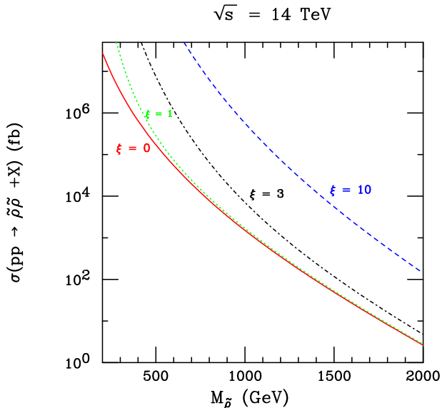
FIG. 9: The cross section of pp \rightarrow \tilde{\rho}\tilde{\rho} + X , as a function of M_{\tilde{\rho}} , for \xi = 0, 1, 3 , and 10 at the LHC with \sqrt{s} = 14 TeV.
