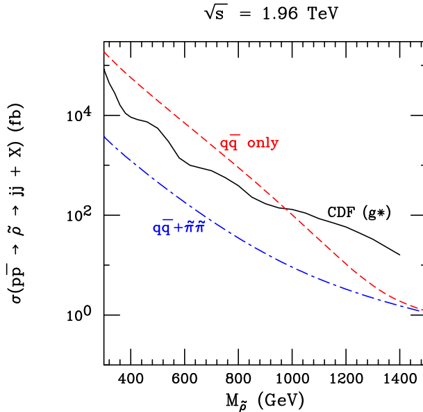
FIG. 1: CDF exclusion limits (black solid line) for dijet-decaying color octets, compared to predicted pp \rightarrow \tilde{\rho} \rightarrow jj + X cross sections computed with \tilde{\pi} decays (blue dot-dashed line) and without \tilde{\pi} decays (red dashed line) for \sqrt{s} = 1.96 TeV.
