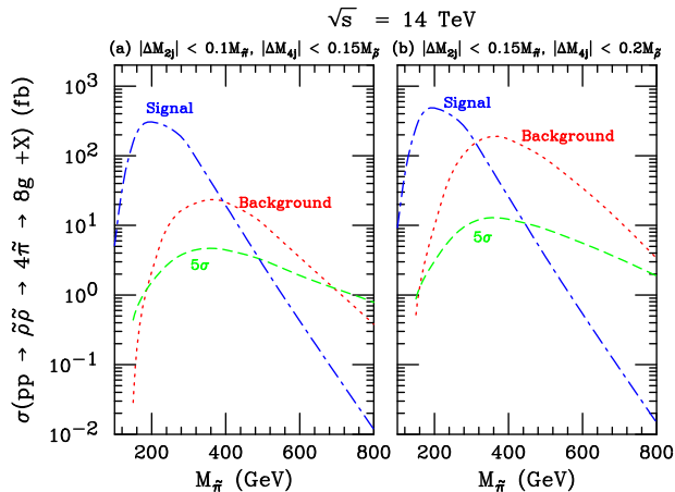
FIG. 15: The cross section for pp \rightarrow \tilde{\rho}\tilde{\rho} \rightarrow 4\tilde{\pi} \rightarrow 8g + X (blue dot-dashed line) as a function of M_{\tilde{\pi}} with acceptance cuts on p_T , \eta , and \Delta R . We have applied two sets of fixed mass cuts: (a) |M_{2j} - M_{\tilde{\pi}}| < 0.10M_{\tilde{\pi}} and |M_{4j} - M_{\tilde{\rho}}| < 0.15M_{\tilde{\rho}} , or (b) |M_{2j} - M_{\tilde{\pi}}| < 0.15M_{\tilde{\pi}} and |M_{4j} - M_{\tilde{\rho}}| < 0.20M_{\tilde{\rho}} . The p_T cuts used were p_T(j_1, \dots, j_8) > 320, 250, 200, 160, 125, 90, 60, 40 GeV. Also shown are the SM background cross section ( \sigma_b ) (red dotted line) and the minimal signal cross section that is required by a 5 sigma criterion (green dashed line) with an integrated luminosity of 30 \text{ fb}^{-1} .
