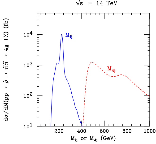
FIG. 6: Invariant mass distribution of two jets ( M_{jj} ) or four jets ( M_{4j} ) from pp \rightarrow \tilde{\rho} \rightarrow \tilde{\pi}\tilde{\pi} \rightarrow 4g + X .
