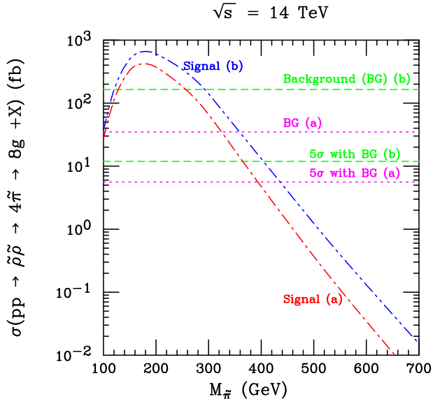
FIG. 14: The cross section for pp \rightarrow \tilde{\rho}\tilde{\rho} \rightarrow 4\tilde{\pi} \rightarrow 8g + X as a function of M_{\tilde{\pi}} . We have applied all kinematic cuts and two sets of relative mass cuts: (a) \Delta M_{2j} < 30 GeV and \Delta M_{4j} < 60 GeV [red dot-dashed line], or (b) \Delta M_{2j} < 50 GeV and \Delta M_{4j} < 100 GeV [blue dot-dot-dashed line]. Also shown are the cross section for the dominant SM background with relative mass cut (a) [magenta dotted line] or (b) [green dashed line] as well as the minimal signal cross section that is required by a 5 sigma criterion with relative mass cut (a) [magenta (lower) dotted line] or (b) [green (lower) dashed line].
