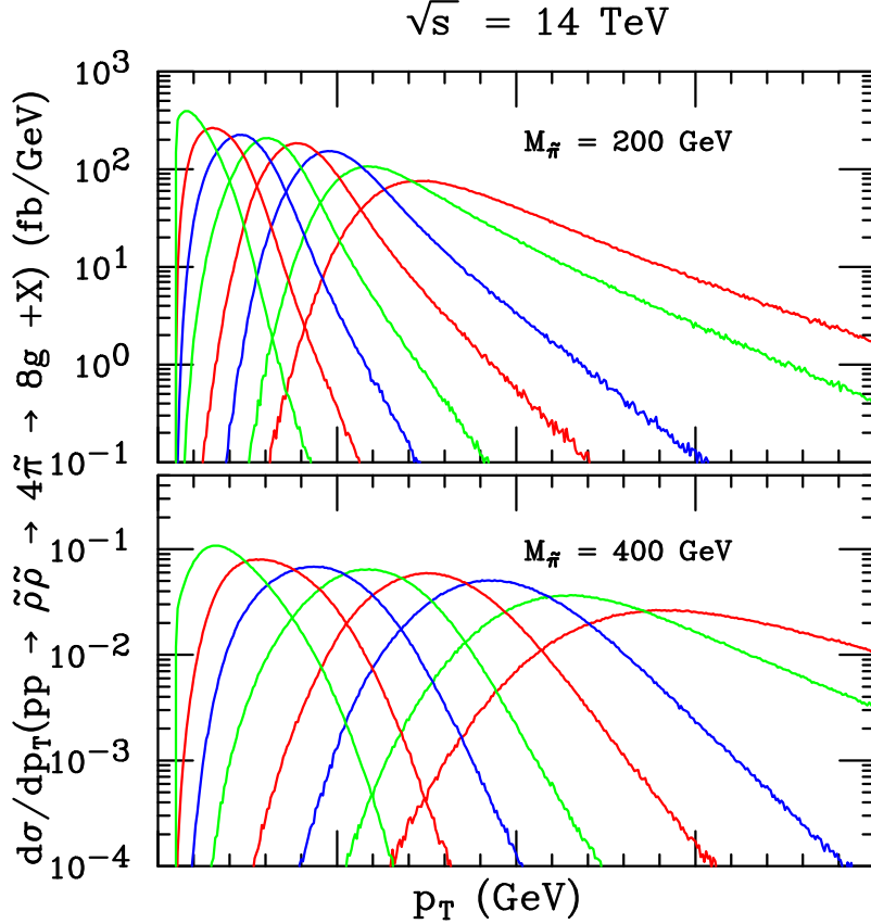
FIG. 11: Transverse momentum ( p_T ) distributions of the eight signal gluons for M_{\tilde{\pi}} = 200 GeV (top) and M_{\tilde{\pi}} = 400 GeV (bottom).
