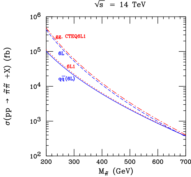
FIG. 3: The cross section of pp \rightarrow \tilde{\pi}\tilde{\pi} + X from gg and q\bar{q} as a function of M_{\tilde{\pi}} . We compare cross sections for two sets of parton distribution functions, CTEQ6L1 and CTEQ6L. [14]
