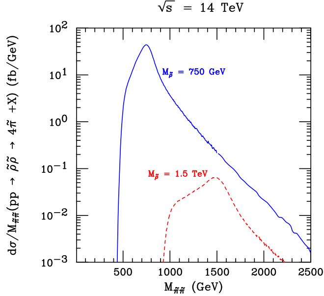
FIG. 7: Invariant mass distribution of two \tilde{\pi} 's for pp \rightarrow 4\tilde{\pi} + X with \sqrt{s} = 14 \text{ TeV} .
