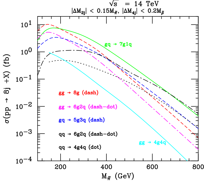
FIG. 13: Individual background channels for pp \rightarrow 8j + X , calculated with fixed mass window cuts and p_T(j_1) > 1.5M_{\tilde{\pi}} , p_T(j_2) > 1.2M_{\tilde{\pi}} , p_T(j_3) > M_{\tilde{\pi}} , p_T(j_4) > 0.8M_{\tilde{\pi}} , p_T(j_5, j_6, j_7, j_8) > 50 \text{ GeV} .
