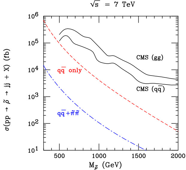
FIG. 2: CMS exclusion limits (black solid line) for dijet-decaying color octets, compared to predicted pp \rightarrow \tilde{\rho} \rightarrow jj + X cross sections computed with \tilde{\pi} decays (blue dot-dashed line) and without \tilde{\pi} decays (red dashed line) for \sqrt{s} = 7 TeV.
