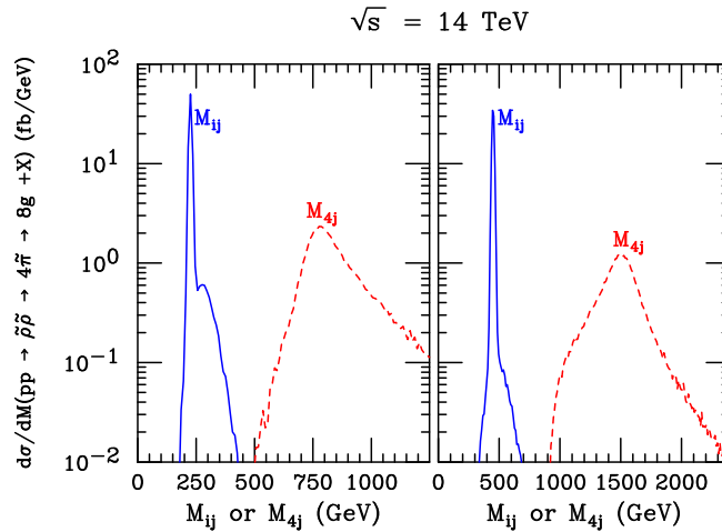
FIG. 12: Invariant mass distribution of two jets or four jets for pp \rightarrow \tilde{\rho}\tilde{\rho} \rightarrow 4\tilde{\pi} \rightarrow 8g + X .
