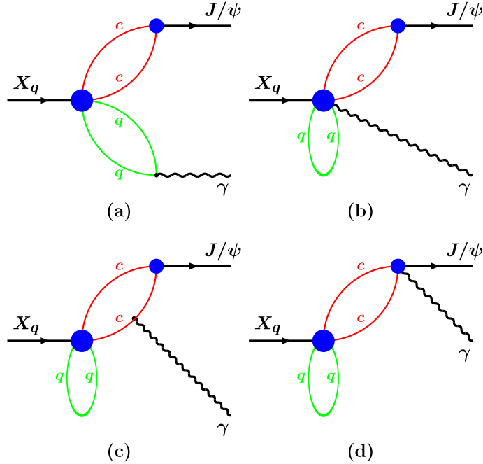
FIG. 1. Feynman diagrams describing the decay X \rightarrow \gamma + J/\psi .
