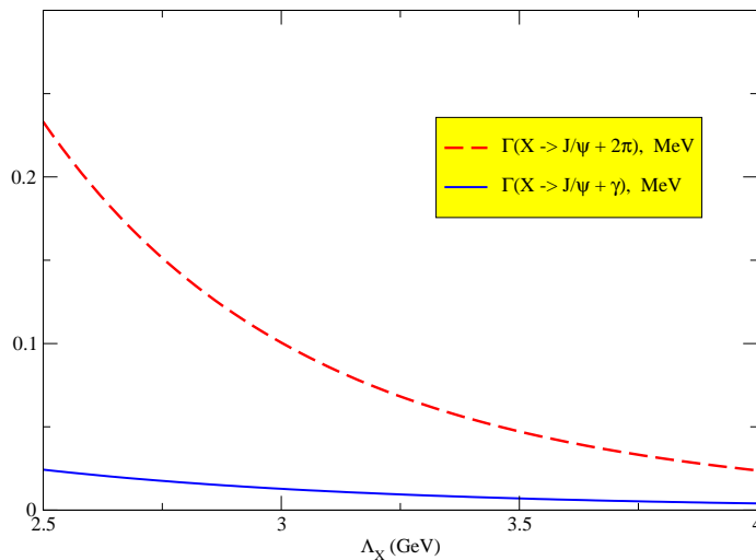
FIG. 2. The dependence of the decay widths \Gamma(X_l \rightarrow \gamma + J/\psi) and \Gamma(X_l \rightarrow J/\psi + 2\pi) on the size parameter \Lambda_X .
