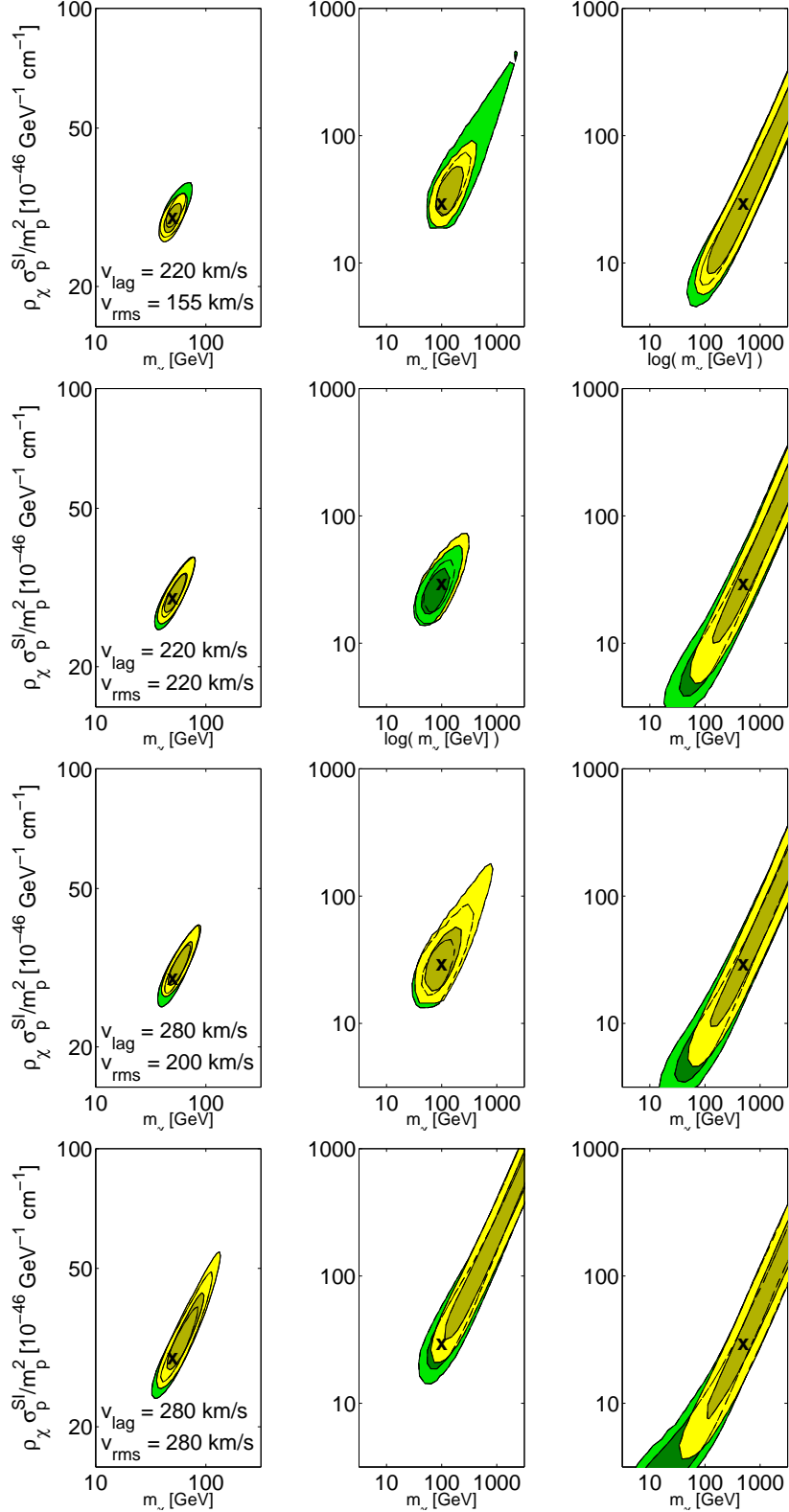
FIG. 4: Marginalized probability distributions for m_\chi and D = \rho_\chi \sigma_P^{SI} / m_p^2 with Maxwellian speed distributions for the WIMPs as the benchmark models and as the hypothesis. The lines outline 68% and 95% C.L. regions. The darker pair of contours is associated with WIMP searches with flat priors on the velocity parameters with Q_{\max} = 1 MeV for all experiments, and the lighter pair are associated with a 10% Gaussian prior on v_{\text{lag}} = 220 km s ^{-1} and a prior on \beta (Eq. 13; see text for details). Each row of figures corresponds to a different benchmark WIMP velocity distribution, and each column represents a different benchmark WIMP mass.
