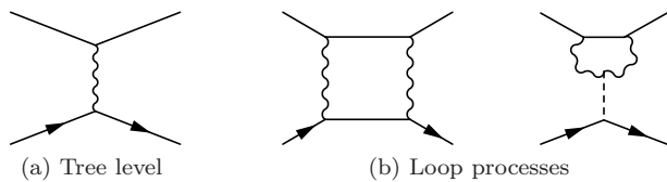
FIG. 1: The tree and loop level contributions to scattering of Majorana fermions through a Z boson. For all box diagrams, the crossed box diagram is included in calculations but not depicted. In the last diagram, a Higgs mediates the scattering through a Z loop.
