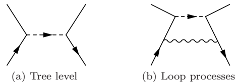
FIG. 2: The tree and loop level contributions to scattering of Majorana fermions through a s -channel scalar.
