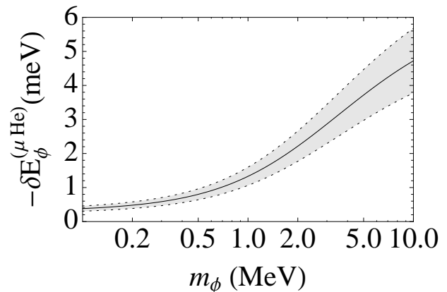
FIG. 2: The contribution to the 2S-2P energy splitting in muonic helium, Eq. (9), plotted against the mediator's mass. The curve is normalized to \delta E_{\mu H} = -0.31 meV, which is the discrepancy between the experimentally measured value and the theoretical prediction, assuming the CODATA value for the proton-radius, r_p = 0.8768 fm. The dotted curves represent the \pm 1 s.d. uncertainty about this value.
