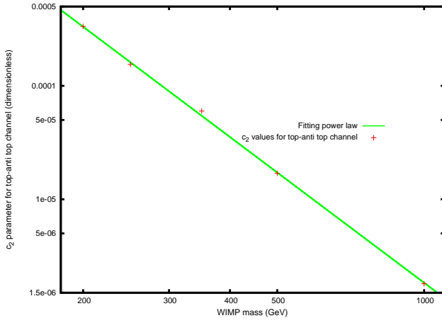
(c) c_2 parameter of expression (6) for t\bar{t} channel. Relative errors of the fitted values range from 6 to 20 % for this parameter.
