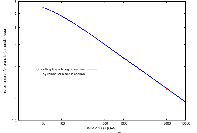
(b) n_1 parameter of expression (6) for b\bar{b} channel. Relative errors of the fitted values range from 1 to 6 % for this parameter.
