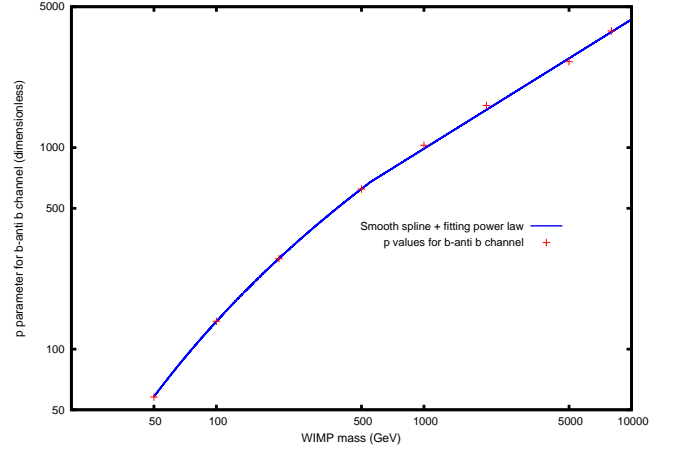
(f) p parameter of expression (6) for b\bar{b} channel. Relative errors of the fitted values range from 1 to 10 % for this parameter.
