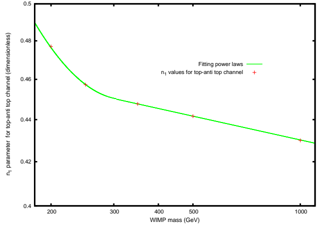
(b) n_1 parameter of expression (6) for t\bar{t} channel. Relative errors of the fitted values range from 1 to 4 % for this parameter.
