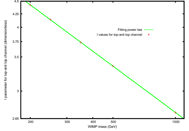
(f) l parameter of expression (6) for t\bar{t} channel. Relative errors of the fitted values are around 1% for this parameter.
