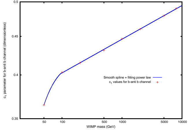
(d) c_1 parameter of expression (6) for b\bar{b} channel. Relative errors of the fitted values are around 3 % for this parameter.
