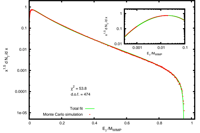
(b) Photon spectrum for M = 200 GeV for W^+W^- channel.
