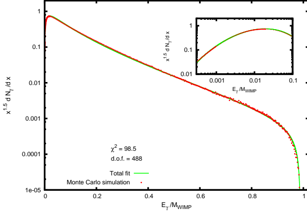
(c) Photon spectrum for M = 350 GeV for W^+W^- channel.
