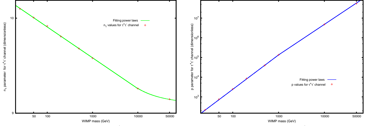
(a) n_1 parameter of expression (6) for \tau^+\tau^- channel. Relative errors of the fitted values range from 2 to 7 % for this parameter.
