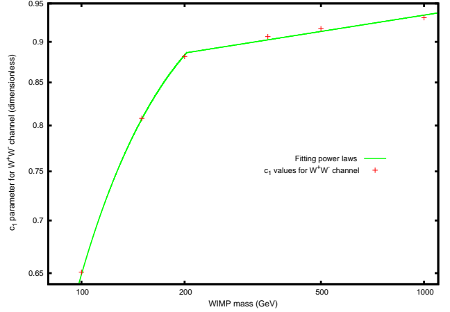
(b) c_1 parameter of expression (6) for W^+W^- channel. Relative errors of the fitted values range from 1 to 2 % for this parameter.
