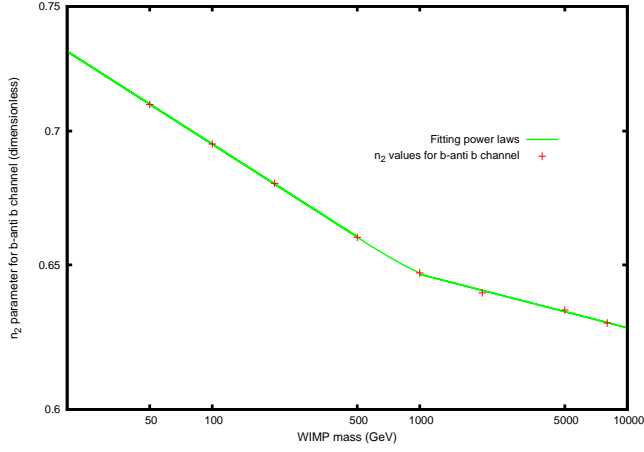
(c) n_2 parameter of expression (6) for b\bar{b} channel. Relative errors of the fitted values range from 1 to 2 % for this parameter.
