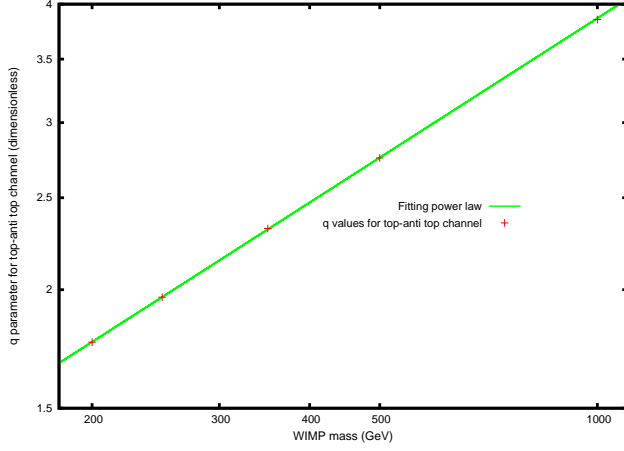
(e) q parameter of expression (6) for t\bar{t} channel. Relative errors of the fitted values range from 2 to 28 % for this parameter.
