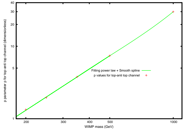
(d) p parameter of expression (6) for t\bar{t} channel. Relative errors of the fitted values range from 1 to 7 % for this parameter.
