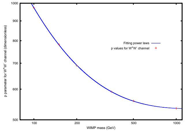
(d) p parameter of expression (6) for W^+W^- channel. Relative errors of the fitted values range from 1 to 2 % for this parameter.
