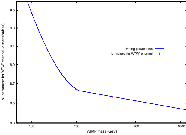
(a) b_1 parameter of expression (6) for W^+W^- channel. Relative errors of the fitted values range from 1 to 2 % for this parameter.
