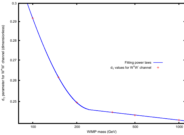
(c) d_1 parameter of expression (6) for W^+W^- channel. Relative errors of the fitted values are around 1 % for this parameter.
