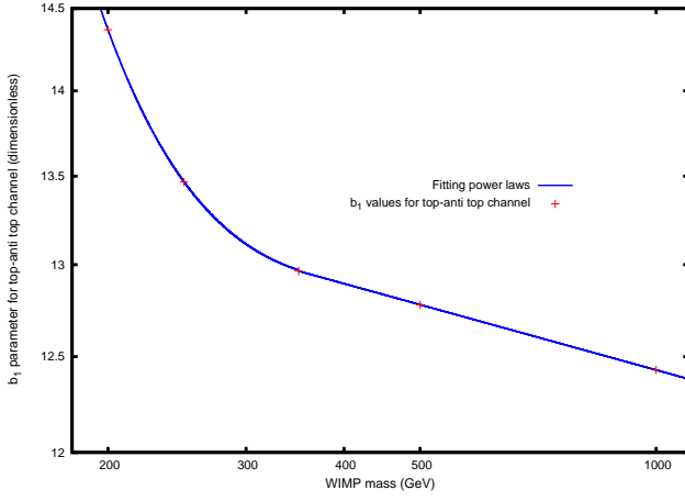
(a) b_1 parameter of expression (6) for t\bar{t} channel. Relative errors of the fitted values range from 1 to 2 % for this parameter.
