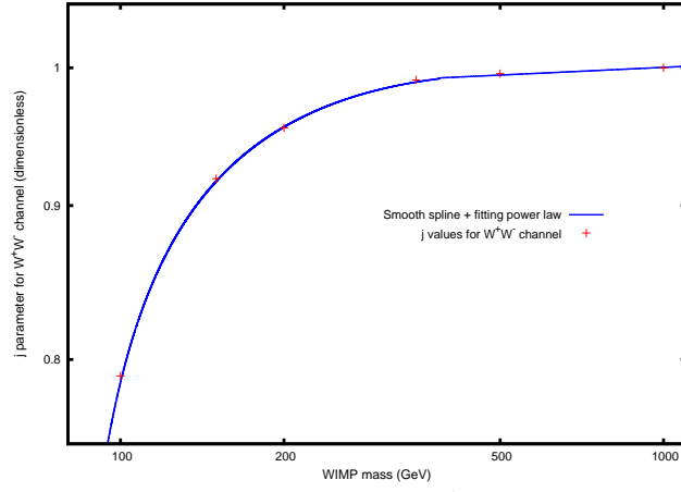
(e) j parameter of expression (6) for W^+W^- channel. Relative errors of the fitted values range from 1 to 3 % for this parameter.
