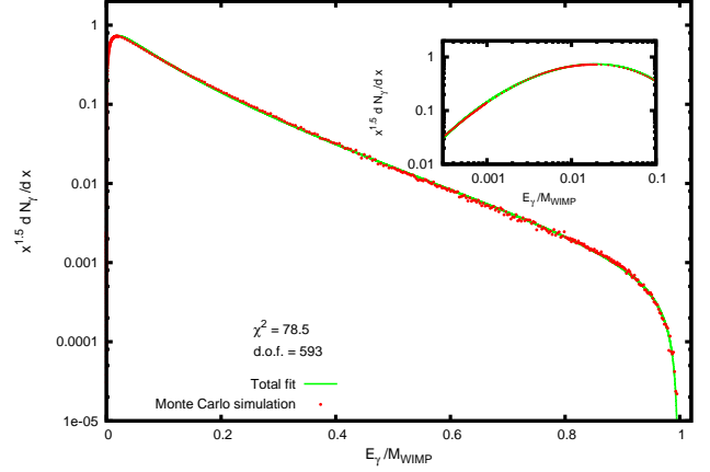
(d) Photon spectrum for M = 1000 GeV for W^+W^- channel.
