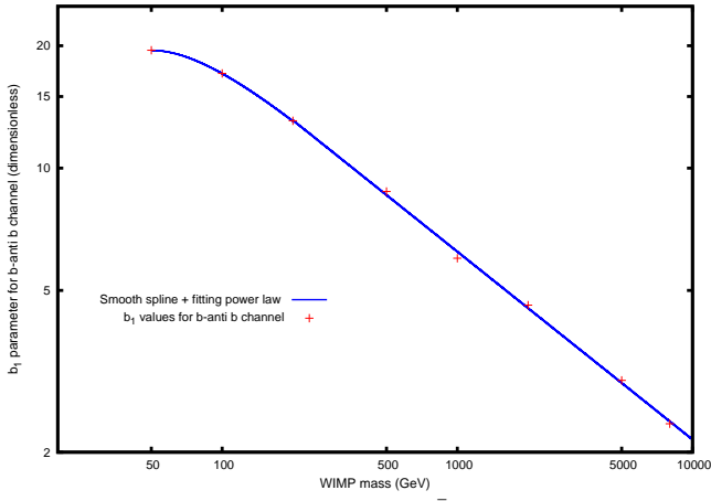
(a) b_1 parameter of expression (6) for b\bar{b} channel. Relative errors of the fitted values range from 5 to 15 % for this parameter.
