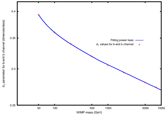
(e) d_1 parameter of expression (6) for b\bar{b} channel. Relative errors of the fitted values are around 1 % for this parameter.
