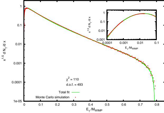
(a) Photon spectrum for M = 100 GeV for W^+W^- channel.
