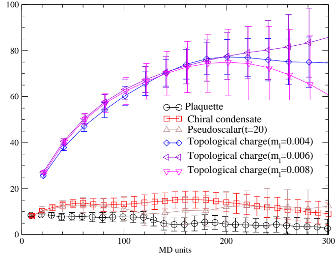
FIG. 2: The integrated autocorrelation time is shown for the average plaquette, chiral condensate \langle \bar{\psi}\psi \rangle , pseudoscalar propagator at time separation 20 from a Gaussian source and point sink, all computed from the 32^3 , m_l = 0.004 ensemble and the global topological charge for all three 32^3 ensembles. The chiral condensate and plaquette are measured every two MD units and the averages within sequential blocks of 10 MD units have been analyzed. The topological charge is measured every 4 MD units and the averages within sequential blocks of 20 MD units have been analyzed. All other quantities were measured every 20 MD units and no averaging has been performed. Further discussion of the topological charge is given in section VII.
