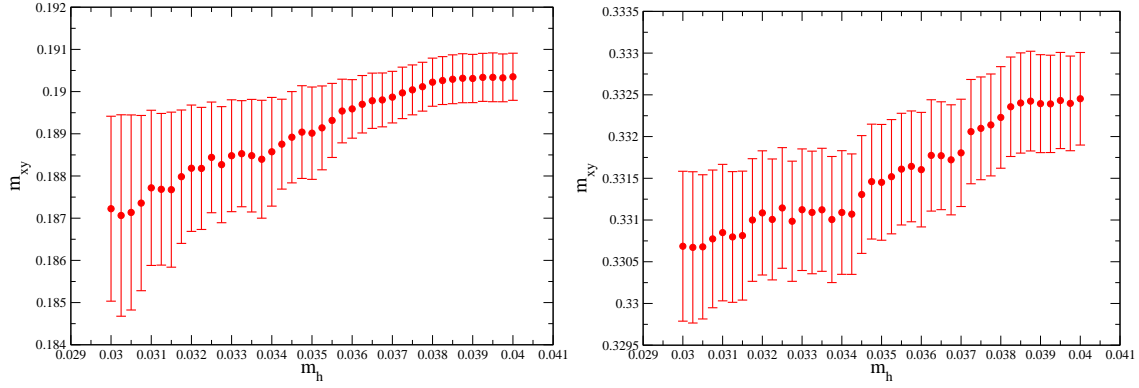
FIG. 13: We illustrate the m_h dependence of the unitary pion (left panel) and kaon (right panel) masses on the m_l = 0.005 , 24^3 ensemble. The values are obtained by reweighting around the simulated value ( m_h = 0.04 ).
