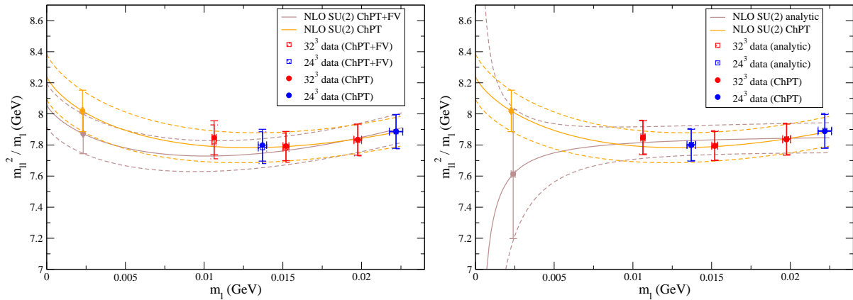
FIG. 31: Left panel: Pion mass fit for the SU(2) NLO fit form in the continuum limit, both with and without finite volume logarithms. We adjust the data points to the continuum limit using the a^2 dependence in our fit form and overlay these. Right panel: Chiral extrapolation of the pion mass using the analytic (52) and infinite-volume NLO ChPT ansätze.
