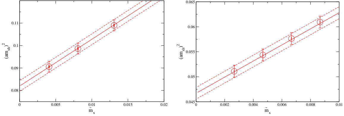
FIG. 39: Dependence of the kaon mass on the mass of the light valence quark with fits performed using finite-volume NLO partially-quenched ChPT. The left panel shows the results from the 24^3 , m_l = 0.005 ensemble and the right panel from the 32^3 , m_l = 0.004 ensemble. In each case the results are for the physical strange-quark mass.
