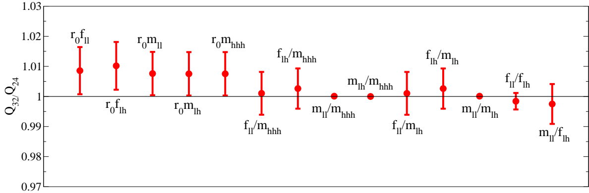
FIG. 26: Ratios of dimensionless combinations of lattice quantities Q (listed in the figure) between the 32^3 and 24^3 lattices at the matching point corresponding to m_l = 0.006 , m_h = 0.03 on the 32^3 lattice. A value of unity indicates perfect scaling. The ratios m_{ll}/m_{hhh} and m_{lh}/m_{hhh} (and consequently m_{ll}/m_{lh} ) are defined to scale perfectly at these quark masses as a consequence of our choice of scaling trajectory.
