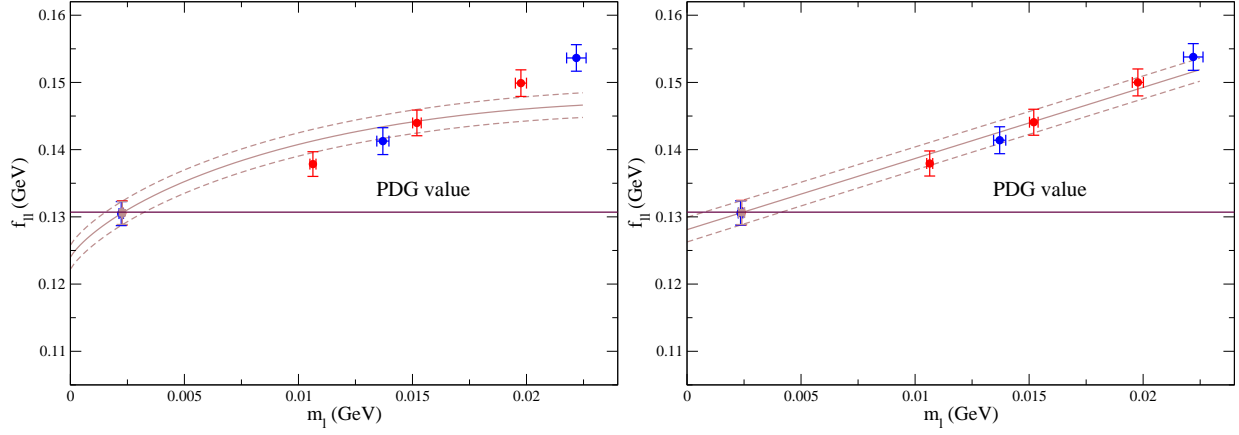
FIG. 37: An artificial data point (the left-most data point in each panel) corresponding to the physical value of f_\pi [45], but including our uncertainties in the lattice spacing, is added to the data for the pion decay constant from the five ensembles. The left-hand panel corresponds to the NLO SU(2) ChPT fits and the right-hand panel to the analytic ansatz.
