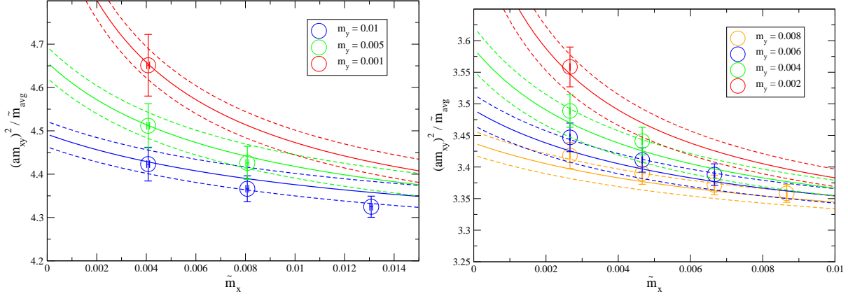
FIG. 30: Global fit curves obtained using the analytic fit ansatz (49) overlaying the simulated pion masses on the m_l = 0.005 , 24^3 ensemble (top-left) and the m_l = 0.004 , 32^3 ensemble (top-right). Points marked by circles were included in the fit, those marked by diamonds were not. The simple linear expansion replicates the entire range of lattice data reasonably well with the description being rather better than NLO chiral perturbation theory at our larger masses. In the bottom two panels we zoom into the low-mass region, illustrating the fits to the points which were included ( 24^3 points on the left and 32^3 points on the right). (For fixed \tilde{m}_x , m_y decreases as (am_{xy})^2/\tilde{m}_{\text{avg}} increases.)
