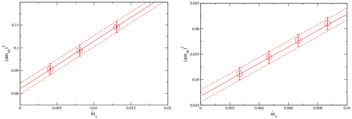
FIG. 38: Dependence of the kaon mass on the mass of the light valence quark with fits performed using infinite-volume NLO partially-quenched ChPT. The left panel shows the results from the 24^3 , m_l = 0.005 ensemble and the right panel from the 32^3 , m_l = 0.004 ensemble. In each case the results are for the physical strange-quark mass.
