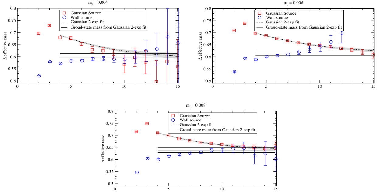
FIG. 25: \Delta effective mass plots from the 32^3 ensembles.
