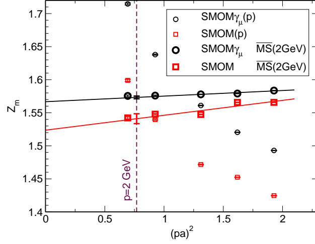
FIG. 50: Z_m^{\text{SMOM}_{\gamma_\mu}}(\mu) and Z_m^{\text{SMOM}}(\mu) as functions of \mu^2 = p^2 , and Z_m^{\overline{\text{MS}}}(2\text{GeV}) from the SMOM or \text{SMOM}_{\gamma_\mu} schemes as function of matching scale squared p^2 for the fine lattice. The interpolation points are shown with the error bar at p^2 = (2 \text{ GeV})^2 .
