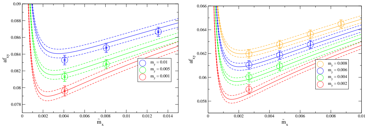
FIG. 32: Global fits to the lattice data for the pion decay constant obtained using infinite-volume NLO SU(2) chiral perturbation theory. The top-left and top-right panels correspond to the 24^3 , m_l = 0.005 and 32^3 , m_l = 0.004 ensembles respectively. Points marked by circles are included in the fits, while those with heavier masses marked by diamonds are not. In the bottom two panels we zoom into the low-mass region, illustrating the fits to the points which were included ( 24^3 points on the left and 32^3 points on the right). (For fixed \tilde{m}_\pi , m_y increases as af_{\pi} increases.)
