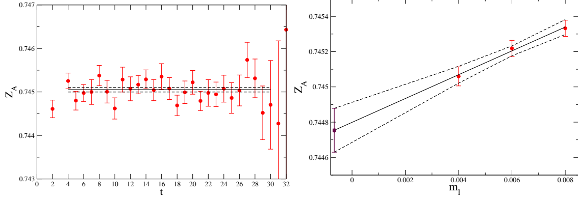
FIG. 18: Measurement of Z_A for m_f = 0.004 on the m_l = 0.004, m_h = 0.03 ensemble (left panel) and the unitary chiral extrapolation of Z_A for the 32^3 ensemble set (right panel). The results do not change significantly under reweighting to the physical strange mass.
