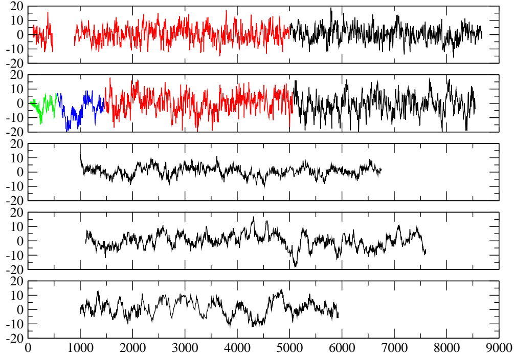
FIG. 52: Monte Carlo time histories of the topological charge. The light sea quark mass increases from top to bottom, (0.005 and 0.01, 24^3 (top two panels), and 0.004-0.008, 32^3 ). Data for the 24^3 ensembles up to trajectory 5000 were reported originally in [1] and the results from the new ensembles are plotted in black. Most of the data was generated using the RHMC II algorithm (red and black lines). The RHMC 0 (green line) and RHMC I (blue line) algorithms were used for trajectories up to 1455 for the m_l = 0.01 ensemble. The small gap in the top panel represents missing measurements which are irrelevant since observables are always calculated starting from trajectory 1000.
