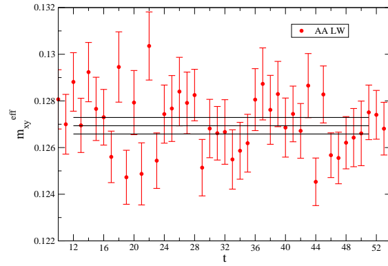
FIG. 19: Effective pion masses from the PP LW correlator (top left), PP WW correlator (top right), AP LW correlator (center left), AP WW (center right) and AA LW correlator (bottom). Note the different vertical scale for the WW correlators. The horizontal bands represent the result for the mass from a simultaneous fit.
