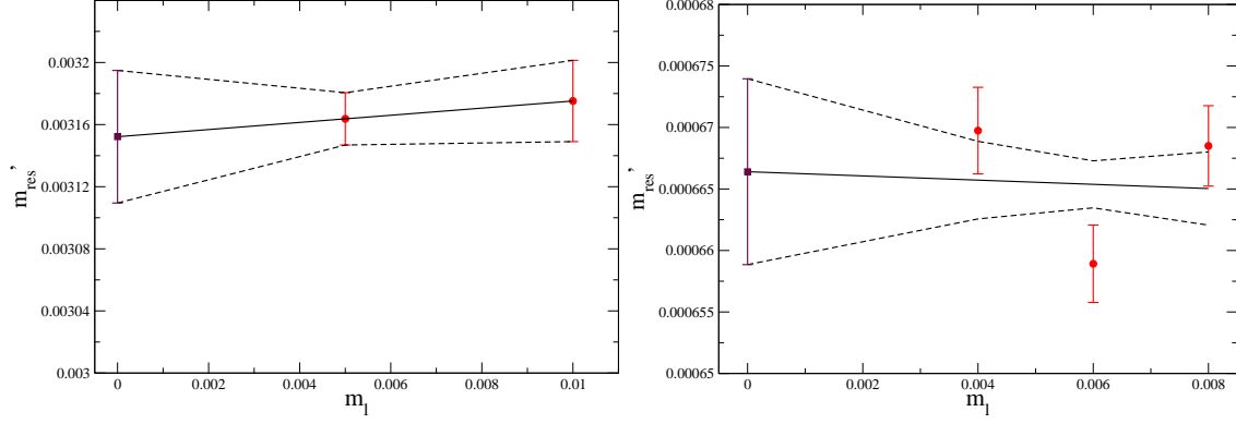
FIG. 9: Chiral extrapolation of the unitary values of m'_{\text{res}} for the 24^3 (left) and 32^3 (right) ensembles. While the fit is only marginally acceptable for the 32^3 lattices, an additional uncertainty of O(5 \times 10^{-6}) is negligible.
