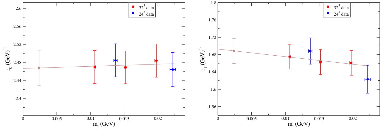
FIG. 47: The scales r_0 (left) and r_1 (right) corrected to the continuum limit, overlaid by the chiral/continuum fit. The extrapolated point at the physical light quark mass is shown as the grey cross. Here the lattice spacings and physical light quark mass were obtained from the global fits using the analytic ansatz. The fits using the quantities obtained with the ChPT and ChPT-fv global fit ansätze are almost indistinguishable from those shown in these figures.
