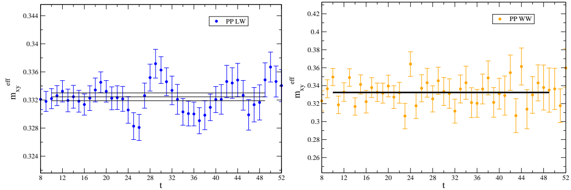
FIG. 11: Effective pion masses from the PP LW correlator (top left), PP WW correlator (top right), AP LW correlator (center left), AP WW (center right) and AA LW correlator (bottom). Note the different vertical scale for the WW correlators. The horizontal bands represent the result for the mass from a simultaneous fit.
