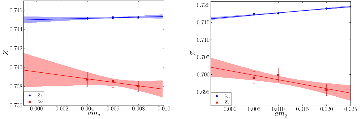
FIG. 59: The quantities Z_A/Z_d and Z_V/Z_V extrapolated to the chiral limit for the 32^3 (left panel) and 24^3 (right panel) ensembles.
