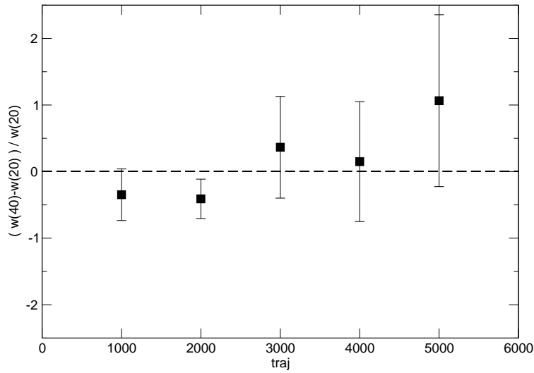
FIG. 4: The relative differences between the reweighting factors for N_{rw} = 20, N_\xi = 4 and N_{rw} = 40, N_\xi = 2 on five lattices. The target and simulation quark masses are m_h = 0.035 and m_h^{(\text{sim})} = 0.040 .
