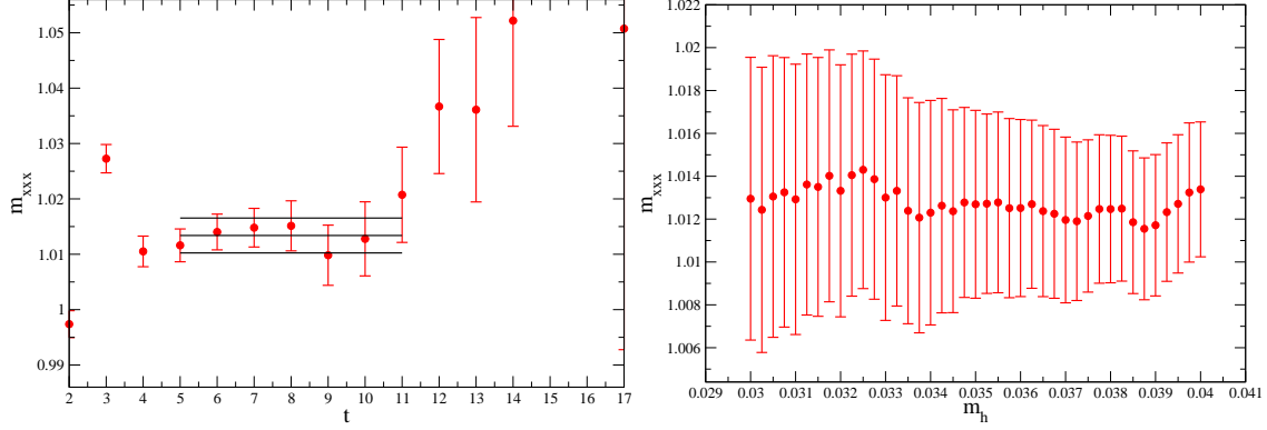
FIG. 14: Fit to the \Omega baryon mass with valence strange mass m_x = 0.04 on the m_l = 0.005 , m_h = 0.04 , 24^3 ensemble showing the quality of the fit with our box source (left panel). We also show the weak dependence of the \Omega baryon mass with fixed valence mass m_x = 0.04 on our simulated m_h inferred by the reweighting procedure on the m_l = 0.005 , 24^3 ensemble (right panel).
