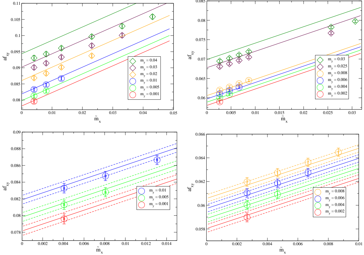
FIG. 34: Global fits to the lattice data for the pion decay constant obtained using the analytic ansatz in Eq. (52). The top-left and top-right panels correspond to the 24^3 , m_l = 0.005 and 32^3 , m_l = 0.004 ensembles respectively. Points marked by circles are included in the fits, while those with heavier masses marked by diamonds are not. In the bottom two panels we zoom into the low-mass region, illustrating the fits to the points which were included ( 24^3 points on the left and 32^3 points on the right). (For fixed \tilde{m}_x , m_y increases as af_{xy} increases.)
