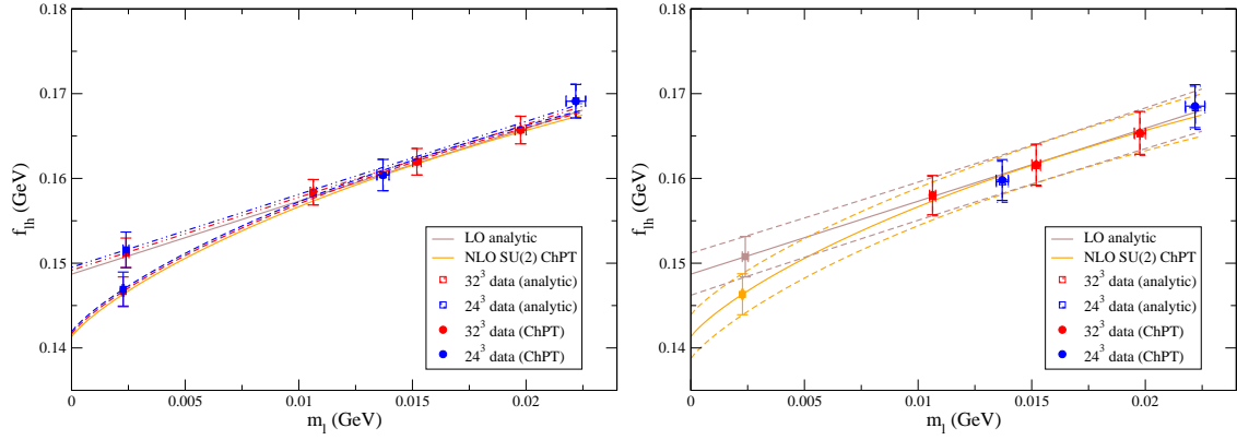
FIG. 46: Chiral extrapolation of the kaon decay constant for unitary data in the continuum limit. We compare the NLO ChPT ansatz to the analytic ansatz. The left panel displays the data and fits at non-zero lattice spacing, while the right panel displays the predicted results and correspondingly adjusted data points for the continuum limit.
