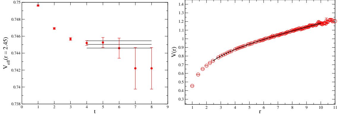
FIG. 23: The effective potential of the Wilson loops with a spatial extent of r = 2.45 on the m_l = 0.004 ensemble at the physical strange-quark mass, overlaid by the fit to the range t = 4 - 8 (left panel). The right panel shows the static inter-quark potential V(r) on this ensemble, again at the physical strange-quark mass, as a function of the spatial extent of the Wilson loops, overlaid by the fit to the Cornell form over the range r = 2.45 - 10 .
