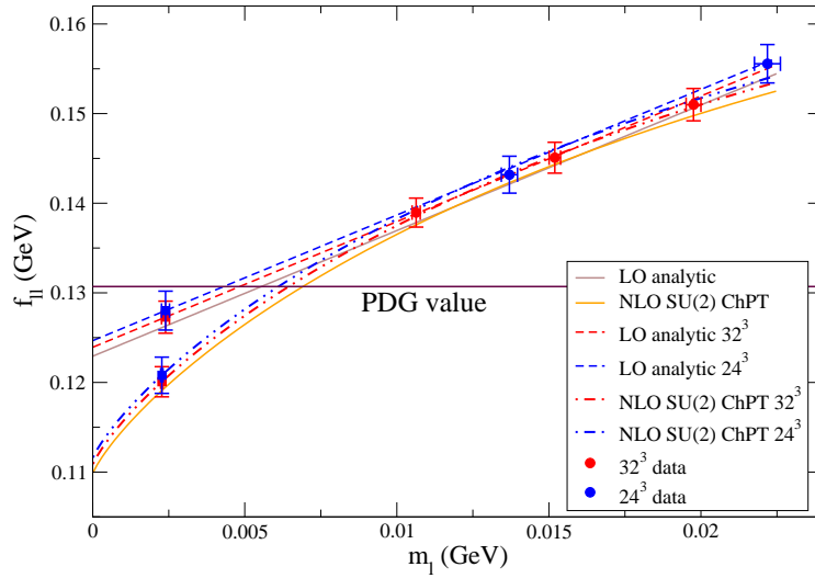
FIG. 36: Chiral extrapolation of the pion decay constant using the analytic (52) and ChPT (42) fit ansätze. Here, the lattice results from the 24^3 and 32^3 ensembles are shown along with the mass dependence we infer both at each lattice spacing and in the continuum limit. The consistency of the two ensembles with each other and with this continuum limit is indicative of the size of lattice artefacts. The horizontal solid line indicates the value f_{\pi^-} = (130.4 \pm 0.04 \pm 0.2) MeV [45].
