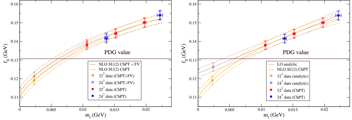
FIG. 35: Unitary data for f_\pi adjusted to the continuum limit using each of the fit ansätze. The left panel compares the infinite volume and finite volume forms of the NLO SU(2) fit, while the right panel compares the analytic fit to the infinite volume NLO SU(2) fit. The horizontal solid line indicates the value f_{\pi^-} = 130.4 MeV (the authors of ref. [45] quote f_{\pi^-} = (130.4 \pm 0.04 \pm 0.2) MeV).
