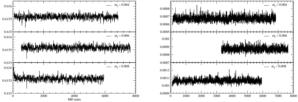
FIG. 1: Evolution of the average plaquette (left panel) and the chiral condensate (right panel) for the \beta = 2.25 , 32^3 \times 64 , L_s = 16 ensembles. The chiral condensate is normalized such that \langle \bar{\psi}\psi \rangle \sim 1/m in the heavy quark limit.
