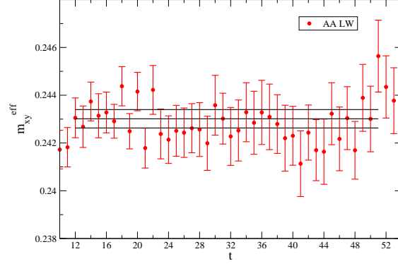
FIG. 20: Effective kaon masses from the PP LW correlator (top left), PP WW correlator (top right), AP LW correlator (center left), AP WW (center right) and AA LW correlator (bottom). Note the different vertical scale for the WW correlators. The horizontal bands represent the result for the mass from a simultaneous fit.
