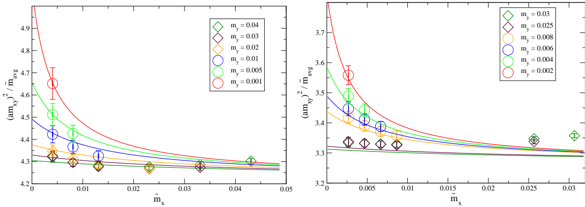
FIG. 29: Global fits for the pion mass obtained using NLO SU(2) chiral perturbation theory with finite-volume corrections. In this case we only include the points which were included in the fit ( m_l = 0.005 , 24^3 points on the left and m_l = 0.004 , 32^3 points on the right) since the finite-volume corrections at larger masses are small. (For fixed \tilde{m}_x , m_y decreases as (am_{xy})^2/\tilde{m}_{\text{avg}} increases.)
