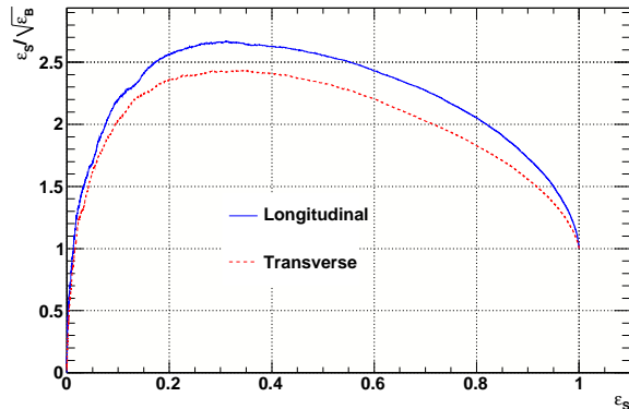
FIG. 18: The SIC using BDTs as a function of signal efficiency for transverse and longitudinally polarized W 's. This is for p_T^{\text{jet}} \in (500, 550) GeV and these gains are on top of the factors of \sim 2 or \sim 2.5 for the two samples from filtering, as shown in Figure 17 (b).
