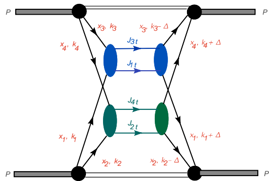
FIG. 1: Kinematics of double hard collision - momenta of the colliding partons in in and out states
