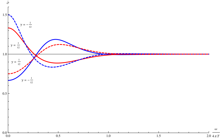
Figure 5: The (dimensionless) conductivity \tilde{\sigma} = g_4^2 \sigma is plotted versus the (dimensionless) frequency \mathbf{w} = \omega/(4\pi T) for various values of \gamma . The solid curves correspond to the same conductivities displayed previously in Fig. 1 — red for \gamma = 1/12 and blue for \gamma = -1/12 . The dashed curves show the conductivity calculated from the EM dual theory for the same values of \gamma .
