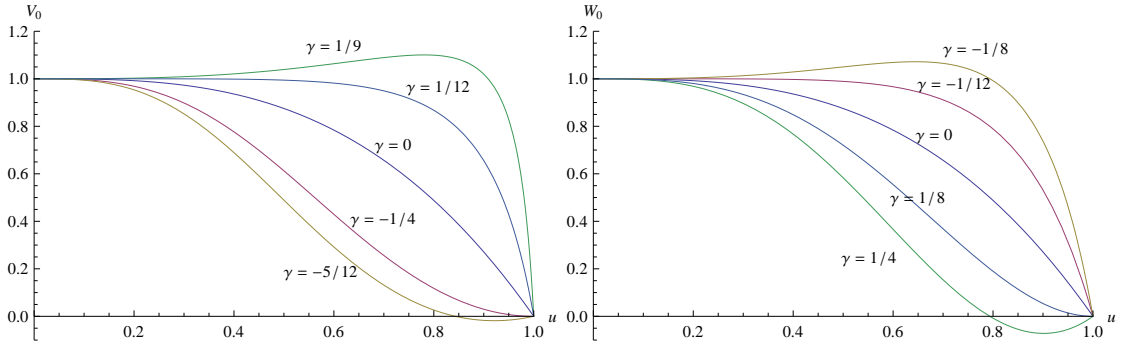
Figure 3: Left: V_0(u) for longitudinal A_t mode for various values of \gamma . Right: W_0(u) for transverse A_y mode for various values of \gamma . Consistency conditions discussed in the text for the longitudinal mode imply \gamma \in [-1/4, 1/12] in V_0 . Similarly for transverse mode, \gamma \in [-1/12, 1/8] in W_0 .
