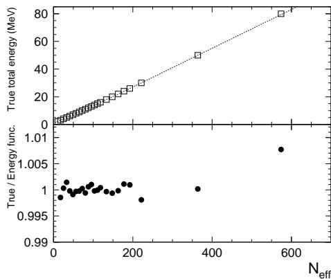
FIG. 6: Relation between N_{eff} and the true total electron energy (MeV) obtained from MC simulation. The dotted line in the upper figure shows the fitted polynomial function. The lower figure shows the deviation of the reconstructed energy from the polynomial function.
