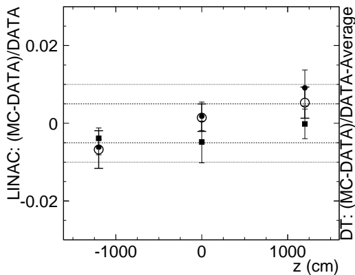
FIG. 8: The z dependence of the energy scale measured by LINAC calibration. The marker shows an average of (MC-DATA)/DATA over four energies at each data-taking point. The error bars show the RMS of (MC-DATA)/DATA for four energies. The filled circle markers are for R=4 m ( x=-4 m, y=0 m) and the square markers are for r=12 m ( x=-12 m, y=0 m). The open circle markers show the z dependence obtained by DT calibration. The dashed and dotted lines show \pm 1 and 0.5\% , respectively. The edge of the fiducial volume is the same as the edge of the plot window (from -1610 cm to 1610 cm).
