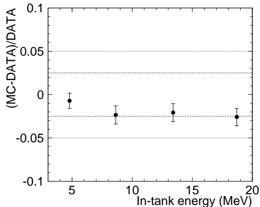
FIG. 11: Energy resolution difference between MC simulation and data as a function of energy, obtained by LINAC calibration.
