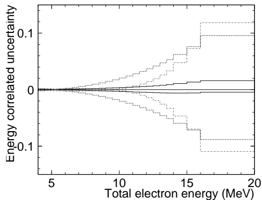
FIG. 25: Energy-correlated systematic uncertainties. The solid, dotted, and dashed lines show the uncertainties of the ^8\text{B} spectrum, the energy scale, and the energy resolution, respectively.
