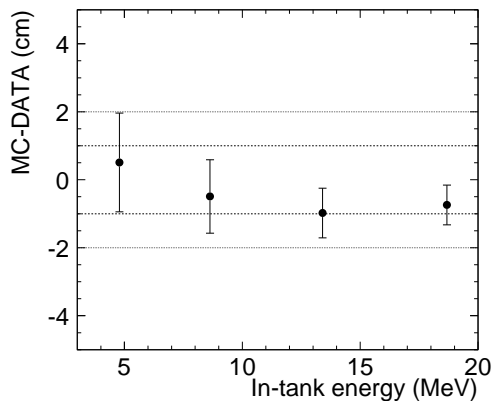
FIG. 24: The difference of vertex resolution between MC simulation and data as a function of energy obtained by LINAC calibration. The dashed line and the dotted line show 1 cm and 2 cm difference respectively.
