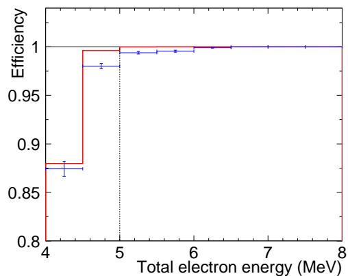
FIG. 12: Trigger efficiency as a function of energy. Markers are ^{16}\text{N} calibration data and the solid histogram is MC simulation. The vertical dashed line shows the analysis threshold, 5.0 MeV.
