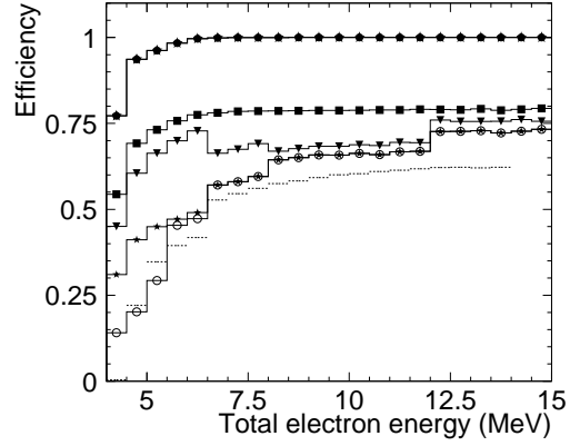
FIG. 21: Reduction efficiency for the solar neutrino MC simulation. The definition of each histogram is the same as for Figure 20.
