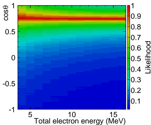
FIG. 4: Likelihood value for reconstruction of event direction as a function of the reconstructed total electron energy and opening angle between the reconstructed direction and the direction from vertex to each hit PMT.
