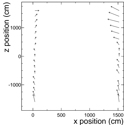
FIG. 2: Vertex shift of Ni calibration events. The origin of the arrows shows the true Ni source position and the direction indicates the averaged reconstructed position direction. The length of the arrow indicates the magnitude of the vertex shift. All vertex shifts are scaled by a factor of 20 to make them easier to see.
