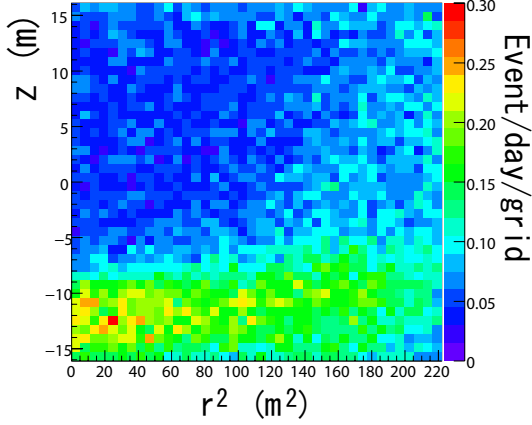
FIG. 19: Vertex distribution of final data sample in the 5.0-6.5 MeV energy region (22.5 kton fiducial volume).
