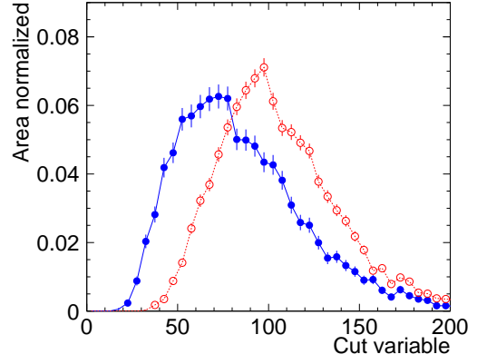
FIG. 17: Distribution of cut variable for the small clustered hit cut. Blue (filled circle) shows background sample events which are selected from r > 12 m and z > -3 m. Red (open circle) shows the solar neutrino MC simulation and the same volume cut is applied. For both data and MC events, event selection cuts up to the external event cut are applied. The reconstructed energies of these samples are in 5.0-6.5 MeV.
