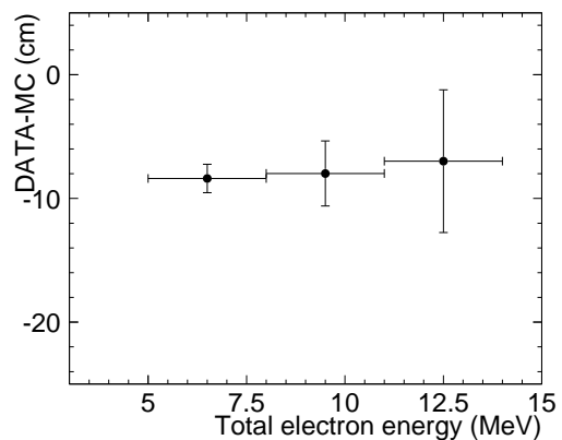
FIG. 22: The vertex shift as a function of energy. The markers show the amount of vertex shift measured by Ni calibration at x=15.2 m y=-0.7 m and z=12 m. For the vertical axis, negative values mean vertex shifts inward towards the center of the detector.
