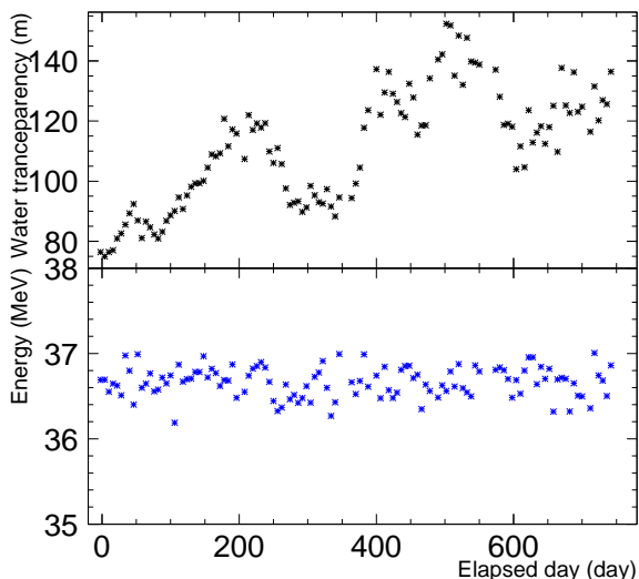
FIG. 14: The upper figure shows the time variation of the measured water transparency (weighted by the Cherenkov spectrum) during SK-III. The lower figure shows the stability of the peak energy of decay electrons in SK-III as a function of time.
