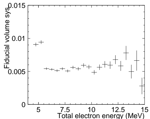
FIG. 23: The systematic uncertainty of the fiducial volume as a function of energy.
