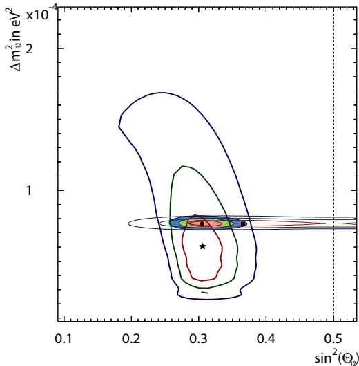
FIG. 32: Allowed region in solar parameter space (\theta_{12}, \Delta m^2) obtained by the three-flavor analysis. The thick lines and the star mark show the allowed regions and the best fit point of the global solar analysis. The thin lines and the square mark show the allowed regions and the best fit point of our KamLAND analysis. The filled areas and the filled point mark show the allowed regions and the best fit point of the combined analysis. For all regions, the innermost area (red), the middle area (green) and the outermost area (blue) show 68.3, 95, 99.7 % C.L. respectively.
