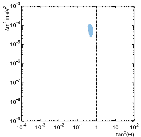
FIG. 28: 95% C.L. allowed region from SK-I,II,III combined analysis. The {}^8\text{B} flux is constrained by the SNO NC rate (LETA and phase-III).
