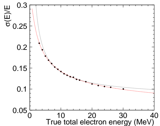
FIG. 7: Energy resolution function obtained by electron MC simulation. Black points show one standard deviation for a Gaussian fit of the MC simulation divided by the true total electron energy, while the red (dashed) line shows a fit to a polynomial function. The black (dotted) line shows SK-I energy resolution.
