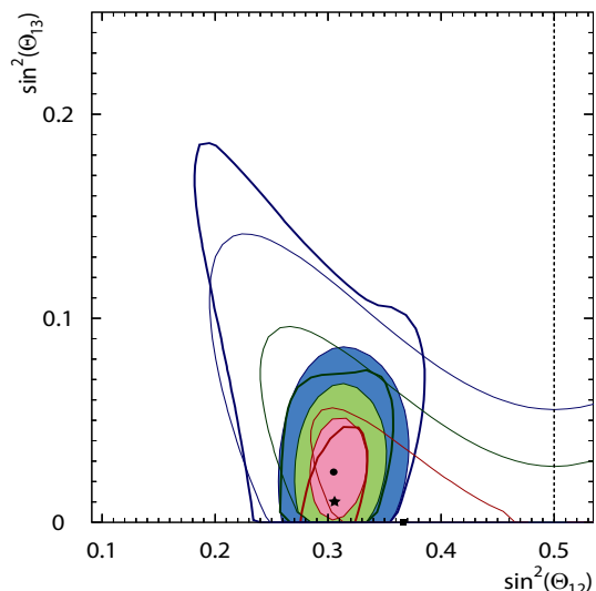
FIG. 33: Allowed region in (\theta_{12}, \theta_{13}) space obtained by the three-flavor analysis. The definitions of marks and lines are same as in Figure 32.
