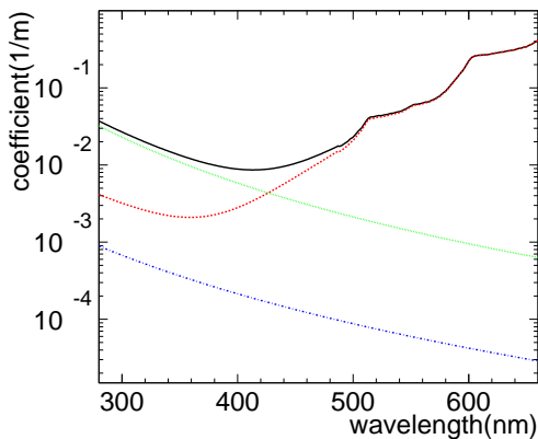
FIG. 13: Wavelength dependence of the water coefficients: scattering and absorption combined (black, solid), absorption (red, dashed), Rayleigh scattering (green, dotted) and Mie scattering (blue, dashed-dotted). The absorption coefficient is a function of water transparency and the water transparency in this graph is 139 m.
