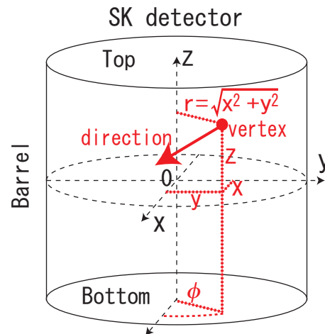
FIG. 3: Definition of detector coordinate system.
