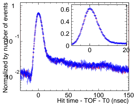
FIG. 16: Timing distribution of each hit PMT after tuning the MC simulation, for LINAC 5.1 MeV (x,z)=(-4\text{ m},0\text{ m}) data. The blue histogram with open circles shows data and the red dashed histogram shows MC simulation.
