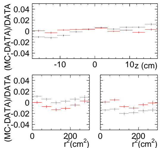
FIG. 15: Hit rate difference, (MC-DATA)/DATA, for barrel (upper), top (left lower), and bottom (right lower). Black (dashed) shows \beta=0 . Red (solid) shows the hit rate difference with tuned \beta . This calibration data was taken in Feb. 2008, the same period as the LINAC calibration.
