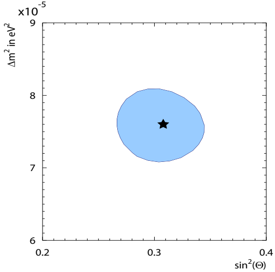
FIG. 30: Allowed region for all solar experiments and KamLAND for two-flavor analysis at 95% C.L..
