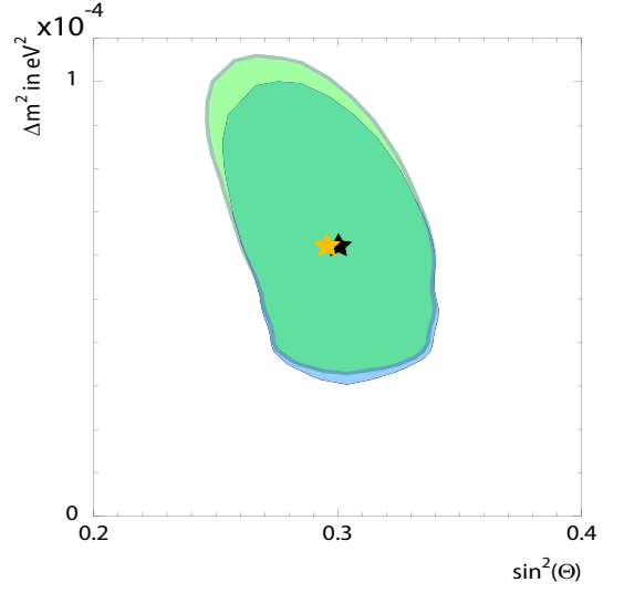
FIG. 31: Allowed region for all solar experiments for two-flavor analysis at 95% C.L.. The light green contour and the yellow star show the result without SK-III, and the light blue contour and the black star show the result with SK-III, which is same as Figure 29.
