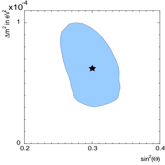
FIG. 29: Allowed region for all solar experiments at 95% C.L..
