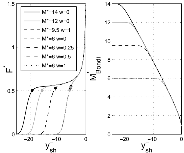
Figure 11. F^* (left) and M_{\text{Bondi}}^* (right) plotted against y_{\text{sh}}^- , for various incoming matter profiles ( w and M_{\text{ADM}} values), including several shell ( w = 0 ) cases. The time when the dynamical horizon first forms is marked on each flux curve (which is later for larger w ). All the curves with the same M_{\text{ADM}} (6 in this example) are on top of each other and cannot be distinguished by the eye, showing that they have the same universal behavior throughout the evolution, including the early times. More generally all the asymptotic physical quantities depend only on the combination M_{\text{ADM}} of the profile parameters M and w as long as \kappa w is small compared to the initial area of the GDH.
