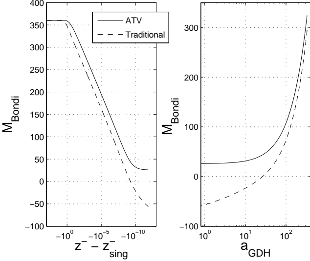
Figure 5. The ATV Bondi mass M_{\text{Bondi}}^{\text{ATV}} (solid lines) and the traditional Bondi mass M_{\text{Bondi}}^{\text{Trad}} (dashed lines) are plotted against z^- - z^-_{\text{sing}} (left) and the horizon area (right). This simulation corresponds to M_{\text{ADM}} = 360 , N = 720 (so M^* = 12 ). For high values of N , both formulas give a large non-zero Bondi mass at the last ray. M_{\text{Bondi}}^{\text{Trad}} becomes negative when the area is still macroscopic. On the other hand M_{\text{Bondi}}^{\text{ATV}} remains strictly positive all the way to the last ray, where the generalized dynamical horizon (GDH) shrinks to zero area.
