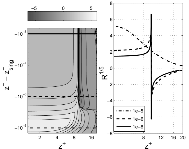
Figure 3. The Ricci scalar R for M^* = 8 . Left: 2D contour plot of R^{1/5} showing the increase in R as the singularity (dark vertical region near the middle) is approached and the asymptotically flat region ( R \rightarrow 0 ) near \mathcal{I}_R^+ ( z^+ \rightarrow \infty ). Right: R^{1/5} as a function of z^+ on the lines z^- - z_{\text{sing}}^- = -10^{-5}, -10^{-6}, -10^{-8} (marked on the left panel as horizontal lines), showing a double peak, indicating the divergent behavior of \partial_+ \partial_- \Phi at the singularity. The fact that the peak is narrow rules out a strong thunderbolt singularity. Note that the dark color at the region of the singularity is due to the high density of contour lines, and not directly due to negative values of R . While naive numerical calculation of R very close to \mathcal{I}_R^+ does not yield reliable results due to catastrophic cancellation, it is already very small in the high z^+ values shown here, and the trend towards 0 is clear.
