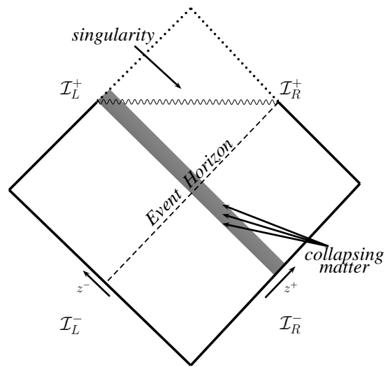
Figure 1. Penrose diagram of the CGHS black hole formed by the gravitational collapse of a left moving field f_+ . The physical space-time is that part of the fiducial Minkowski space which is to the past of the space-like singularity.
