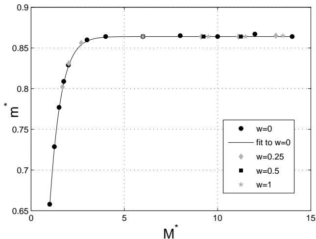
Figure 10. The value of m^* (i.e. M_{\text{Bondi}}^{\text{ATV}}/\bar{N} at the last ray) plotted against M^* (which equals M_{\text{ADM}}/\bar{N} ) for M^* \geq 1 . In addition to points corresponding to shell collapse ( w = 0 ) the plot now includes points with more general profiles with w = 0.25, 0.5, 1 . The universal value m^* \approx 0.864 persists for M^* \geq 4 .
