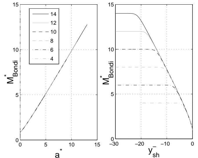
Figure 9. M_{\text{Bondi}}^* = (M_{\text{Bondi}}^{\text{ATV}}/\bar{N}) is plotted against the horizon area \mathbf{a}^* := (\mathbf{a}_{\text{GDH}}/\bar{N}) (left) and y_{\text{sh}}^- (right) for values of M^* from 4 to 14. For all these macroscopic M^* , M_{\text{Bondi}}^* starts at the value of M_{\text{ADM}} in the distant past ( \kappa y_{\text{sh}}^- \ll -1 ), and then joins a universal curve of M_{\text{Bondi}}^* . When the dynamical horizon first forms M_{\text{Bondi}}^* is quite close to its initial value of M^* . (This is difficult to see in the left plot where all the curves crowd.) This means that almost all of the evaporation occurs after the formation of the dynamical horizon.
