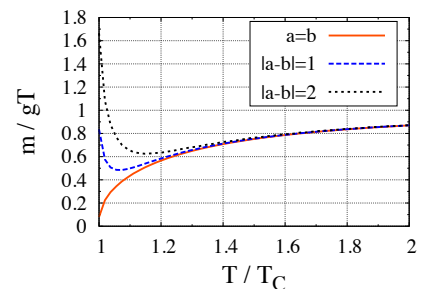
FIG. 4: Gluon masses, m_{ab}/(gT) , for SU(3) pure gauge theory: diagonal gluons, with a = b , are light; while there are two off diagonal gluons with heavy masses, for |a - b| = 1 and |a - b| = 2 .
