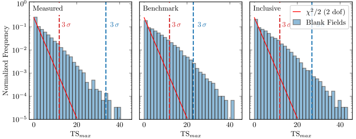
FIG. 2. TS distribution for combined blank fields corresponding to each of our sub samples. For reference, we show the distribution of \chi^2/2 with two degrees of freedom, as well as vertical lines comparing the TS value corresponding to 3\sigma for the Chernoff's theorem approach (red-dashed) vs the empirical method used in this analysis (blue-dashed) for a given subsample.
