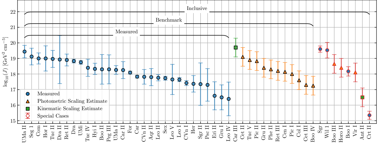
FIG. 1. J -factors and uncertainties for all 50 dSphs considered in this work. Marker shapes and colors indicate whether the J -factor is determined by measurement (blue circles), the kinematic scaling relation of Equation 3 (green squares), or the photometric scaling relation of Equation 4 (orange triangles). The special cases are outlined in red. Also indicated in this figure are the different subsets into which each dSph falls.
