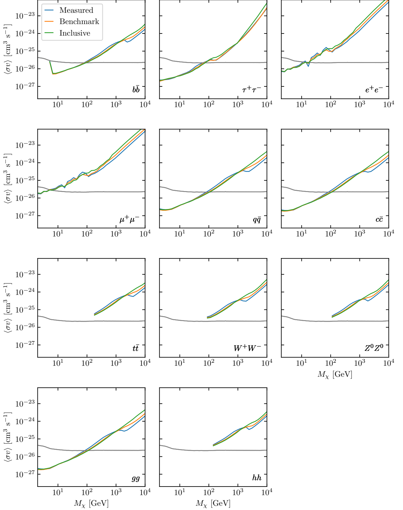
FIG. 8. Constraints on the \langle \sigma v \rangle - M_\chi parameter space for an expanded selection of DM annihilation channels for each of the samples considered in this work. The grey horizontal line is the thermal relic cross-section from [54].
