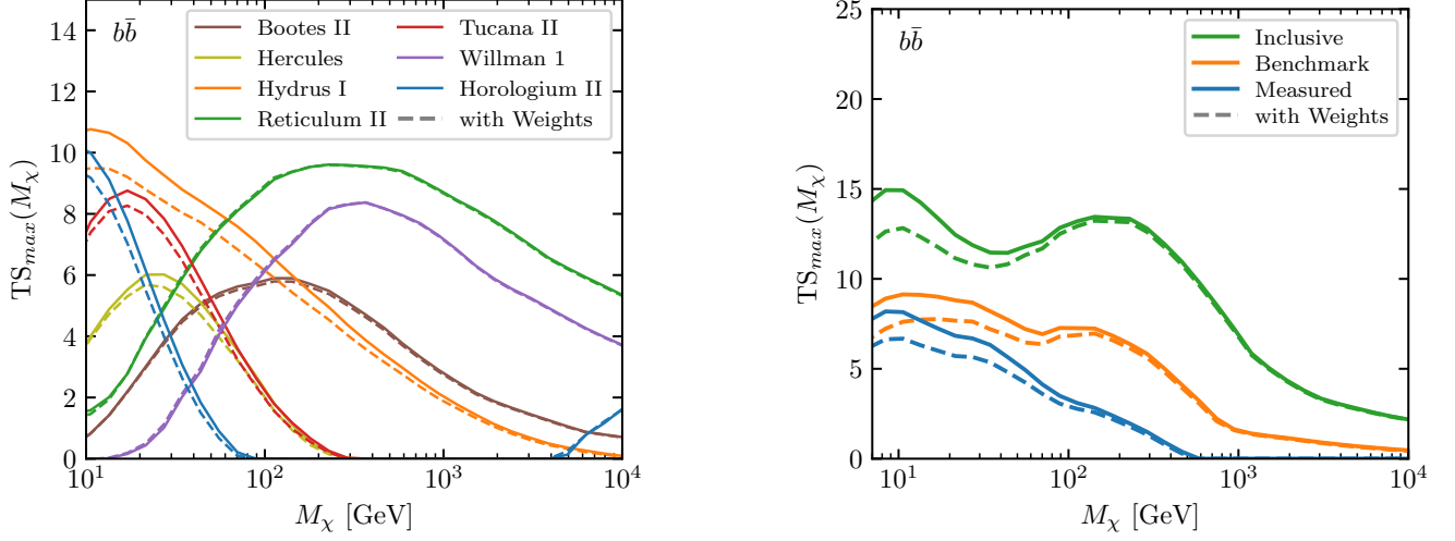
FIG. 9. TS vs M_\chi for the standard likelihood analysis (solid lines) and the weighted likelihood analysis (dashed lines) for the individual high TS dSphs ( left ), and the combined dSph samples ( right ).
