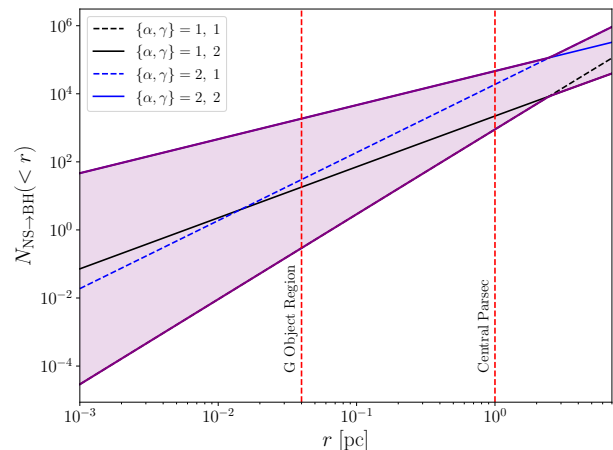
FIG. 1. The expected number of NS converted into black holes within a volume of radius r . The purple shaded region encapsulates varying \{\alpha, \gamma\} between 1 and 2 for each parameter individually. Here we assumed that M_{\text{PBH}} = 10^{21} g .
