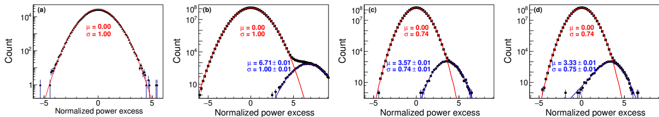
FIG. 3: Triangles in (a) show the normalized power excess distribution of the normalized grand power spectrum from the CAPP-12TB data after applying a frequency-independent scale factor of 0.74. (b), (c), and (d) show the normalized power excess distributions of 10 000 normalized grand power spectra from the 10 000 simulated CAPP-12TB experiments. Rectangles in (b), (c), and (d) are from all frequencies of the normalized grand spectra, while the circles there are from the frequency with the simulated axion signals. (b) and (c) were obtained without a filtering procedure, while (d) was obtained with filtering. (b) was obtained after background subtraction with a perfect fit, while (c) and (d) were obtained with our SG filter with d = 4 and W = 37 . Lines are a Gaussian fit resulting in \mu (mean) and \sigma (width), except for the Crystal Ball line shape [27] fit to the circle distribution in (d).
