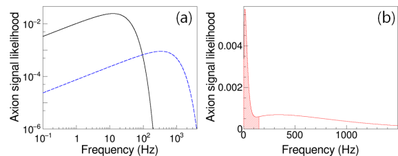
FIG. 1: Axion signal shapes for a corresponding frequency of 1.1 GHz following the SHM (blue dashed line in (a)) and the Sagittarius tidal stream model (black solid line in (a)). Red solid line in (b) is the dark matter shape considered in this work assuming axion dark matter makes up 100% of the local dark matter density, where the Sagittarius tidal stream model and the SHM contribute 23 and 77%, respectively, and only the red hatched region corresponds to the signal model.
