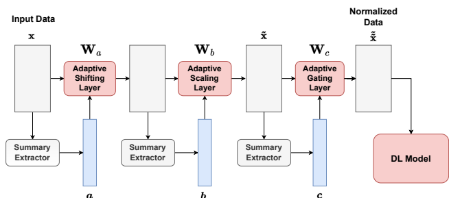
FIG. 2. Deep Adaptive Normalization (DAIN) is applied before feeding the data to the employed DL model. DAIN involves three adaptive normalization steps, i.e., adaptive shifting, adaptive scaling and adaptive gating, increasing the ability of DL models to handle non-stationary data.
