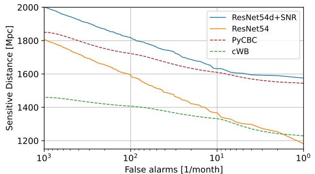
FIG. 10. Sensitive distance vs. false alarm rate for our best model (ResNet54d+SNR), in comparison with the simpler setup (ResNet54) used in [32] and two widely used algorithms for GW detection, Coherent WaveBurst (cWB) and PyCBC (the latter using aligned-spin templates only, see text for details). All codes were run on the same test dataset established in [32]. Our best model surpasses the performance of the other algorithms at all FAR in this setting (notice that the PyCBC run was based on a template bank with only aligned-spin waveforms).
