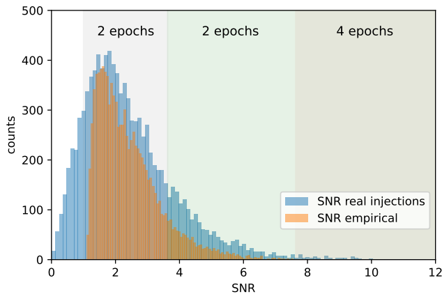
FIG. 4. Comparison of the SNR histogram computed with the empirical relation Eq. (13) to the optimal SNR of the injections (using a random subset of 10000 injections). A similar distribution is obtained. The shaded areas correspond to the restricted values of the SNR used in the first eight epochs of the learning strategy (from right to left, see Table II).
