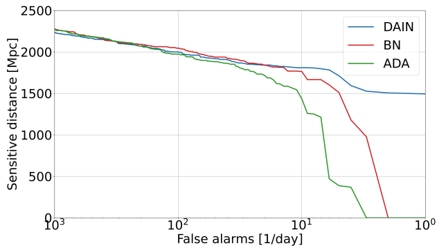
FIG. 9. Sensitive distance vs. false alarm rate for three different input normalizations: DAIN [34], Batch Normalization (BN) [39] and Adaptive Batch Normalization (ADA) [50] (for a shorter test dataset of duration of one day). In contrast to BN and ADA, DAIN maintains a good sensitive distance down to the lowest FAR.
