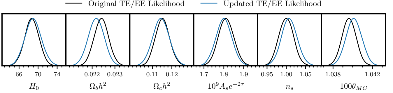
FIG. 13. Marginalized posterior distributions for core \Lambda CDM and H_0 from the original (black) and updated (blue) SPT-3G 2018 TE/EE likelihood. The posteriors widen slightly; the largest change is a 15% correction to the \Omega_c h^2 uncertainty. The shift to the central values of parameter constraints are less than the size of the new error bars.
