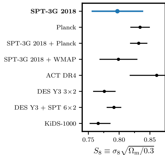
FIG. 11. Top panel: Constraints in the \sigma_8 vs. \Omega_m plane from SPT-3G 2018 (red), Planck (black line), a joint analysis of DES Y3 galaxy position and lensing data and SPT and Planck CMB lensing data ( 6 \times 2 , blue) [54], and DES Y3 joint galaxy density and weak lensing data ( 3 \times 2 , gray) [52]. The combined structure growth parameter, S_8 \equiv \sigma_8 \sqrt{\Omega_m}/0.3 , varies perpendicular to the degeneracy direction of the DES data.
