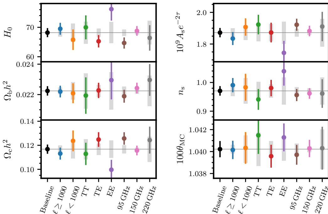
FIG. 3. Parameter constraints from the full SPT-3G 2018 TT/TE/EE data set (black points) and select subsets (coloured points as indicated) in \Lambda CDM. The grey boxes indicate the expected 1\sigma fluctuations between each subset and the full data set, taking the shared data into account. The observed shifts between subsets and the full data are consistent with statistical fluctuations. During the blind stage of this analysis, the parameter values along the vertical axes were not shown.
