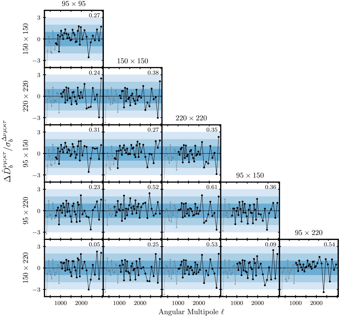
FIG. 14. Relative TT difference spectra as indicated by the row and column labels, i.e. difference spectra \Delta\hat{D}_b^{\nu\mu;\kappa\tau} divided by the square root of the associated covariance, \sigma_b^{\Delta\nu\mu;\kappa\tau} . The blue shading indicates the range of 1 - 3\sigma fluctuations, while gray indicates data excluded in the analysis. We conservatively exclude all TT data at \ell < 750 ; this is motivated by the shape of the transfer function, which slowly rises and plateaus at \ell \approx 750 ; the common-mode filter removes TT power on large and intermediate angular scales. We further exclude 150 \times 220 GHz and 220 \times 220 GHz TT spectra at \ell < 1000 , based on our model for correlated atmospheric noise. The PTE values are indicated in the top right corner of each panel. All PTE values are in the 95th percentile and the multifrequency spectra are in good agreement with one another.
