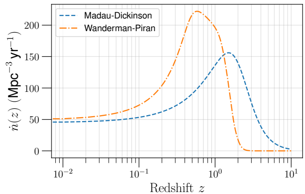
Figure 14. The merger rate density as a function of redshift for the Madau-Dickinson model with P(t_d) \propto 1/t_d and the Wanderman-Piran model using the log-normal delay time distribution. Both the distributions have been normalized such that the local merger rate ( \dot{n}(0) ) is equal to 45 \text{ Gpc}^{-3} \text{ yr}^{-1} .
