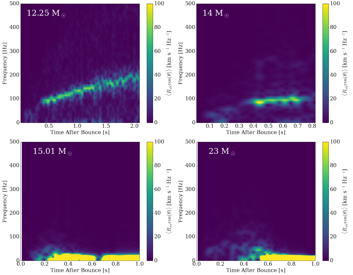
FIG. 9. In this figure, we show the spectrogram of the z-component of shock dipole position for four models. Note the focus on lower frequencies. In the non-exploding 12.25- and 14- M_{\odot} models, the spiral-SASI modes are clearly seen and manifest gradually increasing frequencies as the PNS core shrinks. The exploding models (for example, the 15.01 and 23 M_{\odot} models depicted here) don't show this feature, but do manifest the even lower frequency signals due to the matter memory caused by explosion anisotropy (see also Figure 8). We note that the 23- M_{\odot} model may show a weak SASI signature (analogous with that found in the 25- M_{\odot} model in reference [72]) that vanishes at \sim 0.55 seconds and is perhaps indicative of its delayed explosion time. The onset of explosion corresponds with the rise of the low-frequency signal memory in the bright yellow band.
