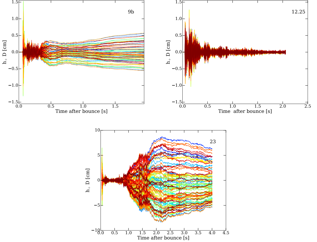
FIG. 13. The gravitational-wave strain h_+ D (cm) as a function of time after bounce (in seconds) for the 9b model, the non-exploding model 12.25-M_\odot , and model 23-M_\odot for various, arbitrary, viewing angles illustrated by color. These plots do not include the neutrino memory (§II F). Note the large anisotropy by viewing angle, which is dominated at late times by the matter memory, which is sourced by the large-scale explosion asymmetry. In the black hole model ( 12.25-M_\odot ), we see no memory, and little anisotropy, at late times. Though we show only the + polarization, the results are consistent for both polarizations. We see that in principle some measure of the degree and angle of the matter explosion asymmetry can be discerned by the sign and magnitude of this memory. However, the neutrino memory, if only weakly correlated with the matter memory, will complicate the extraction of such a feature. Nevertheless, the difference in the frequency spectra of the matter and neutrino memories generically, with the former at a higher average frequency, may allow one someday to disentangle the two.
