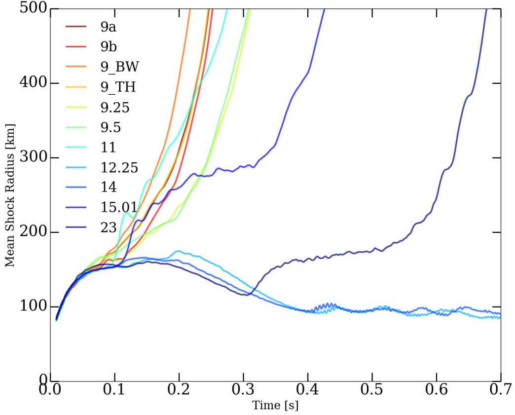
FIG. 2. Early post-bounce behavior of the mean shock radii (in km) for all the models as a function of time (in seconds after core bounce). All models explode except for the 12.25- and 14- M_{\odot} progenitors, which show evidence for a spiral SASI after \sim 400 and \sim 300 ms post-bounce, respectively, in the form of \sim 10 ms oscillations in the shock radii. Note that the 12.25- and 14- M_{\odot} (non-exploding) progenitors also shows a secular \sim 70 ms oscillation in the shock radii.
