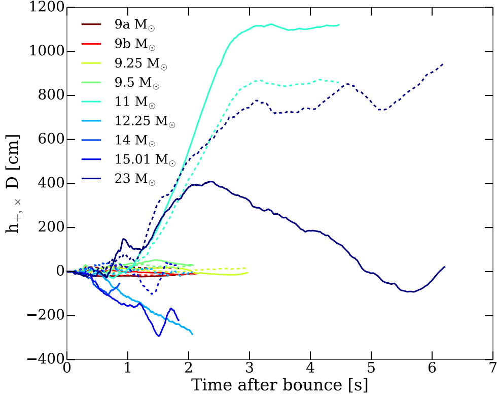
FIG. 14. Same as Figure 3, but for the gravitational-wave memory due to neutrino emission anisotropy. Because of the cumulative nature of the neutrino GW memory, the strain is both larger and shows less variation on small timescales when compared to the matter-driven strain. We reach strains as high as 1000 cm for the 11- and 23- M_{\odot} models. Note that this is consistent with earlier work [92] showing continued growth with time of the memory strain. The strain growth rate also accelerates, showing upwards of 600 cm growth from \sim 2 to \sim 3 seconds for the 11- M_{\odot} progenitor. This emphasizes our essential point that models should be carried out to late times to fully capture not only the explosion dynamics, but the emerging GW signatures. The 11- M_{\odot} progenitor has the highest neutrino memory strain among those models we present in this paper. Otherwise, we see a general correlation with mass, with the low-mass progenitors having the smallest neutrino memory. The non-exploding 12.25- and 14- M_{\odot} models show significant evolution and magnitude in their memory signatures.
