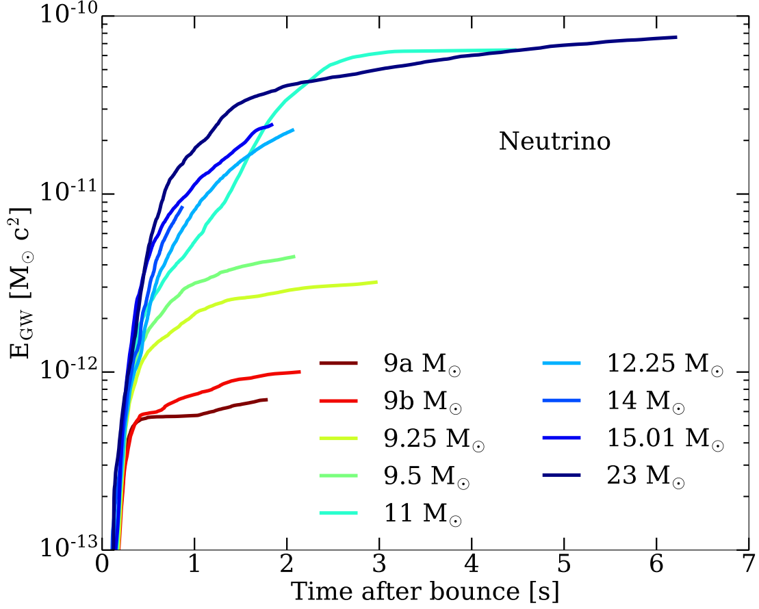
FIG. 15. Same as Figure 10, but for the radiated gravitational-wave energy due to the neutrino anisotropy. As seen in Figure 14, unlike the matter contribution, the neutrino anisotropy continues to contribute to the gravitational signal past six seconds (for our longest simulation), emphasizing the presence of sustained neutrino emission asymmetry. We see again at least two orders of magnitude of growth with time after \sim 50 ms in the associated GW energy, this time in the neutrino memory component. The 23- M_{\odot} progenitor has neutrino GW memory energies only slightly higher than the matter GW components for the least energetic, lowest-mass progenitors. Importantly, for the same progenitor model, the late time neutrino-sourced GW energies, albeit still growing, are more than two orders of magnitude smaller than the corresponding matter components.
