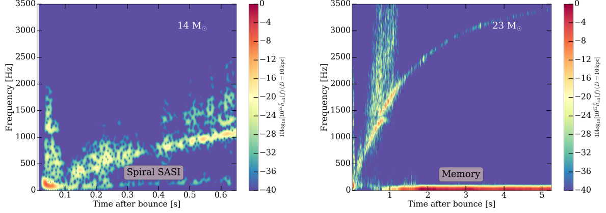
FIG. 8. Plots of the effective strains as a function of time after bounce (in seconds) for two representative 3D models (the black-hole former 14\text{-}M_{\odot} and late-exploding 23\text{-}M_{\odot} model). Note that we see a dark red band at low ( \leq 50 Hz) frequencies for the exploding model associated with the asymmetric ejecta at later times (matter “memory”). The non-exploding model shows a spiral SASI signature at \sim 100 Hz. This quasi-periodic feature is also seen after \sim 0.4 seconds in Figure 2 for both the 14\text{-}M_{\odot} and 12.25\text{-}M_{\odot} black-hole formers. Such a feature shows up only for non-exploding models when the shock radius has shrunken below \sim 100 km. These features are much less prominent in the gravitational-wave energy spectra because they are low-frequency, and, hence, low-power components. There may be a hint of the SASI itself in the lower left-hand corner of the panel to the right. See text in §II A for a discussion.
