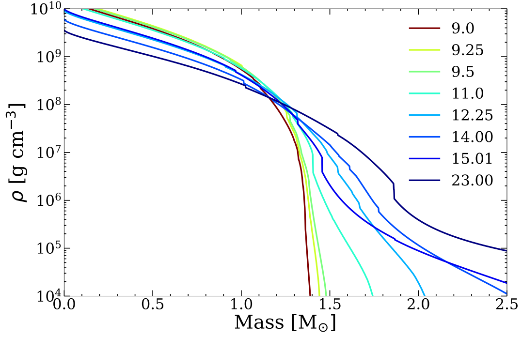
FIG. 1. Mass density profiles for the various progenitors studied here, from 9.0 (reddish) to 23 (blue) M_\odot . The accretion of the Si/O interface frequently corresponds with the onset of shock revival. Note that the 12.25- and 14- M_\odot models do not explode and are destined to produce a stellar-mass black hole.
