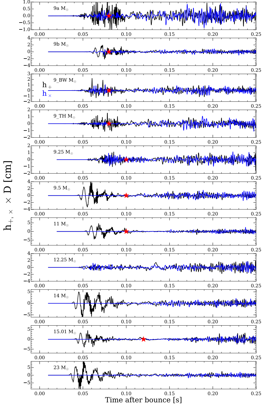
FIG. 4. Same as Figure 3, but now focusing on the matter strain during the first 250 ms after core bounce to illustrate the prompt convection. Note the stately oscillation present in most models of \sim 10 ms periods visible in the + polarization and absent in the \times polarization. This is a generic feature indicative of the strain polarization geometry. Note that only model 9a has any perturbations on bounce.
