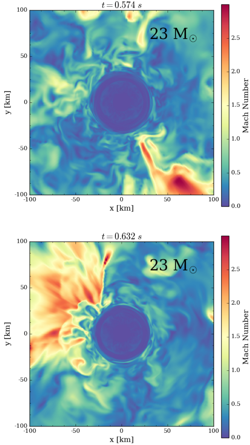
FIG. 7. Plots (2D slices of 3D data) of the Mach number distribution in the inner 100 kilometers of the 23- M_{\odot} simulation at 574 and 632 milliseconds after bounce. Seen are representative supersonic plumes crashing onto the PNS core. Such plumes not only excite the GW emission, but themselves emit a component of the GW signal. See text in §II A for a discussion.
