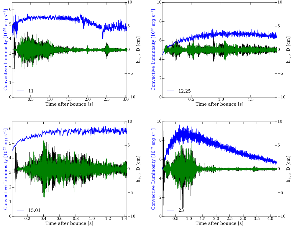
FIG. 19. Same as Figure 18, but for models 11-, 12.25-, 15.01-, and 23- M_{\odot} .
