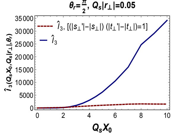
FIG. 2. The origin of the rapid growth for \hat{I}_3 . The solid line shows the full result; the dashed line shows the result without the secular growth factors.
