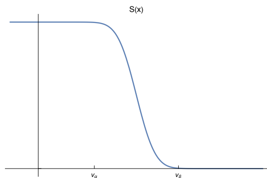
Figure 10. The interpolating function S(x) defined in eq. (56)
