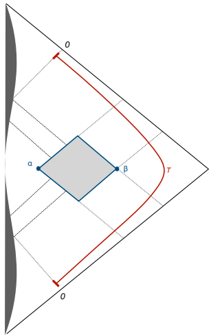
Figure 6. In red, the worldline of an observer moving at a constant distance R \gg 2m .
