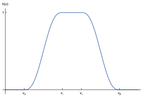
Figure 9. The interpolating function h(v) defined in Footnote 1.
