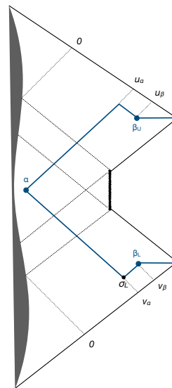
Figure 4. The blue line is the boundary of the region that is excised, because it is not a good approximation of the spacetime of a physical black hole. The two horizontal portions of the blue line are identified; the excised region is replaced by a non-singular geometry.
