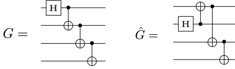
FIG. 8. Two GHZ state preparation circuits.
