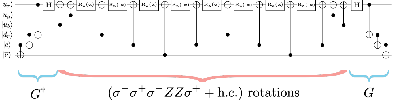
FIG. 9. A quantum circuit that provides the time evolution associated with the \sigma_{\bar{\nu}}^- \sigma_e^+ \sigma_{d,r}^- Z_{u,b} Z_{u,g} \sigma_{u,r}^+ operator in the \beta -decay Hamiltonian, with \alpha = \sqrt{2}Gt/8 .
