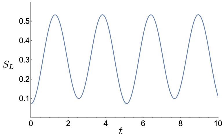
FIG. 5. The linear entanglement entropy, S_L , between quarks and antiquarks plus leptons during the \beta -decay of an initial \Delta^- -baryon.
