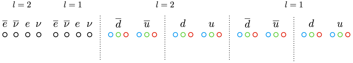
FIG. 10. A qubit layout which is efficient for the simulation of \beta -decay. Shown is an example for L = 2 .
