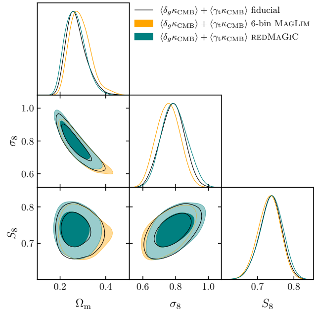
FIG. 8. Fiducial constraints on cosmological parameters \Omega_m , \sigma_8 , and S_8 using the \langle\delta_g\kappa_{\text{CMB}}\rangle + \langle\gamma_t\kappa_{\text{CMB}}\rangle probes compared with using the REDMAGIC lens sample instead of the MAGLIM lens sample.
