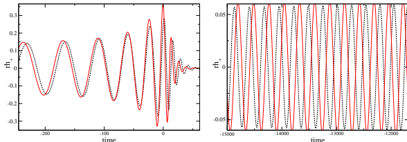
FIG. 1: Comparison of NR results (dashed-black curve) for gravitational wave amplitude, and “naively” rescaled PP results (solid-red curve) for q = 3 . The rescaling is a reduction of both the time and the gravitational wave strength rh_+ by the factor of 1/(1 + 1/q) = 0.75 . The curves are aligned so that the peaks of both the NR and PP runs agree.
