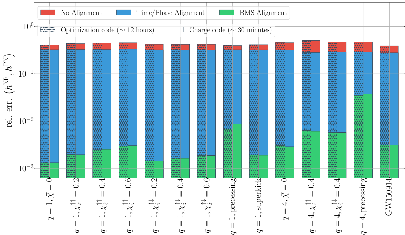
Errors before and after mapping to PN BMS frame
