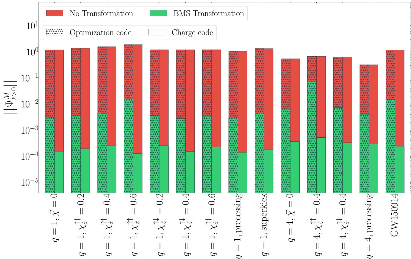
Errors before and after mapping to superrest frame
