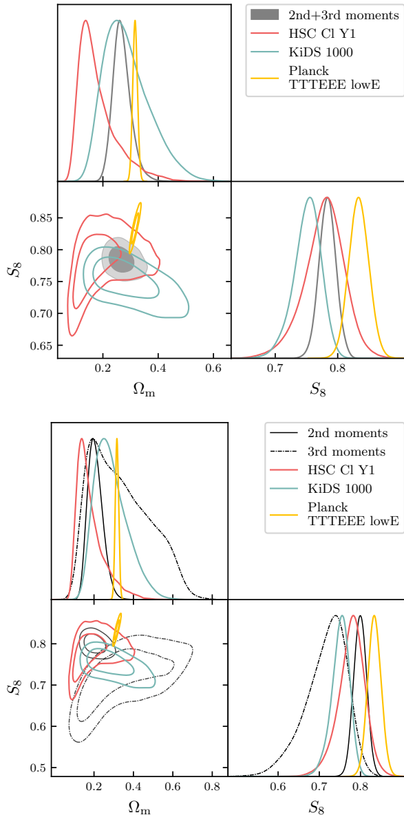
Figure 8. Posterior distributions of the cosmological parameters \Omega_m and S_8 , for the moments analysis and for the recent results of the KIDS-1000 survey [6], HSC [52], and Planck [2]. Table III shows the tension between the DES moments and other analyses. The upper panel only shows the combination of second and third moments, whereas the lower panel shows second and third moments constraints individually.
