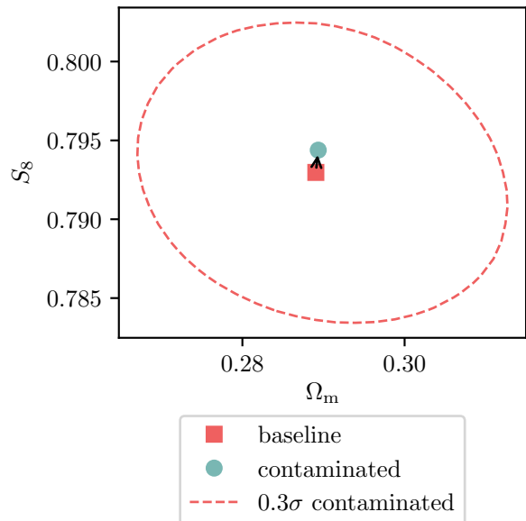
Figure 13. Parameter posteriors used to determine the level of PSF additive bias contamination. Constraints from the combination of second and third moments are shown. ‘Baseline’ refers to an analysis performed on a theory data vector, ‘contaminated’ refers to the analysis performed on a data vector contaminated by the impact of PSF additive biases (see Appendix C). The dashed lines demarcate the 0.3\sigma contours for the 2D marginalised constraints of the contaminated data vector; the filled square and circle show the peak of the posteriors.
