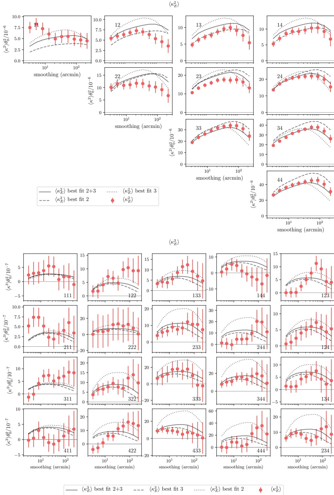
Figure 3. Measured second moments (upper plots) and third moments (lower plots). Red points represent the measurement. Grey shaded regions highlight the scales removed by the analysis. The conservative scale cut implemented in this analysis removes a large part of our data vector. Solid, dotted, and dashed lines represent the predictions obtained using the best-fitting cosmology of second and third moments analysis (either considered in combinations or alone). Data points are very correlated (Fig. 2), so we caution the reader from any \chi^2 -by-eye estimation.
