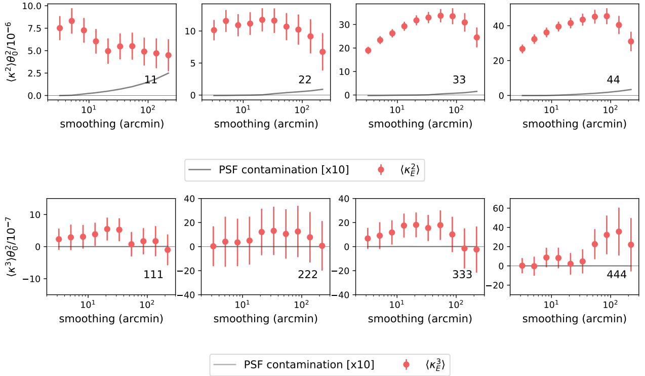
Figure 12. Contribution of PSF modelling errors to the second and third moments of the convergence fields. The contribution, estimated as explained in Appendix C, is shown as the black lines. Due to its small amplitude, the signal has been multiplied by a factor of 10. The red points represent the measured moments of the convergence field. We only show ‘auto’ moments here, although the pattern is very similar for all the other moments. Grey shaded regions highlight the scales removed by the scale cut used in the analysis.
