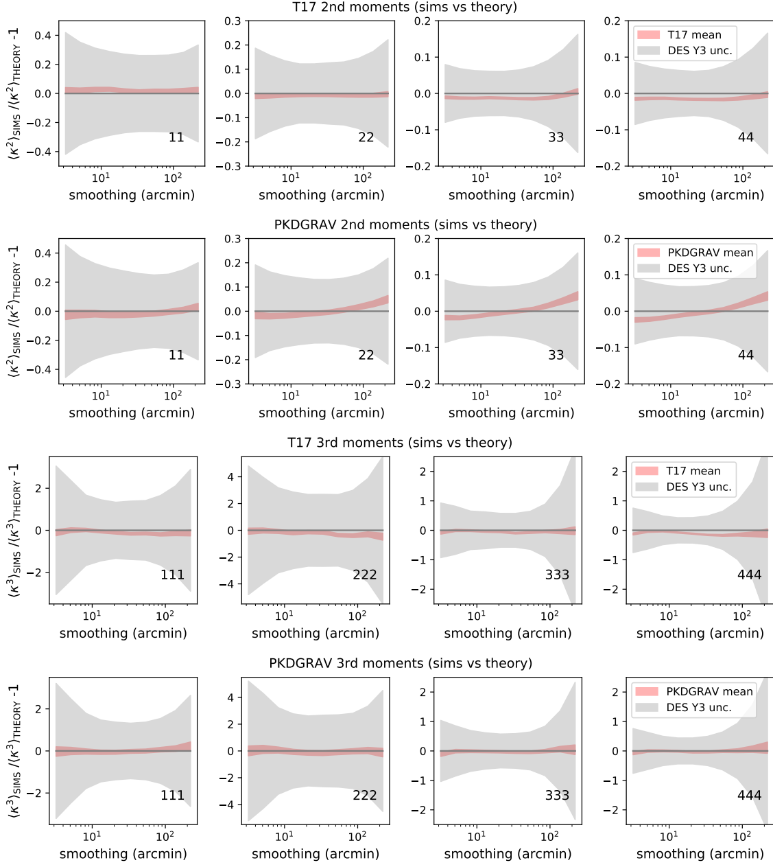
Figure 10. Comparison between theory predictions and moments as measured in N-body simulations. The red bands encompass the 68 percentile of the moments as measured on all the realisations from the T17 or PKDGRAV simulations. The grey bands represent the expected measurement uncertainty for one individual realisation, which represents the DES Y3 survey. No scale cut is applied here. Only ‘auto’ moments are shown. It is evident that the theoretical model agrees with N-body simulations to well within the statistical uncertainty of the survey.
