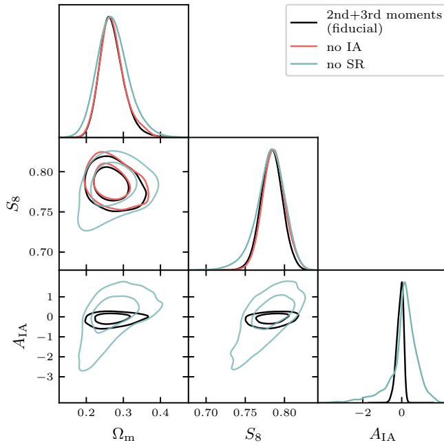
Figure 6. Posterior distributions of the cosmological parameters \Omega_m and S_8 , and the IA amplitude parameter A_{IA} , for the combination of second and third moments. “SR” stands for shear ratio. The 2D marginalised contours in these figures show the 68 per cent and 95 per cent confidence levels.
