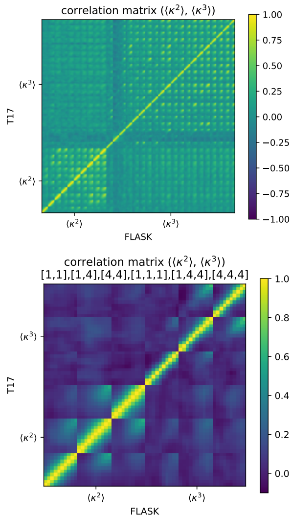
Figure 2. Top : measured correlation matrix of second and third moments from FLASK simulations (lower right triangle) and from T17 simulations (upper left triangle). No scale cut has been applied. From bottom left to top right, we show the bins: [1,1], [2,2], [3,3], [4,4], [1,2], [1,3], [1,4], [2,3], [2,4], [3,4], [1,1,1], [2,2,2], [3,3,3], [4,4,4], [2,1,1], [3,1,1], [3,2,2], [4,1,1], [4,2,2], [4,3,3], [1,2,2], [1,3,3], [1,4,4], [2,3,3], [2,4,4], [3,4,4], [1,2,3], [1,2,4], [1,3,4], [2,3,4]. The main difference between the two covariances is that the FLASK one has on average 5-10 per cent larger amplitude at large scales. The difference vanishes at small scales since those are dominated by shape noise. Bottom : same as the top image, but focusing on a few elements ( from bottom left to top right, we show [1,1], [1,4], [4,4] for second moments and [1,1,1], [1,4,4] and [4,4,4] for third moments), and showing only the dynamical range [-0.1,1.0] effectively spanned by the elements of the correlation matrix. The diagonal blocks of the correlation matrix contain essentially all the non-negligible contributions. On large scales, where the cosmic variance contribution to the covariance dominates, the window function of the moments generates off-diagonal terms (within the block diagonal matrix) while on small scales these are due to the pixel window function. Note that in the absence of shape noise we also expect a contribution from non-linear evolution on small scales. The third moments correlation matrices are more diagonal than second moments ones owing to a larger shape noise contribution. Non-negligible cross-covariance between second and third moments is limited to very large scales, and is generally small (10-15 per cent at most).
