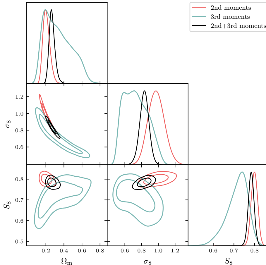
Figure 4. Posterior distributions of the cosmological parameters \Omega_m , \sigma_8 , and S_8 for the second moments, third moments, and the combination of second and third moments. We note that our fiducial analysis include small-scale galaxy-galaxy lensing ratios (a.k.a. shear ratios, §IV). The 2D marginalised contours in these figures show the 68 per cent and 95 per cent confidence levels.
