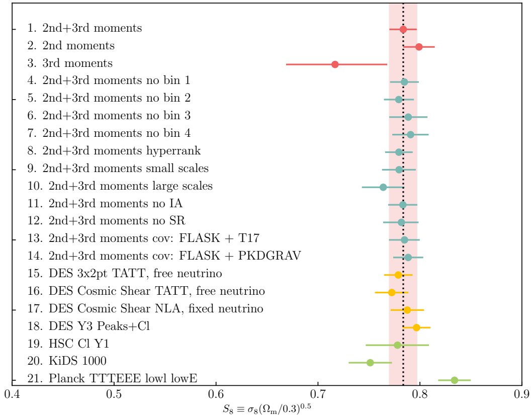
Figure 5. Constraints on the cosmological parameter S_8 ; we report the mean of the posterior and the 68 per cent confidence interval. The first three lines are the fiducial results from this analysis. Following that are the S_8 values for a number of variations and systematic tests: removing one redshift bin at a time, using a different parameterization for the redshift distribution called “hyperrank”, considering only small or large scales, considering the case with no intrinsic alignment or no shear ratio (SR), and using different covariance matrixes (FLASK + T17 or FLASK + PKDGRAV), as explained in Appendixes F and G. Lastly, we compare with a number of results from other works, either with DES or external data.
