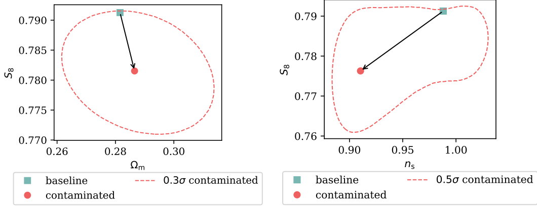
Figure 9. Parameter posteriors used to determine the scale cuts for the cosmological analysis. Constraints from the combination of second and third moments are shown. ‘Baseline’ refers to an analysis performed on a theory data vector, ‘Contaminated’ refers to the analysis performed on a data vector contaminated by the impact of baryonic feedback (see Appendix A). The dashed lines demarcate the 0.3\sigma or 0.5\sigma contours for the 2D marginalised constraints of the contaminated data vector; the filled square and circle show the peak of the posteriors for the Contaminated and Baseline data vectors, respectively.
