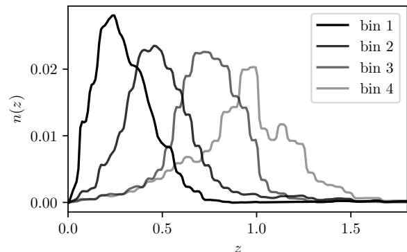
Figure 1. Redshift distributions as estimated in data for the four DES Y3 tomographic bins [75].
