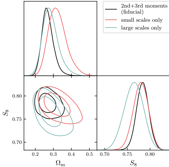
Figure 17. Posterior distributions of the cosmological parameters \Omega_m and S_8 for the combination of second and third moments. The 2D marginalised contours in these figures show the 68 per cent and 95 per cent confidence levels. The figure shows the posteriors obtained using only the small or the large scales of the data vector.
