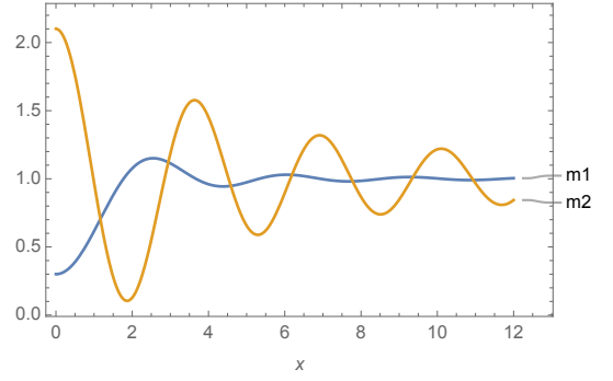
Figure 1: We plot m_1 = 1 + m_{EE}^\parallel/m_{EE}^{(0)} and m_2 = 1 + m_{EE}^\perp/m_{EE}^{(0)} as a function of the dimensionless x = a(|\nu| - \Omega) .
