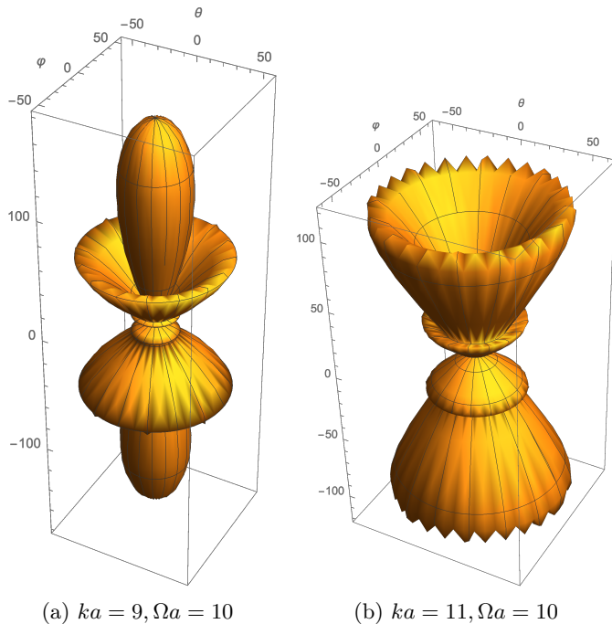
Figure 4: Total contribution to the emission probability p_1(ka, \Omega a, \theta) + p_2(ka, \Omega a, \theta) per unit of solid angle as a function of spherical angle \theta . We show two different values of ka at a fixed value of \Omega a = 10 .
