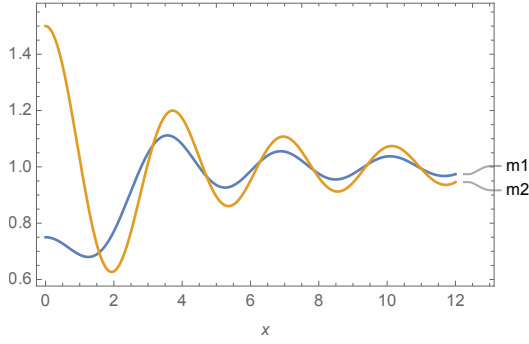
Figure 3: Ratios m_1 = 1 + m_{BB}^{\parallel}/m_{BB}^{(0)} and m_2 = 1 + m_{BB}^{\perp}/m_{BB}^{(0)} as a function of the dimensionless x = a(|\nu| - \Omega) .
