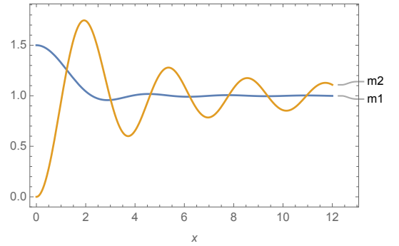
Figure 2: m_1 = 1 + m_{EB}^\parallel/m_{EB}^{(0)} and m_2 = 1 + m_{EB}^\perp/m_{EB}^{(0)} as a function of the dimensionless x = a(|\nu| - \Omega) .
