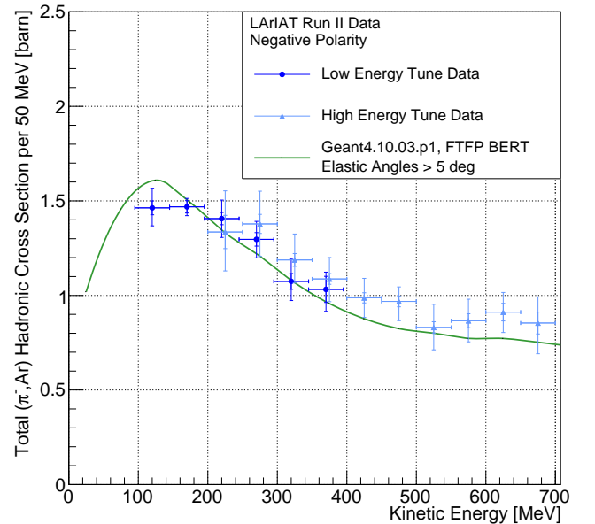
FIG. 15. (\pi^-, \text{Ar}) total hadronic cross section for scattering angles greater than 5 degrees measured in the LArIAT low energy and high energy tune Run II data samples. The Geant4 prediction for the total hadronic cross section for inelastic scattering and elastic scattering angles greater than 5 degrees is displayed in green.
