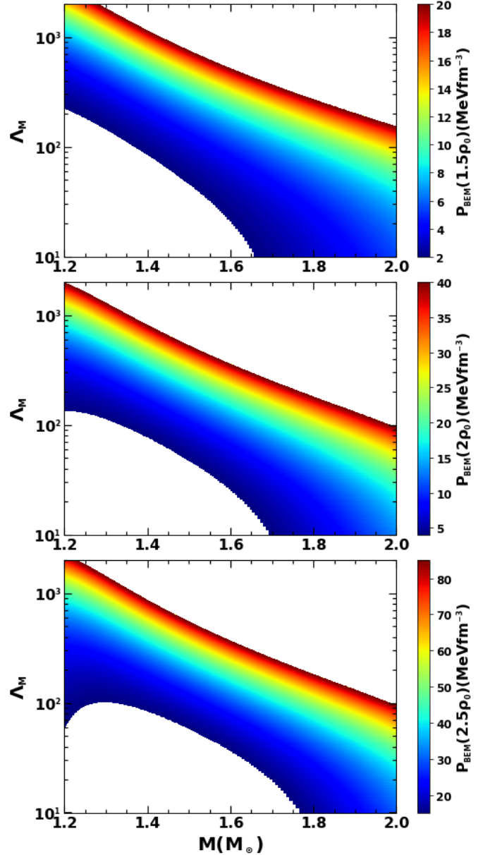
FIG. 8: The median values of pressure for \beta -equilibrated matter is shown here as a function of neutron star mass and its tidal deformability at densities 1.5\rho_0 (top), 2.0\rho_0 (middle) and 2.5\rho_0 (bottom).
