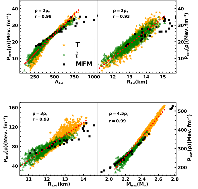
FIG. 6: The variations of pressure for \beta -equilibrated matter ( P_{\text{BEM}}(\rho) ) at selected densities versus tidal deformability \Lambda_{1.4} , radii R_{1.4} and R_{2.07} and maximum mass M_{\text{max}} of neutron star. The red dashed lines are obtained by linear regression (see Eq. (17) in section III D).
