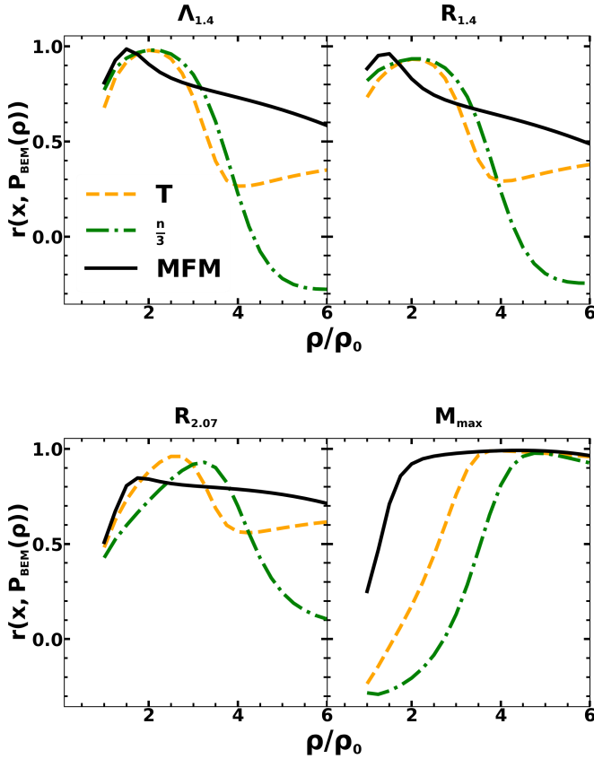
FIG. 5: The correlation coefficients r(x, P_{\text{BEM}}(\rho)) , as approximated by both Taylor and \frac{n}{3} expansion along with the mean-field theory calculations, is shown in this figure. Here, x represents either of the tidal deformability \Lambda_{1.4} , radii R_{1.4} , R_{2.07} , or maximum mass M_{\text{max}} of the neutron star, whereas, P_{\text{BEM}}(\rho) represents the pressure for \beta -equilibrated matter at a density \rho . The calculations are performed with neutron star properties obtained using marginalized posterior distributions of nuclear matter parameters in Taylor and \frac{n}{3} expansions. For the comparison the results are also displayed for a diverse set of non-relativistic and relativistic microscopic mean-field models (MFM).
