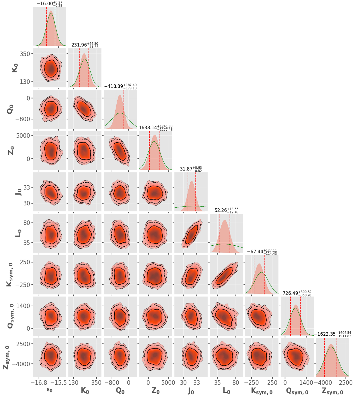
FIG. 2: Same as Fig. 1, but, for \frac{n}{3} expansions for the EoS of asymmetric nuclear matter.
