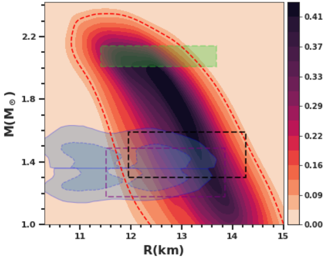
FIG. 4: Plot for joint probability distribution P(M, R) as a function of mass and radius of neutron star obtained for the \frac{n}{3} expansion. The red dashed line represents the 90% confidence interval. The outer and inner gray shaded regions indicate the 90% (solid) and 50% (dashed) confidence interval of the LIGO-Virgo analysis for BNS component from the GW170817 event [91–93]. The rectangular regions enclosed by dotted lines indicate the constraints from the millisecond pulsar PSR J0030+0451 (purple & black) NICER x-ray data [94, 95] and PSR J0740+6620 (green) [96]
