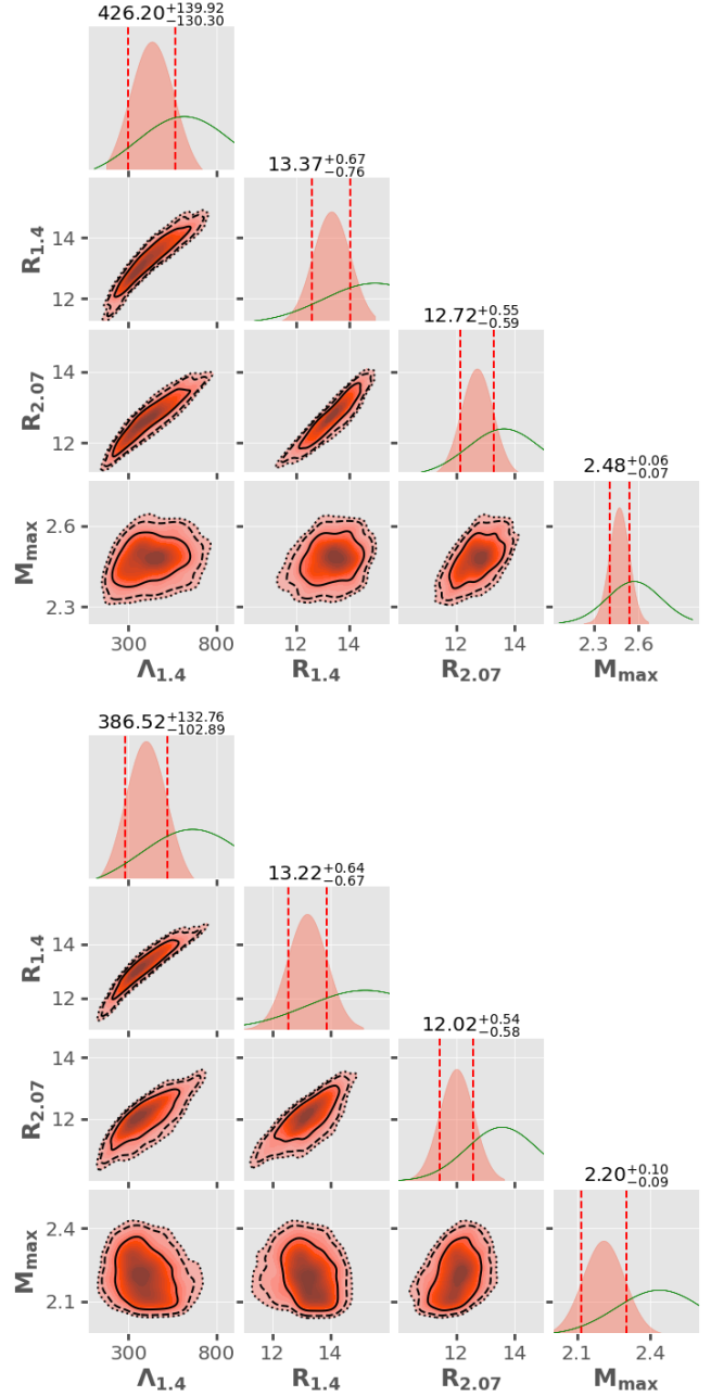
FIG. 3: Corner plots for the marginalized posterior distributions (salmon) of the tidal deformability \Lambda_{1.4} , radii R_{1.4} (km) and R_{2.07} (km) and the maximum mass M_{\text{max}} ( M_\odot ) for Taylor (top) and \frac{n}{3} (bottom) expansions. The green lines represent effective priors obtained using the priors for nuclear matter parameters (see also Table I).
