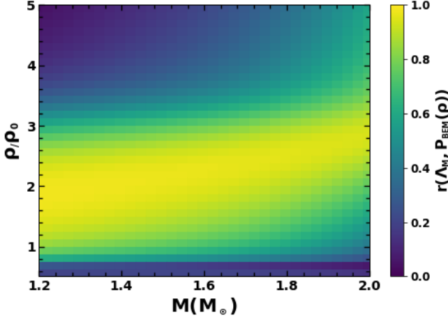
FIG. 7: Dependence of correlation coefficients between tidal deformability ( \Lambda_M ) and the pressure of \beta -equilibrated matter ( P_{\text{BEM}}(\rho) ) on neutron star mass ( M ) and density ( \rho ) is depicted in this plot. Here \rho_0=0.16 \text{ fm}^{-3} is used only for the scaling purpose.
