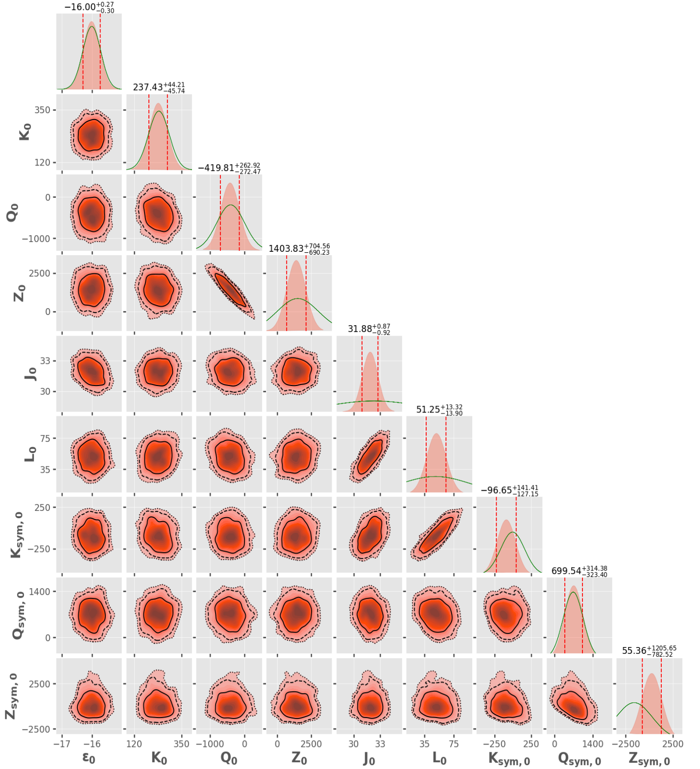
FIG. 1: Corner plots for the nuclear matter parameters (in MeV) obtained for Taylor expansions for the EoS of asymmetric nuclear matter. The one dimensional marginalized posterior distributions (salmon) and the prior distributions (green lines) are displayed along the diagonal plots. The vertical lines indicate 68% confidence interval of nuclear matter parameters. The confidence ellipses for two-dimensional posterior distributions are plotted with 1 \sigma , 2 \sigma and 3 \sigma confidence intervals along the off diagonal plots. The distributions of nuclear matter parameters are obtained by subjecting them to minimal constraints (see text for details).
