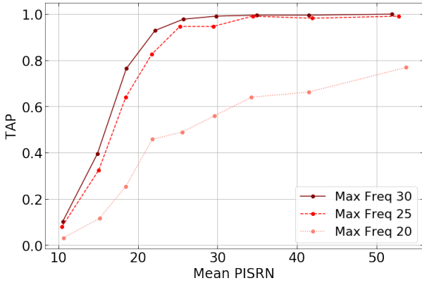
FIG. 5: The True Alarm Probability as a function of the PISNR for the O3 Gaussian noise case. Each curve represents a different test set with a different maximum frequency seen by the CNN.
