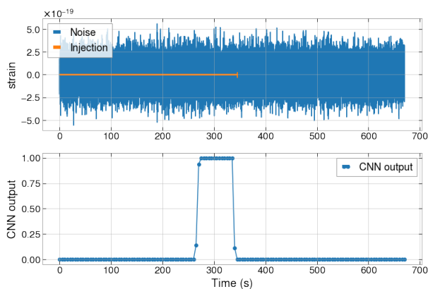
FIG. 8: Top: Representation of a signal and the noise it is injected in. Bottom: Representation of the output of the CNN. Each point represents the probability to have an inspiral in the 300 seconds of data. By convention, the time of a point represents the end of the time window. The network does not trigger on the early inspiral because the PISNR is too low. When it becomes high enough, the networks produces a trigger until the injection leaves the frame, giving multiple points with a high probability in a row.
