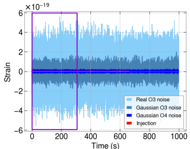
FIG. 3: Representation of the different types of noises for the Handford detector used together with an injection similar to GW170817, i.e. with neutron star masses of 1.46 and 1.27 M_{\odot} [79]. Note that only the part in the rectangle is passed to the network.
