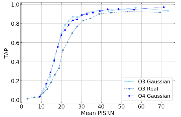
FIG. 6: The True Alarm Probability as a function of the PISNR for the O3 Gaussian noise, real O3 noise, and O4 Gaussian noise.
