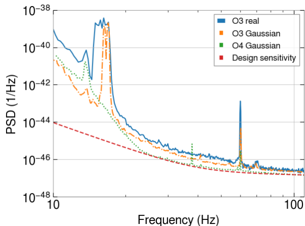
FIG. 2: Representation of the different PSDs, for the Livingston detector, used to generate the different data sets. We also show the design sensitivity PSD provided by PyCBC [71] used in [1].
