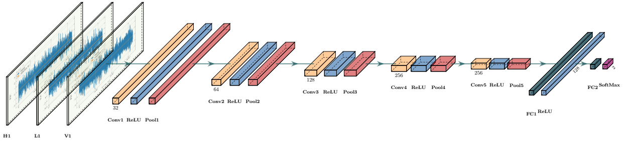
FIG. 4: Representation of the CNN architecture, the yellow layers are the convolutions, the blue ones are the ReLU activation, the red ones are the pool layers, the purple ones are the dense layers, and the dark purple is the final softmax layer. The number under each layer represents the number of channels.
