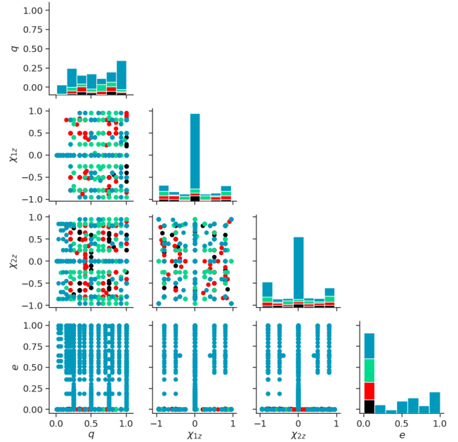
FIG. 5. Counting simulations in the (q, \chi_1, \chi_2, e) planes (faces of the 4-cube) for the 1320 nonprecessing binaries. The 120 release 1 simulations are black, the 154 release 2 simulations are red, the 203 release 3 are in green, and the 843 release 4 in blue.
