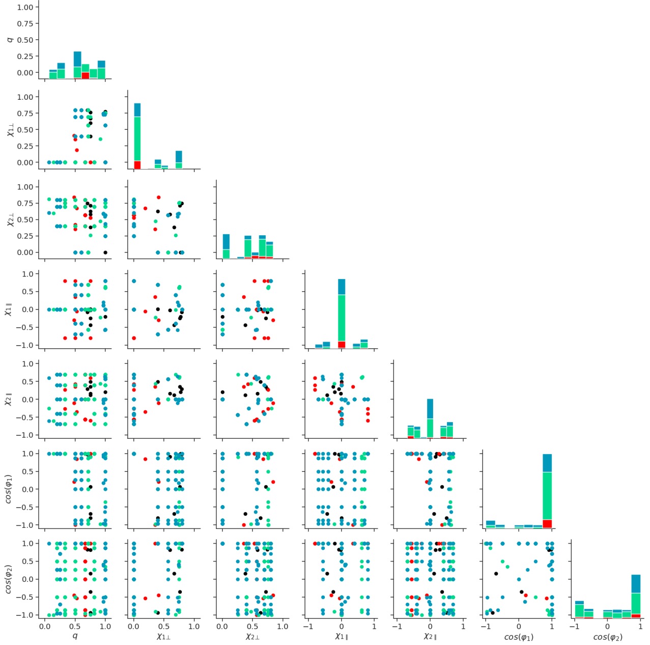
FIG. 8. Panels showing different combinations of the 7 binary parameters of the precessing parameter space ( q, \chi_{1\parallel}, \chi_{1\perp}, \varphi_1, \chi_{2\parallel}, \chi_{2\perp}, \varphi_2 ) for the 446 quasicircular simulations (black first release, red second release, green third release, blue fourth release) in this catalog.
