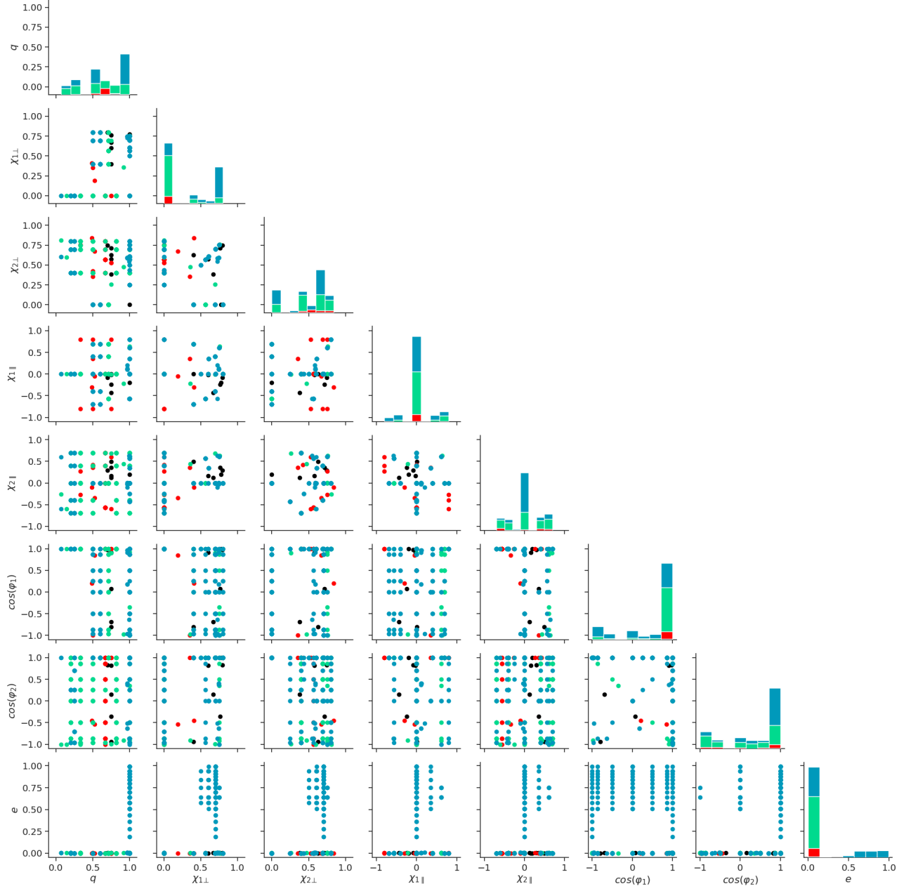
FIG. 9. Panels showing different combinations of the 8 binary parameters of the precessing parameter space ( q, \varphi_2, \chi_{1\parallel}, \chi_{1\perp}, \varphi_1, \chi_{2\parallel}, \chi_{2\perp}, \varphi_2, e ) for the 561 eccentric simulations (black first release, red second release, green third release, blue fourth release) in this catalog.
