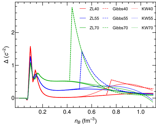
FIG. 4. Difference of squared inverse sound speeds, 1/c_{\text{eq}}^2 - 1/c_{\text{ad}}^2 for the same models as in Fig. 2.
