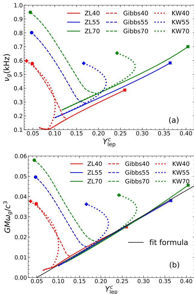
FIG. 8. (a) Comparison of the g -mode frequencies vs lepton fraction for the various EOSs with and without quarks. (b) Same as (a) but for the dimensionless quantity GM\omega_g/c^3 vs lepton fraction.
