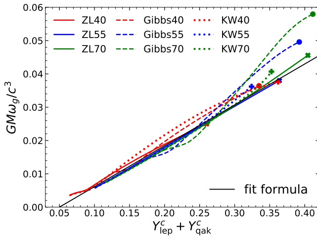
FIG. 10. Same as Fig. 8 (b) but with x-axis replaced with Y_{lep}^c + Y_{qak}^c for hybrid NS EOS.
