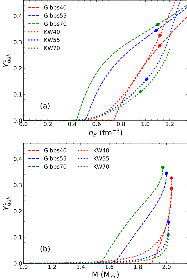
FIG. 9. Same as Fig. 7 but for quark fraction Y_{qak} in hybrid NS EOS.
