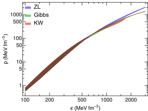
FIG. 1. Range of EOSs displayed as pressure p versus energy density \epsilon . The composition of the three models used are: for ZL, nucleons and leptons, for Gibbs, nucleons, quarks, and leptons in a soft first-order phase transition description, and for KW, the same as for Gibbs, but in a cross-over description.
