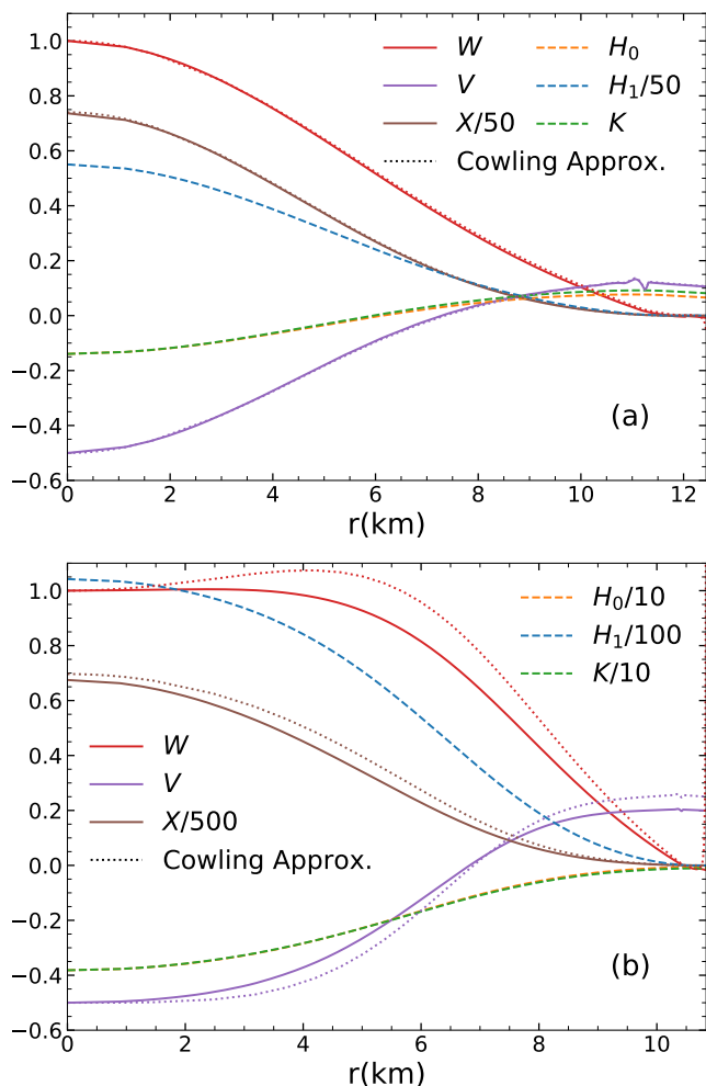
FIG. 6. g -mode fluid perturbation functions' radial profile of general relativistic (solid curves) and Cowling approximation (dotted curves) as well as metric perturbation functions' radial profile (dashed curves) with ZL55 EOS for (a) 1.4 M_{\odot} NS and (b) 2.11 M_{\odot} (maximum mass) NS. W and V are dimensionless, while H_0 , H_1 and K are in units of empirical energy density at saturation \varepsilon_s = 152.55 \text{ MeV fm}^{-3} and X is in units of \varepsilon_s^2 .
