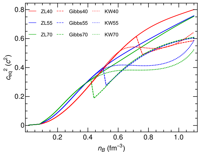
FIG. 2. Squared equilibrium sound speeds vs baryon density for the models indicated in the inset. See also text for more details.
