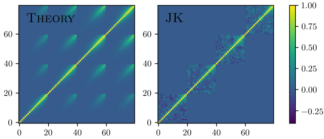
FIG. 18. Correlation matrix for the redMAGiC sample using the halo-model theory covariance from Friedrich et al. (2020) (left) and the jackknife method (right). This is a subset of the covariance for the second lens bin and each of the four source redshift bins.
