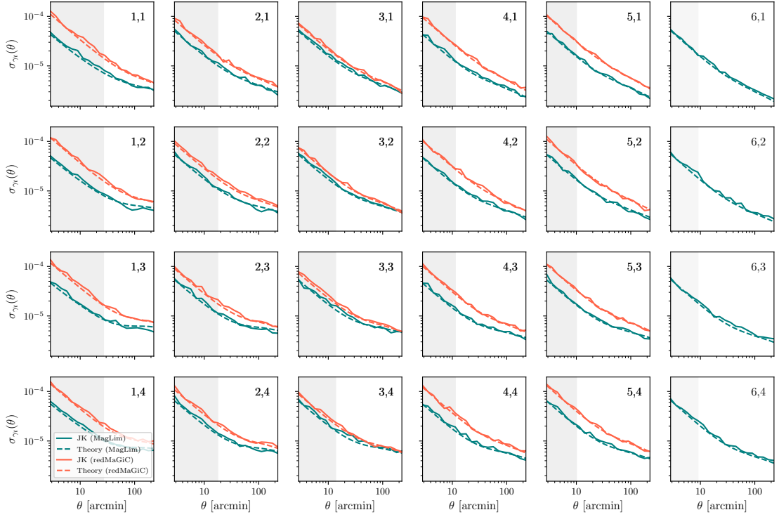
FIG. 16. Comparison of the Jackknife errorbars (JK) computed in this work as described in Sec. III F with the theory errorbars from Friedrich et al. (2020).
