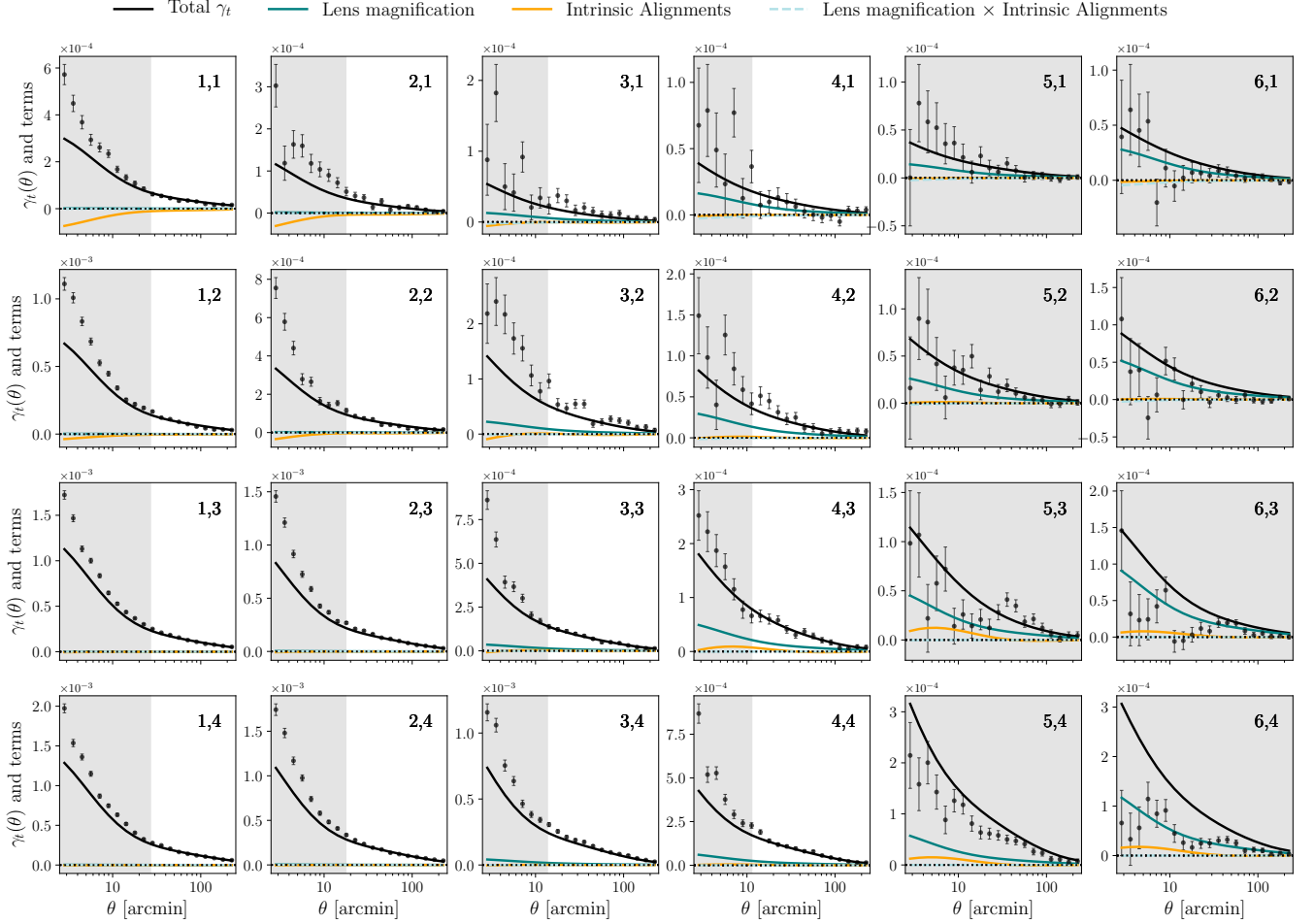
FIG. 7. This plots shows the contribution from each of the components of our model at the best-fit values from the 3\times 2 pt result for the \text{MAGLIM} sample and the total model (black line), as obtained from Eq. (53). The contribution from the coupling of IA and lens magnification is very close to zero.
