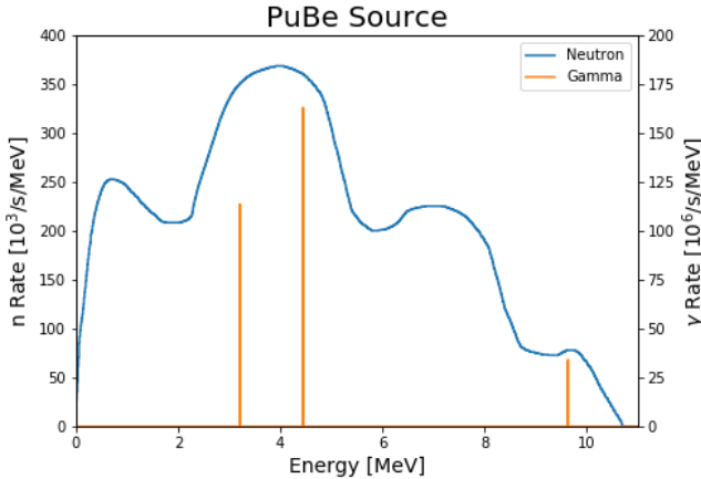
FIG. 2. (Color online) PuBe source spectrum. The neutrons from the source were measured in the early reference [28] and the gammas come from the accompanying de-excitation of the residual ^{12}\text{C} system. The neutrons are emitted in broad groups corresponding to the excitation level of the residual system and the amount of stopping experience by the \alpha prior to the (\alpha, n) reaction.
