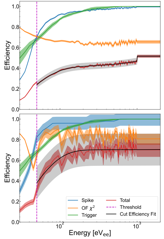
FIG. 4. (Color online) Energy-dependent efficiencies for PuBe (upper) and background (lower) datasets. Black curves show smooth functional forms of the total cut efficiency used for further analysis.
