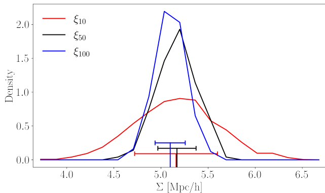
FIG. 2: Distribution of \Sigma (histograms) estimated from our Laguerre-based analysis (fit equation 5 to the measured \xi_{\text{NL}} ) of the 1500, 300 and 150 realizations of the three different effective volumes indicated (10, 50 and 100h^{-3}\text{Gpc}^3 ): larger volumes return a narrower distribution, hence a tighter constraint on the smearing scale.
