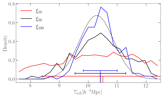
FIG. 3: Distribution of estimated \Sigma_{\text{eff}} from our Laguerre-based analysis (fit equation 5 to the measured redshift-space correlation function). Three histograms show results from 1500, 300 and 150 realizations of the three different effective volumes as indicated (10, 50 and 100h^{-3}\text{Gpc}^3 ). Vertical bars near the bottom mark the mean values of the distributions; horizontal error bars show the mean plus and minus the rms. Dashed curve shows the constraint on \Sigma_{\text{eff}} from propagating the error on a single realization of the \xi_{50} ensemble (the one shown in Figure 4); it is slightly narrower than the actual distribution of measurements in the ensemble (black histogram).
