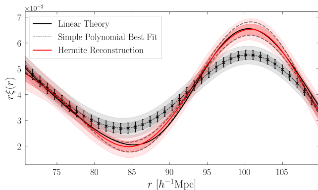
FIG. 6: Comparison of Hermite reconstruction (equation 14) of the shape of the z = 1 dark matter correlation function (solid red curve; pink bands show 1- and 2-standard deviation uncertainties) with the linear theory shape (solid black) when \Sigma = 5.1h^{-1}\text{Mpc} , the linear theory value, is used. Dashed grey curves show reconstructions when \Sigma is assumed to be larger or smaller by 10%. Symbols with error bars show the measured (i.e. evolved) dark matter correlation function; dashed black curve shows the best fit of equation (15) to these measurements, which was used to determine the a_k coefficients used in the reconstruction; grey bands show the 1- and 2-standard deviation uncertainties.
