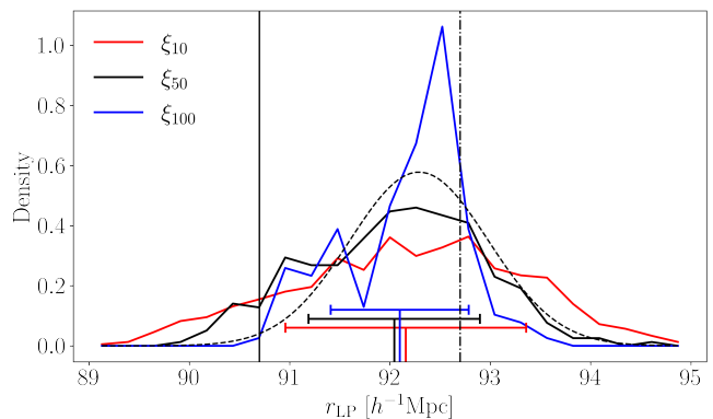
FIG. 5: Distribution of reconstructed r_{\text{LP}} from our Laguerre-based analysis (fit equation 5 to \xi_0 , the monopole of the measured redshift-space correlation function; then insert the a_k coefficients of the best fit in equation 4 to define \xi_{\text{Lag}} ; finally, determine r_{\text{LP}} from the peak and dip scales of \xi_{\text{Lag}} ). Three histograms show results for three different effective volumes as indicated. Vertical bars near the bottom mark the mean values of the distributions; horizontal error bars show the mean \pm the rms. Smooth black dashed curve shows a Gaussian distribution with mean and rms determined from the single \xi_{\text{Lag}} shown in Figure 4. Vertical solid line shows the mean r_{\text{LP}} scale measured in \xi_0 prior to reconstruction (it is similar for all three effective volumes), and dot-dashed line shows the scale in linear theory.
