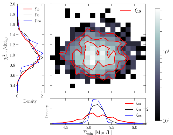
FIG. 1: Estimated \Sigma when we use exactly the correct shape and amplitude of \xi_{\text{L}} when fitting the right-hand side of equation (2) to the measured \xi_{\text{NL}} but \Sigma is determined from the fit, as well as a measure of the goodness of fit, \chi_{\text{min}}^2/\text{d.o.f.} . Main panel shows this joint distribution from 1500 realizations, each of an effective volume 10h^{-3}\text{Gpc}^3 . Histograms in bottom panel show the distribution of \Sigma for three different effective volumes as indicated (10, 50 and 100h^{-3}\text{Gpc}^3 ): as expected, larger volumes return a narrower distribution, hence a tighter constraint on the smearing scale. Histograms in the panel on the left show the associated distributions of \chi_{\text{min}}^2/\text{d.o.f.} ; as expected, the goodness of fit does not depend on the effective volume.
