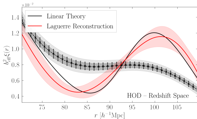
FIG. 4: Measured redshift-space monopole for a mock galaxy catalog in an effective volume of 50h^{-1}\text{Gpc} (symbols with error-bars), the 9th-order Laguerre fit to it (black dashed curve, which shows equation 5), and associated reconstruction (red curve, which shows equation 4 with the a_k determined by the black dashed curve). This particular realization happens to have \Sigma_{\text{eff}} = 10.3h^{-1}\text{Mpc} . Grey bands show the 68% and 95% range covered by 300 such realizations of the observed redshift-space monopole, and pink band shows the 68% range covered by the 300 associated reconstructed shapes \xi_{\text{Lag}} . Solid black curve shows the linear theory b_{\text{eff}}^2 \xi_{\text{L}} .
