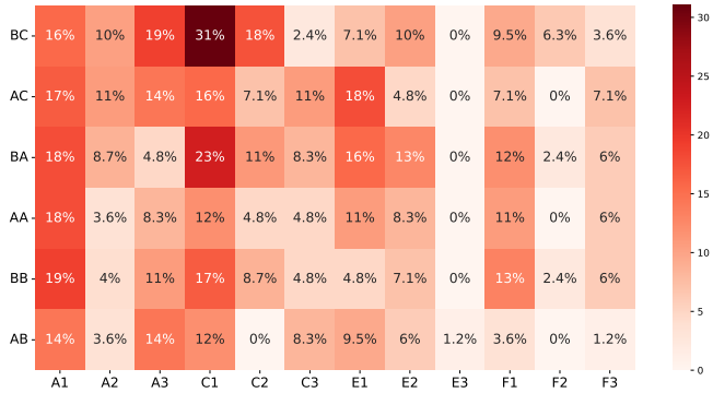
FIG. 8. Same as Figure 7, for the combination of the six choices ("BC", "AC", "BA", "AA", "BB" and "AB") of n and g(\eta) and the twelve ISM models.
