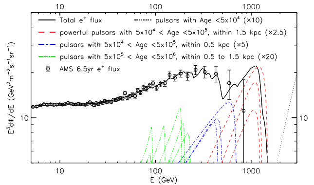
FIG. 1. The cosmic-ray positron flux from a Milky Way pulsars simulation. The solid black line includes the contribution of the cosmic-ray secondaries (from inelastic p-p, p-N and N-N collisions in the ISM). We highlight the contribution to the positron flux from individual pulsars that have ages from O(10) kyr to 5 Myr and that are relatively close-by. The contribution from individual pulsars is enhanced from the original simulation to show their fluxes within the figure. The AMS-02 observation is shown in the data points.
