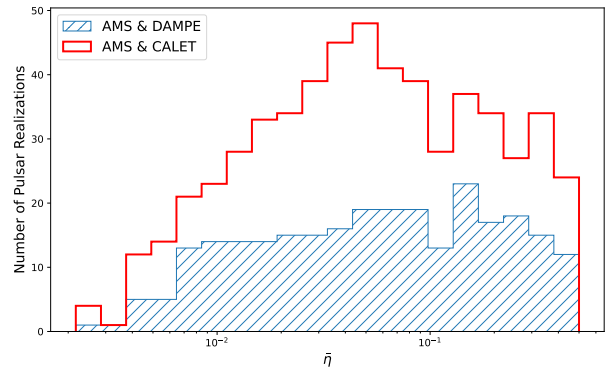
FIG. 12. The distribution of the fitted values for the averaged conversion efficiency \bar{\eta} of pulsars' spin down power to cosmic rays. The y-axis shows the number of allowed Milky Way pulsars simulations within 2\sigma . Typical values for \bar{\eta} are \simeq 0.1 .
