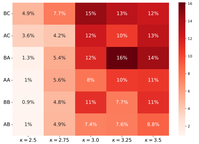
FIG. 9. Similar to Figures 7 and 8, for the combination of the six choices of n and g(\eta) and the five choices for braking index \kappa = 2.5, 2.75, 3.0, 3.25, 3.5 .
