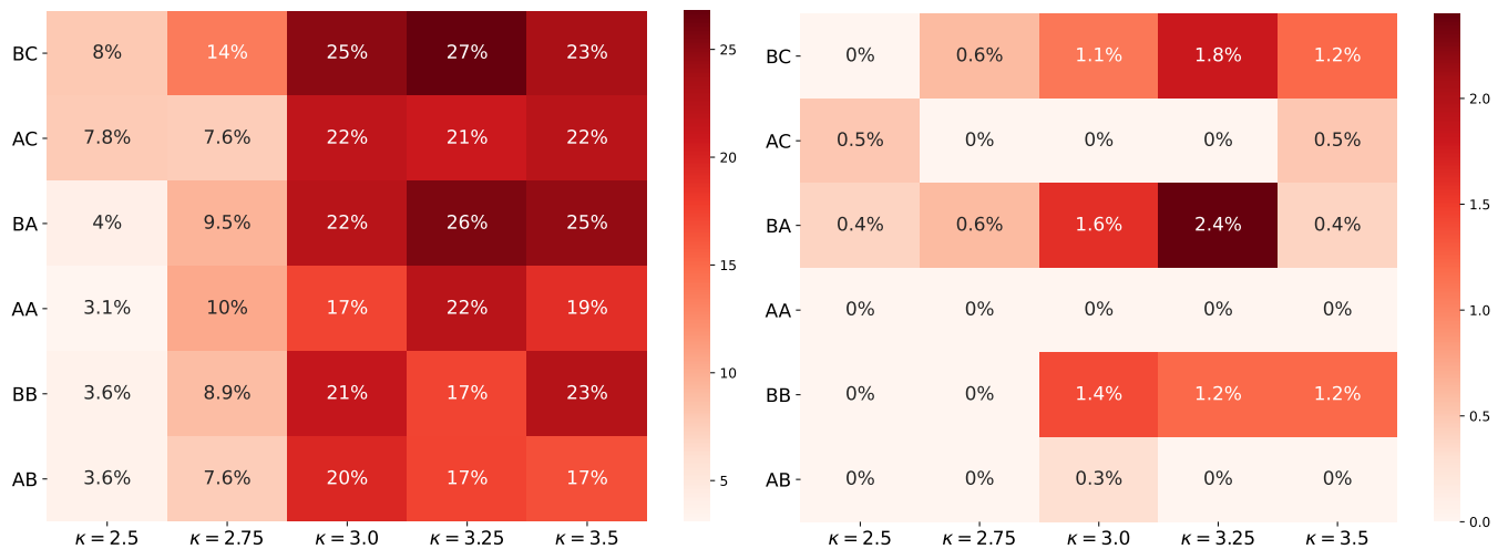
FIG. 13. Similarly to Figure 9, for given combination of pulsars' properties (each cell), we show the fraction of pulsar population simulations that are consistent within 3\sigma . On the left we have fitted the simulations to the AMS-02 observations from E > 15 GeV, and on the right to the AMS-02 observations from E \geq 5 GeV (see text for further details).
