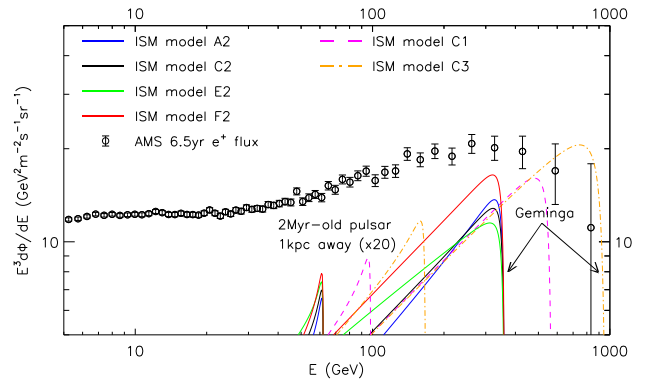
FIG. 3. The impact of different ISM assumptions on the positron flux from two individual pulsars. Solid lines (blue, black, green and red) show the impact of different diffusion assumptions. The magenta dashed and orange dot-dashed are to be compared to the black solid line that is made under the same diffusion assumptions.
