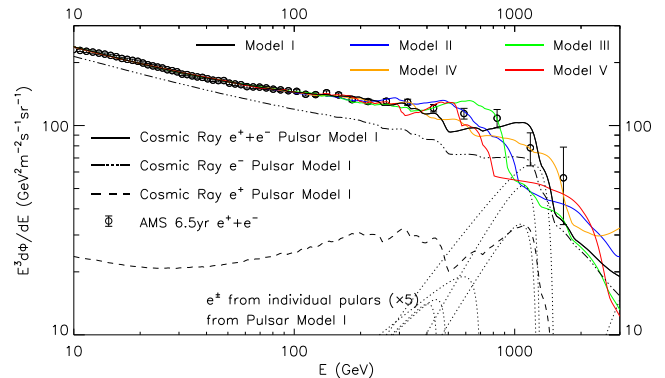
FIG. 5. The predicted e^+ + e^- spectrum for the same five pulsar simulations of Figure 4, along with the AMS-02 observation. For model I, we also show the individual electron and positron spectra and fluxes from individual pulsars.
