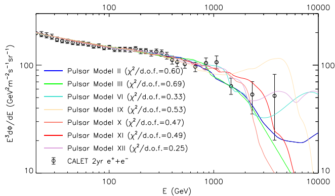
FIG. 11. Seven different predicted e^+ + e^- fluxes from realizations that can fit the CALET data and their \chi^2/\text{d.o.f.} . Pulsar Model IX, which was excluded by DAMPE in Figure 10 can fit the CALET data very well. Prominent features are also visible at the highest energies from powerful pulsars (models VI, IX, XI and XII).
