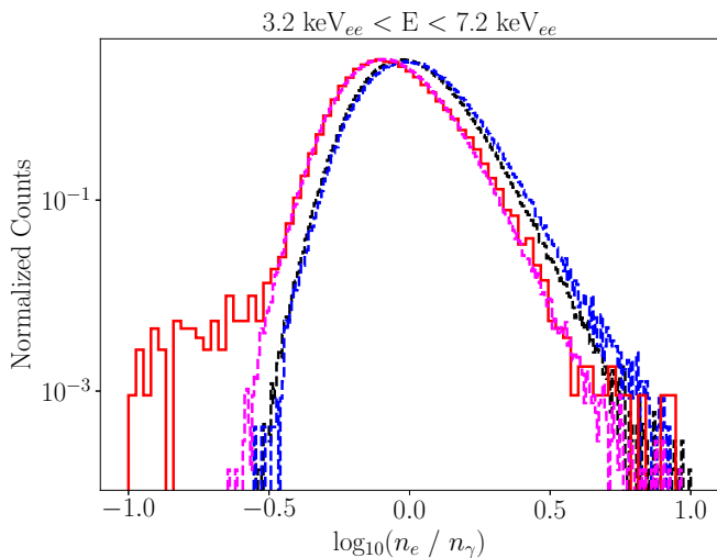
FIG. 12. Distributions of discrimination parameters for events within the 3.2–7.2 keV ee region of interest at 363 V/cm. Curves include the ^{127}\text{Xe} L-shell as measured by XELDA (red), the NEST expectations for the tritium continuum (blue), a monoenergetic \beta of 5.2 keV (black), and a monoenergetic 5.2 keV beta with our modified recombination fraction (magenta). The L-shell data, as well as our modified recombination beta, shows a clear downward shift in n_e/n_\gamma when compared to NEST expectations.
