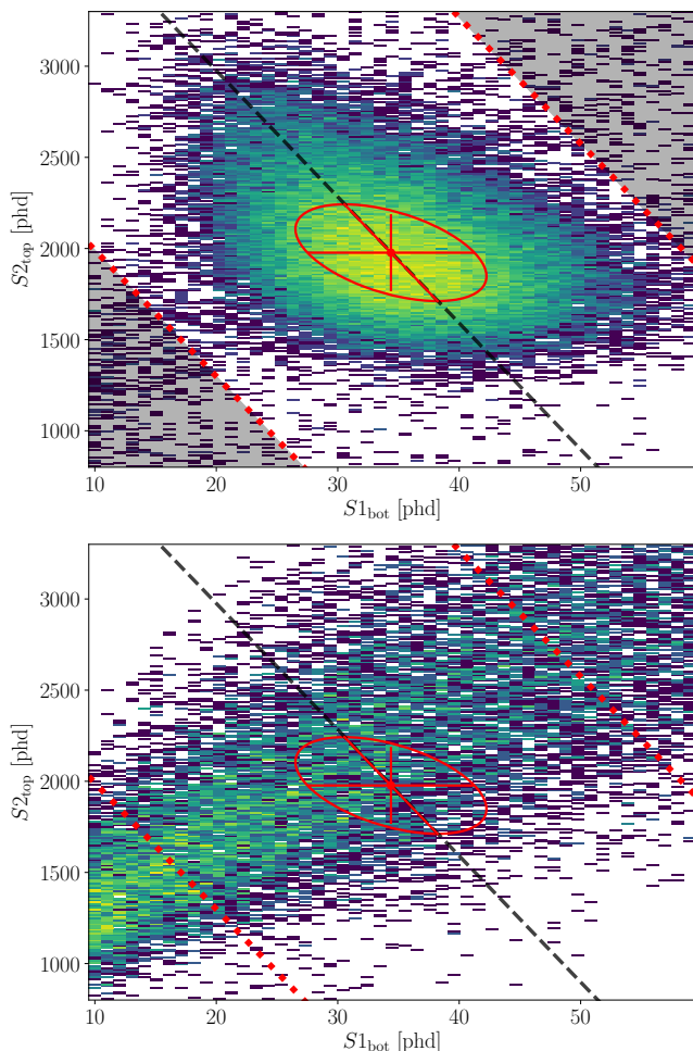
FIG. 9. (Top) The ^{127}\text{Xe} L-shell electron capture peak, as observed in the 363 V/cm data. The red dotted lines denote the limits of the energy region of interest (the shaded regions are not used in L-shell analysis), while the black dashed line denotes the 5.2 keV energy of this peak. The red point is the median in both S1_{\text{bottom}} and S2_{\text{top}} for events falling within the energy region of interest (3.20–7.20 keV), while the error bars shown denote the widths ( \sigma ) of the distribution decomposed into independent physical fluctuations: S1 fluctuations (horiz.), S2 fluctuations (vert.), and recombination fluctuations (diag.). (Bottom) The ^3\text{H} \beta -decay continuum in the K-shell energy region of interest, as observed in the 363 V/cm data, with the same lines of constant energy. The 1\sigma widths of the L-shell are drawn on top, again to illustrate the offset.
