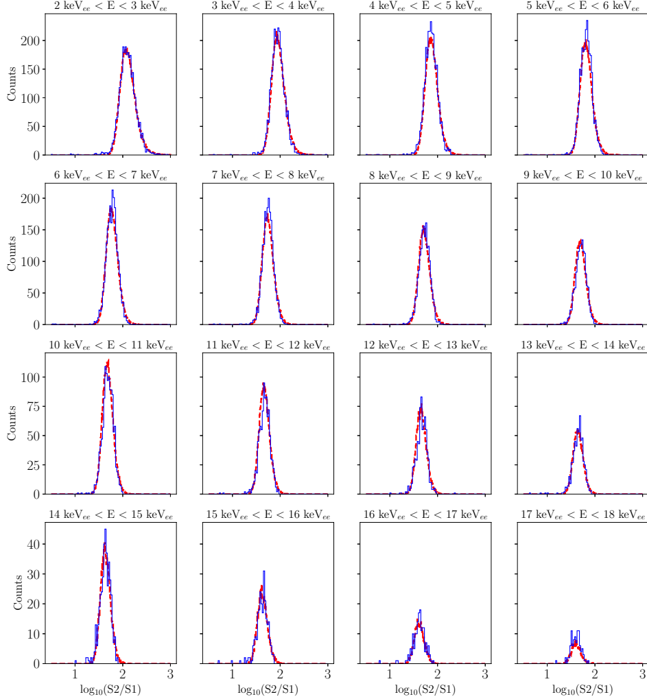
FIG. 11. Distributions of \log(S_2/S_1) for the tritium \beta -decay continuum, in 1 keV energy bins, comparing the observed tritium data (blue) to expected distributions from a NEST simulation (red) at 363 V/cm. Threshold effects become relevant for signals below 2 keV, so those bins are excluded from this analysis. Above this energy, the observed and simulated distributions are in good agreement. The slight excess in data in the 3-8 keV bins is caused by residual ^{127}\text{Xe} L-shell activity in the tritium dataset.
