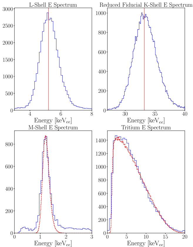
FIG. 10. Reconstructed energy distributions for the ^{127}\text{Xe} electron capture peaks and tritium continuum (bottom-right) from 363 V/cm data (blue). Vertical red lines denote the true energy of the K- (top-right) and L- (top-left) capture peaks (red). The NEST expectation for the tritium energy spectrum (red, bottom-right) in XELDA, including our 2-phd S1 threshold, is shown for comparison to the observed data. The NEST expectation for a 1.2 keV beta, also with a 2-phd S1 threshold applied, is overlaid on the M-shell peak (bottom-left). The K-shell peak is shown for a reduced fiducial volume where saturation effects are not present.
