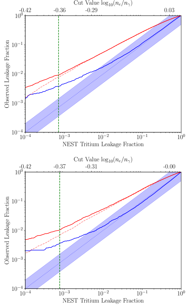
FIG. 14. The observed leakage fractions of tritium (blue) and ^{127}\text{Xe} L-shell (red) for an energy region of 3.2–7.2 keV as a function of NEST’s predicted tritium leakage fraction for the 363 V/cm (top) and 258 V/cm (bottom) datasets. The blue band shows a factor of two around y = x (perfect agreement with NEST), while the red dashed line indicates NEST’s simulation of the modified-recombination \beta model. The NR median from NEST is indicated by the vertical green dashed line. The secondary x -axis is the value of the cut in \log_{10}(n_e/n_\gamma) that gives rise to the expected and observed leakage fractions.
