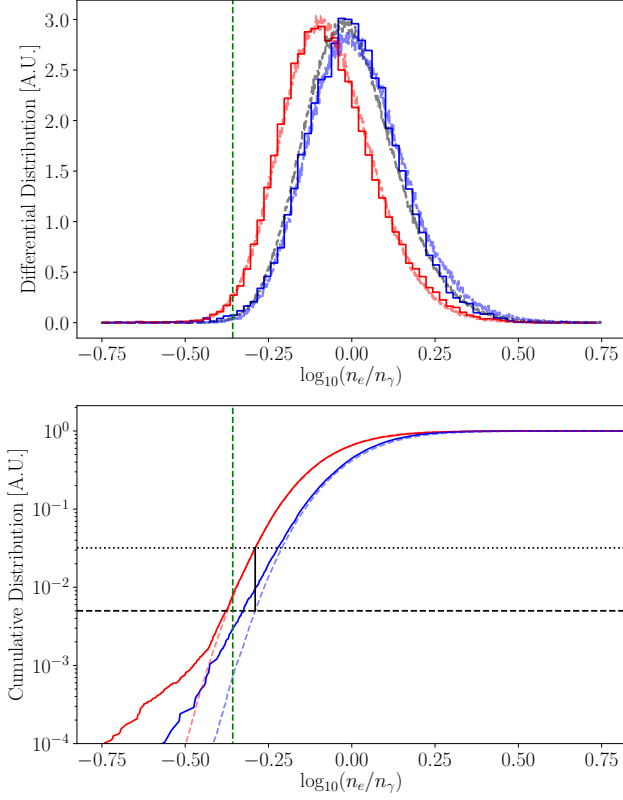
FIG. 13. Differential (top) and cumulative (bottom) distributions of \log_{10}(n_e/n_\gamma) for 363 V/cm L-shell (solid red) and tritium (solid blue) events in the 3.2–7.2 keV region of interest. The dashed curves show the NEST expectations for a 5.2-keV \beta (black, top-only), the tritium continuum in this region of interest (blue), and the modified-recombination 5.2-keV \beta (red). Also shown is the expected median of the NR distribution (green dashed). The horizontal dashed and dotted lines in the lower plot show the nominal 0.5% inefficiency predicted by NEST and 1.65% inefficiency from the L-shell data, respectively, at the cut choice indicated by the vertical black line. Data diverge from NEST expectations at low acceptance values because the NEST simulation does not include background \gamma -X events, wall leakage, and other effects that impact discrimination in small detectors.
