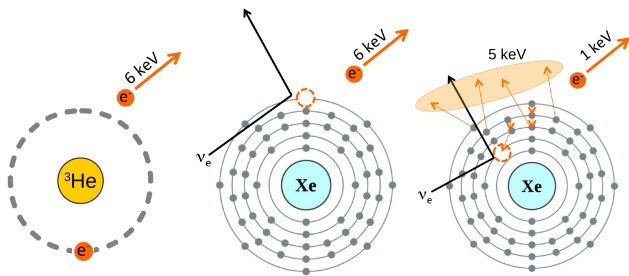
FIG. 1. A cartoon depicting a \beta -decay from tritium (left), a valence recoil from neutrino or Compton scattering (center), and an inner-shell recoil (right). Each of these interactions deposits a total of 6 keV via electron recoil(s), but the inner-shell recoil produces a distinct event topology from either the \beta -decay or valence recoil.
