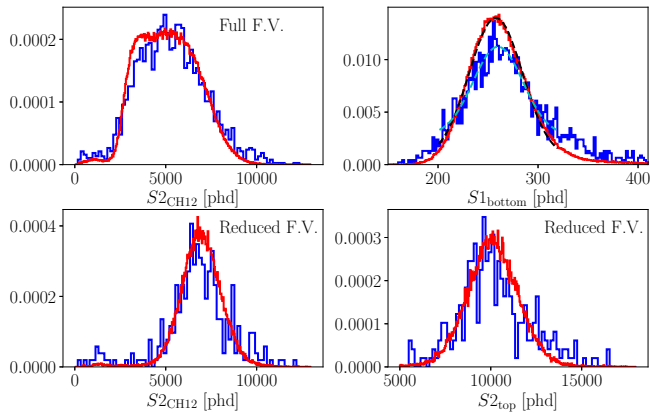
FIG. 7. Comparison of the K-shell common candles at 363 V/cm, reconstructed after cross-calibration between xenon-only and tritium datasets is complete. In each figure the red histogram shows the xenon-only distribution and the blue histogram shows the tritium distribution. Dashed curves show Gaussian fits to the S1_{\text{bottom}} distributions. The top figures use the full fiducial volume, while the bottom two use a reduced volume that is offset from the center of the detector to avoid PMT saturation effects. The vertical axis is scaled such that all the histograms integrate to unity.
