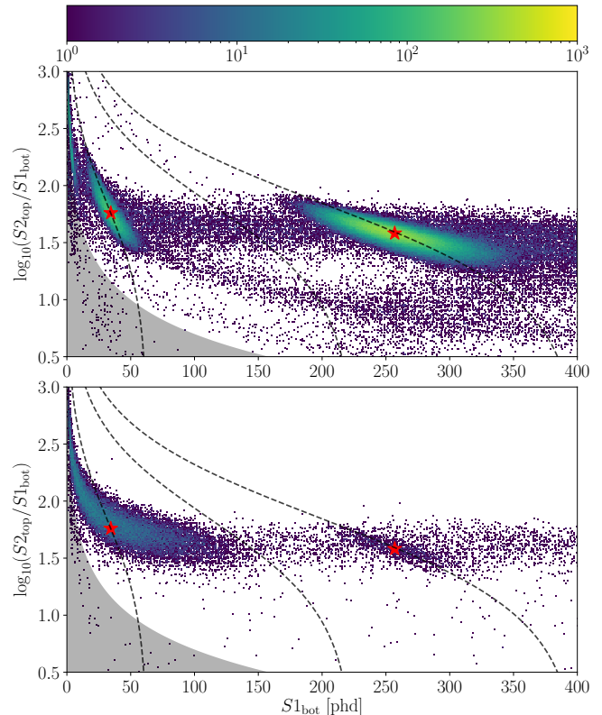
FIG. 8. Distribution of \log_{10}(S2_{\text{top}}/S1_{\text{bot}}) vs. S1_{\text{bot}} for the 363 V/cm Xe-only data (top) and ^{127}\text{Xe} plus tritium data (bottom). The dashed curves denote constant energies at 33.2 keV (K-shell), 18.6 keV (tritium Q -value), and 5.2 keV (L-shell). The color represents the absolute counts per bin, and the scale is logarithmic. The red stars indicate the centroids of the K- and L-shell distributions, as determined by the Xe-only data set. Those points are reproduced in the tritium data to help guide the eye. The L-shell centroid is clearly offset below the center of the tritium band. The grey regions indicate the analysis threshold, and events in this region are excluded from the analysis.
