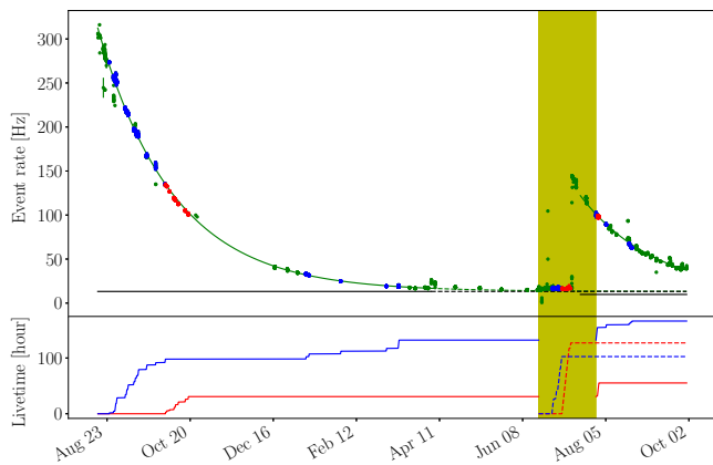
FIG. 5. Trigger rates (above) and accumulated livetimes (below) for data taken by XELDA from August 2018 through October 2019. Above: Blue and red points in the rate plot indicate data used in this paper at 363 and 258 V/cm, respectively. Green points indicate datasets not used in analysis but shown here to illustrate the decay of ^{127}\text{Xe} in the detector. These runs were rejected due to effects including poor electron lifetime ( <10 \mu\text{s} ), unstable liquid level, lack of clear single- and double-electron peaks in the S2 spectrum, or abnormal trigger rate. Lines indicate fits to the data rate taking a flat background plus decaying exponential with fixed 36.3-day half-life. The shaded band indicates the period where tritium is present in the detector. In the bottom panel, solid(dashed) lines indicate xenon-only(tritium) livetimes.
