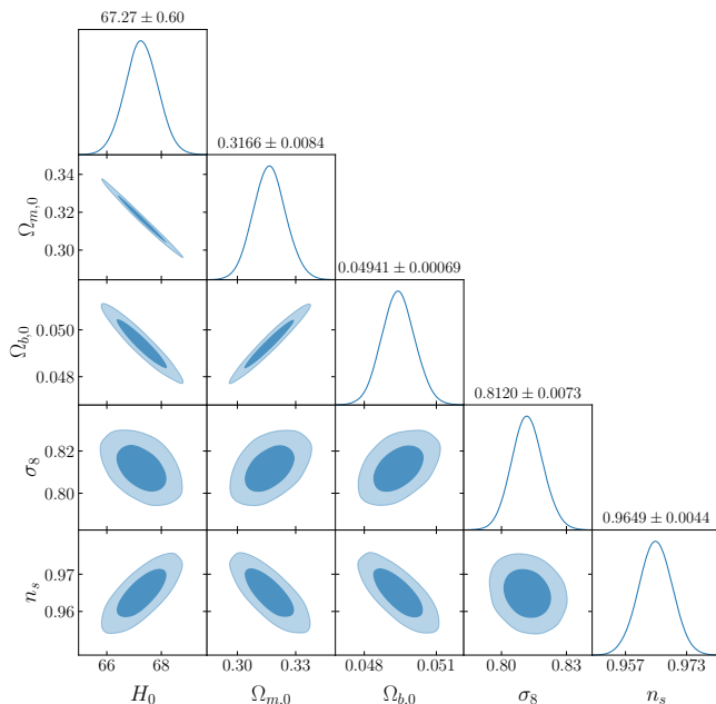
FIG. 8. Planck 2018 CMB TT,TE,EE+lowE constraints on the five background cosmological parameters considered in this work, recompiled from Monte Carlo chains provided using GETDIST [68, 69]. Contours show 68% and 95% confidence regions. The corresponding covariance matrix will be used as prior information in our Fisher analyses, see Section V E.
