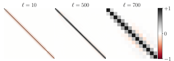
FIG. 14. Similar as Fig. 13 but for SFB galaxy power spectra. The upper left corner corresponds to lower k_{\ell n} modes.
