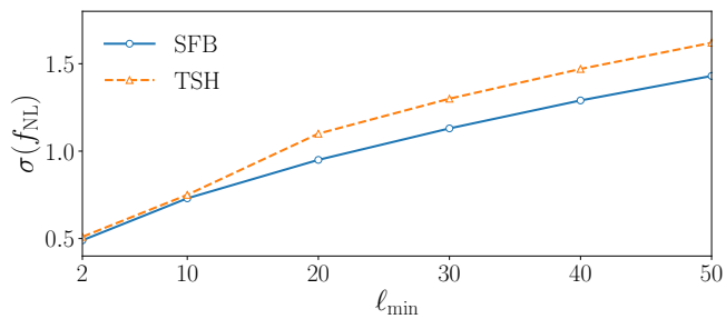
FIG. 11. Dependence of \sigma(f_{\text{NL}}) on the minimum multipole \ell_{\text{min}} used for Fisher analyses, shown for the LSST sample (joint analyses with CMB lensing and with Planck prior added) as an example.
