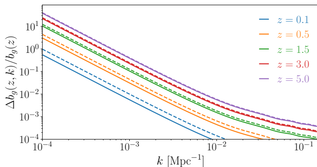
FIG. 1. Redshift and scale dependence of the clustering bias correction due to PNG of local type, shown as the fractional change to the fiducial bias b_g(z) assuming f_{\text{NL}} = 1 . Lines are plotted for b_g(z) = 1/D(z) (solid) or b_g(z) = 1 + z (dashed), which represent two typical types of redshift dependence.
