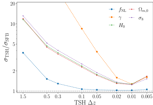
FIG. 12. The ratios between parameter constraints given by TSH and SFB analyses of the Euclid -like galaxy sample, with CMB lensing included. To get a more straightforward idea about the dependence of background cosmological parameters on the bin size \Delta z in TSH analysis, Planck CMB prior is not added. See Section VID for more details.
