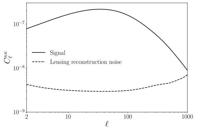
FIG. 2. CMB lensing convergence power spectrum and the lensing reconstruction noise discussed in Section III C 1.
