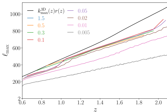
FIG. 6. Linear modes in TSH analysis of the Euclid galaxy sample, where each mode is specified by the redshift bin size and the angular multipole \ell . Each line labelled by the tomographic redshift bin size shows the maximum \ell for each bin determined by the linear requirement. As a reference, we also show k_{\max}^{\text{3D}}(z)r(z) , which is usually used to convert k to \ell for a single redshift bin. See Section VB for more details.
