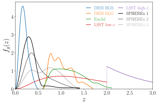
FIG. 3. Redshift distributions of the galaxy samples, the integrals of which are normalized to one in the redshift range covered. Note that the LSST high- z sample extends to z = 5 though we truncate the plot at z = 3 for better clarity.
