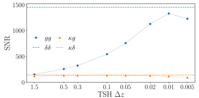
FIG. 9. SNRs of TSH power spectra \mathbf{C}^{gg} and \mathbf{C}^{\kappa g} with different bin sizes for the Euclid galaxy sample. SNRs of SFB power spectra \mathbf{C}^{\delta\delta} and \mathbf{C}^{\kappa\delta} are also shown as horizontal dashed lines for reference.
