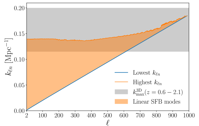
FIG. 5. Linear modes in SFB analysis of the Euclid galaxy sample, where each mode is specified by the angular multipole \ell and the discrete radial wavenumber k_{\ell n} . The blue line shows the lowest k_{\ell n} we could have for each \ell under the boundary condition, while the orange line denotes the highest k_{\ell n} determined by the linear requirement. Thus all the linear modes that will be included in the Fisher analysis are covered by the enclosed orange area. As a reference, we also show the maximum 3D linear wavenumber k_{\text{max}}^{\text{3D}} , which evolves with redshift, in the grey shaded area. See Section V B for more details.
