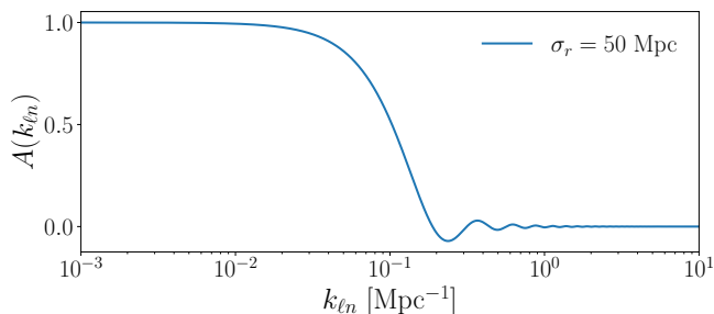
FIG. 7. Spectral window function (Eq. (54)) multiplied to the galaxy SFB modes. The example line is shown for a redshift uncertainty \sigma_r = 50 Mpc, which roughly corresponds to \bar{\sigma}_z = 0.01 centered at z = 0.7 (e.g. the SPHEREx 2 sample).
