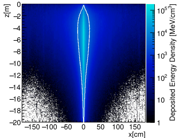
FIG. 5. A one centimeter wide, two-dimensional slice of the in-ice energy density distribution along the cascade axis for a primary proton with E= 10^{17} \text{ eV} . The solid white line outlines the region for which the plasma frequency exceeds 100 MHz.
