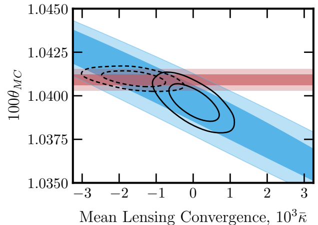
FIG. 7. Constraints in the \bar{\kappa} vs. \theta_{MC} plane from SPT-3G 2018 without (blue contour) and with (solid black line) a prior on the mean convergence. Contours indicate the 68% and 95% probability regions. Using SPT-3G 2018 data alone the two parameters are degenerate with one another, unless a prior is placed on the mean convergence. The red band indicates the 2\sigma range of the latest Planck value for \theta_{MC} . From the joint constraints from SPT-3G 2018 and Planck without a prior on \bar{\kappa} (dashed black lines) we infer \bar{\kappa} < 0 at 2.9\sigma .
