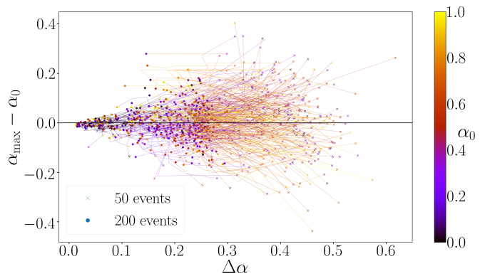
FIG. 4. Evolution of the shift and the error on \alpha (90% confidence interval) with the number of observed events. We consider two sets of observations, with 50 events (crosses) and 200 events (dots). The color scale indicates the value of \alpha_0 . As expected, they tend to decrease as we observe more events. The fact that the points are equally distributed on both sides of the \alpha_{\text{max}} = \alpha_0 line indicates that there is little systematic bias in our analysis.
