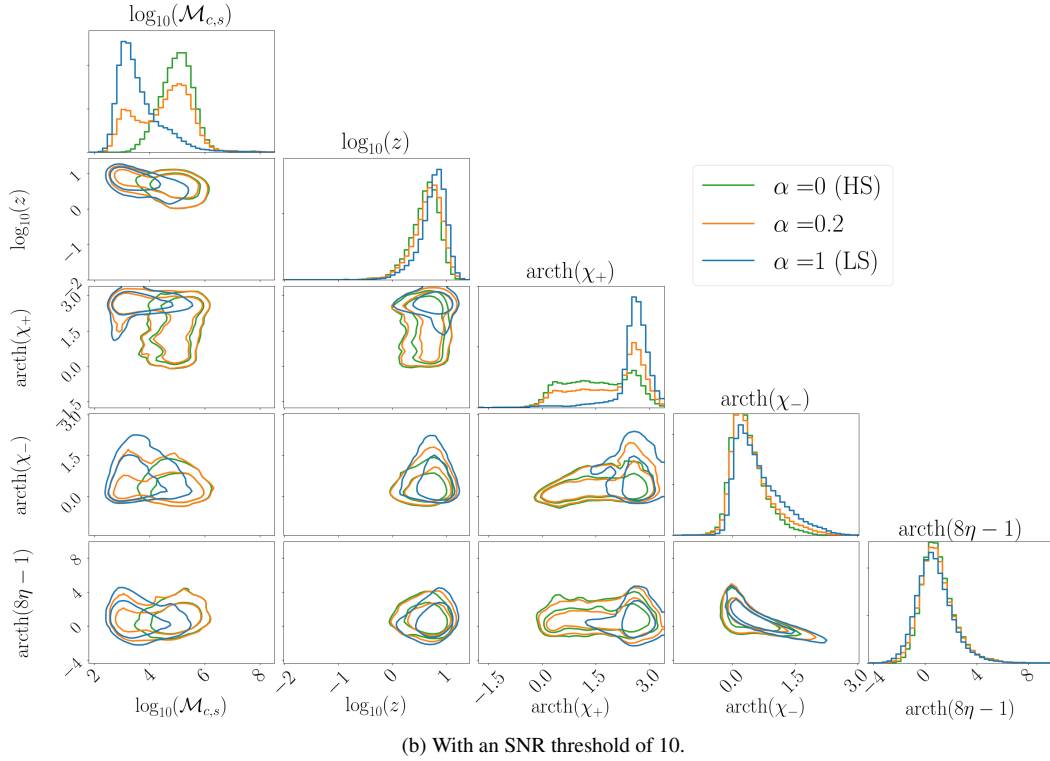
FIG. 1. Normalized population distribution for different values of the mixing fraction between the fiducial LS and HS models. We show the 68% and 90% confidence intervals. The (source-frame) chirp mass distribution is the most sensitive to \alpha . The redshift distributions of detectable events look much more similar, unlike the effective spin distributions, as discussed in the main text.
