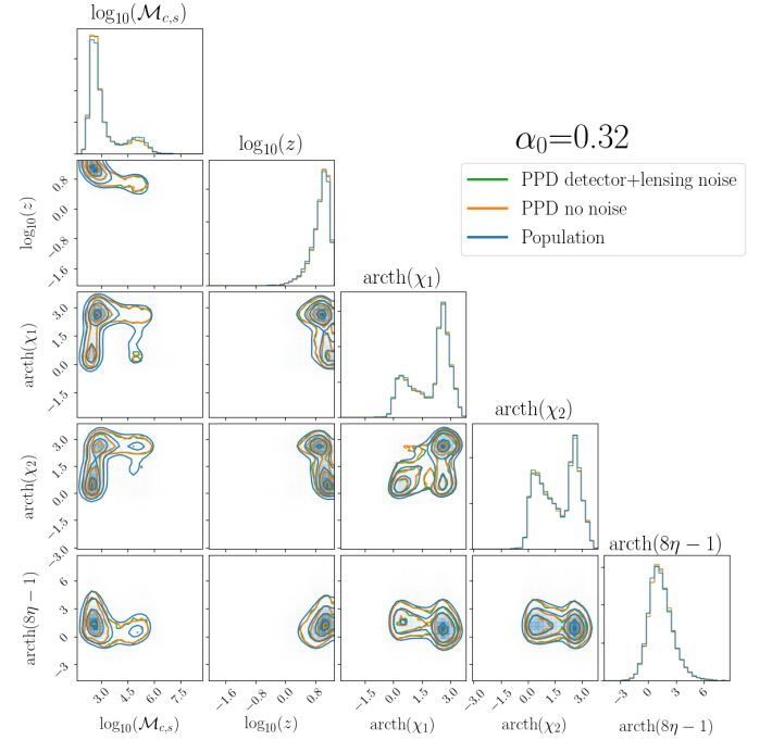
FIG. 9. Population distribution and PPDs obtained in the no-noise and detector+lensing noise scenarios for a representative case. The data set contains 500 events (before applying the detectability criterion). Including measurement errors barely affects our ability to infer the population distribution.
