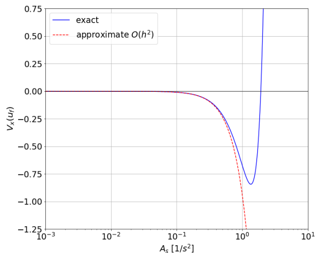
FIG. 1: This plot summarizes the results of numerically integrating the Brinkmann equations of motion versus approximating the equations of motion with perturbation theory. The red dotted curve (approximate) shows how much the \mathcal{O}(h^2) energy density term contributes to the total velocity memory effect at a fixed amplitude of the sandwich wave. The solid blue curve (exact) is calculated from numerically integrating the metric, which includes all terms. We begin to see agreement between the two curves as the amplitude decreases below A_s \sim 0.5 \text{ sec}^{-2} , implying that for weaker gravitational sandwich waves, the velocity memory is well approximated by just the energy density term. Higher order terms are responsible for the disagreement between the two curves for larger amplitudes. For reference, the sandwich wave studied in [46] had an amplitude of A_s = 1 \text{ sec}^{-2} .
