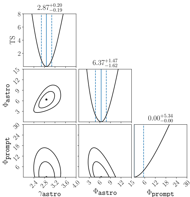
FIG. 15. Single power-law profile likelihood. Diagonal panels show the TS, as a function of different model parameters, and the one sigma intervals assuming Wilks’ theorem. Other panels show the best-fit point and two-dimensional contours. Solid (dashed) contours represent the 68.3% (95.4%) confidence regions assuming Wilks’ theorem. The parameter \gamma_{\text{astro}} is the single power-law spectral index, \Phi_{\text{astro}} is a scaling factor of the astrophysical flux at 100 TeV, and \Phi_{\text{prompt}} is a scaling factor of the BERSS prompt neutrino flux calculation [103]; further descriptions of these parameters are provided in Section V, Eq. (9), and Eq. (1)
