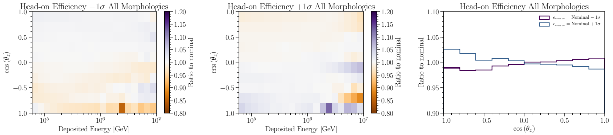
FIG. 31. Effect of changing the hole ice on the sample. The layout and colors have the same meaning as in Fig. 30, and show the effect of decreasing and increasing the head-on efficiency. Since this effect is predominantly an effect in the angular distribution, the right most panel shows the ratio to nominal as a function of the cosine of the zenith angle. In these three panels all morphologies are considered.
