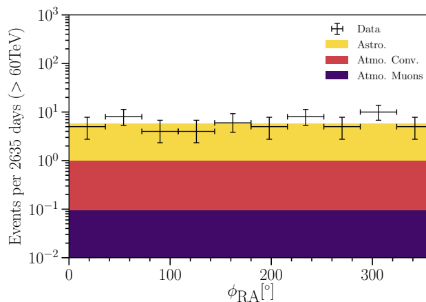
FIG. 29. Right ascension distribution. Events above 60 TeV are shown together with the stacked expectation of different components using simulation weighted with the best-fit parameters for the single power-law astrophysical model. This figure has the same format as Fig. 14
