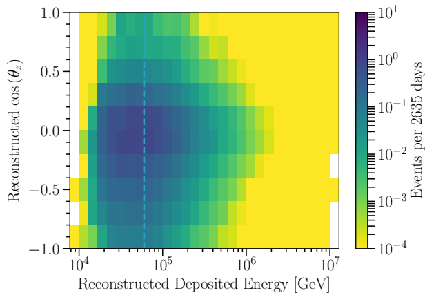
FIG. 10. Expected distribution of atmospheric neutrinos produced by pions and kaons in the sample. Distribution of neutrinos that pass the veto as a function of the deposited energy and the cosine of the zenith angle assuming nominal values for the nuisance parameters. The dashed line at 60 TeV marks the low energy cut of the analysis. Suppression in the down-going region is due to the veto. Suppression in the up-going region is due to absorption of neutrinos in the Earth.
