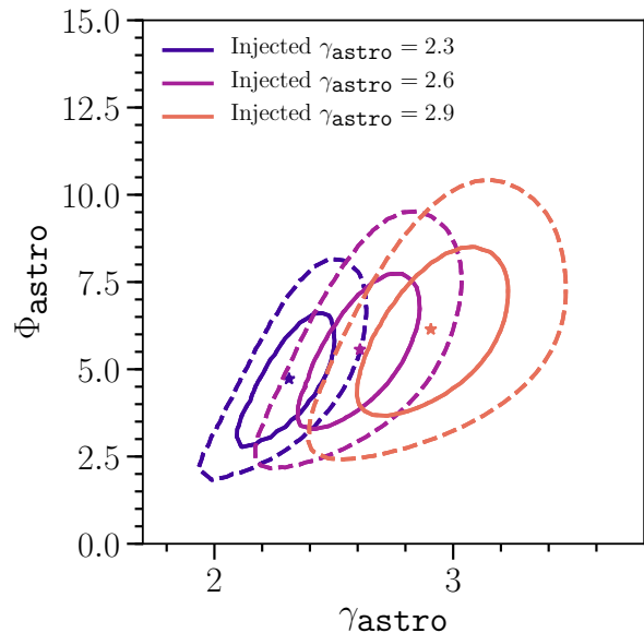
FIG. 18. Astrophysical parameter sensitivity to injected spectra. The three colors from blue to salmon show the expected astrophysical parameter 68.3% (solid lines) and 95.4% (dashed lines) uncertainty for three injected astrophysical spectra \gamma_{\text{astro}} \in \{2.3, 2.6, 2.9\} . In each of these cases the expected number of events for 7.5 years of livetime is injected as data using nominal values for nuisance parameters and holding the number of injected astrophysical events to be equal between the spectra. As expected, the spectral index uncertainty grows with softer spectra from \sim 0.14 to \sim 0.21 when changing \gamma_{\text{astro}} from 2.3 to 2.9.
