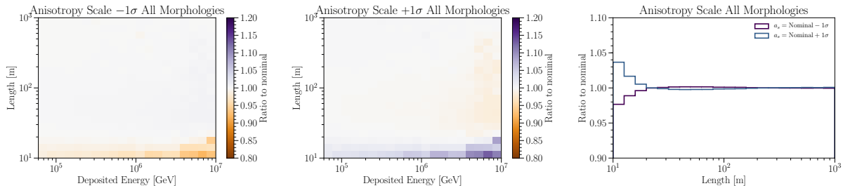
FIG. 32. Effect of changing ice anisotropy on length distribution in the sample. The layout and colors have the same meaning as in Fig. 30, and show the change relative the baseline to ice model anisotropy. The right most panel shows the ratio of length distributions, when decreasing and increasing the anisotropy, as dark and light lines as a function of the reconstructed length. In these three panels all morphologies are considered.
