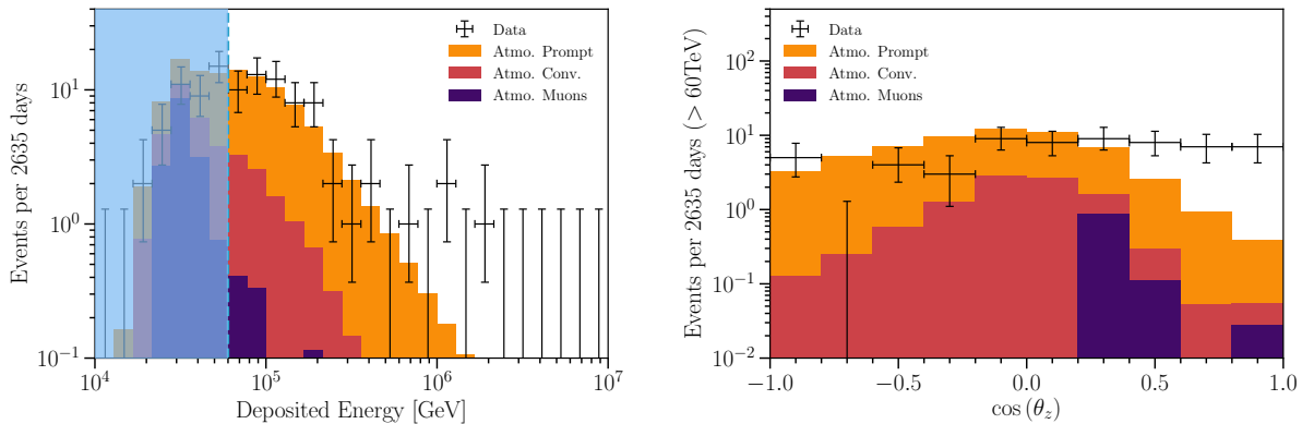
FIG. 25. Atmospheric-background-only fit to the data. In these figures we present the best fit distribution from simulation in the absence of an astrophysical component as stacked histograms. The left panel shows the deposited energy distribution and the right panel the angular distribution. As can be seen in the right panel, the angular distribution is in tension with the expectation in several bins. This amounts to a greater than 5\sigma difference with respect to the best-fit astrophysical model. The colors of the stacked histogram are the same as in Fig. 14, and the data is shown as black crosses.
