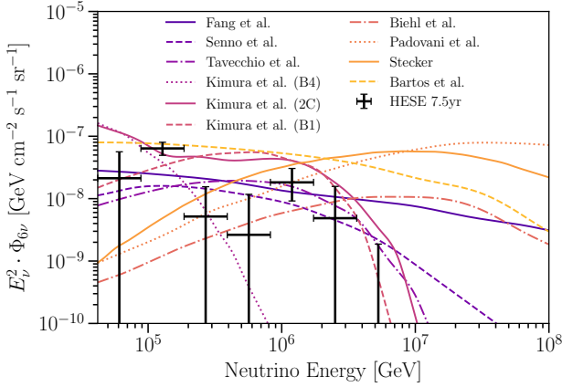
FIG. 28. Source-specific models tested in this work together with the segmented-fit outcome. Models discussed in Section VIC and listed in Table XII are shown as lines. The HESE segmented power-law model, described in Section VIA 5, best-fit normalizations are shown as black crosses. Models are ordered in the color scale from largest (darkest color) to smallest (lightest color) evidence as reported in Table XII.
