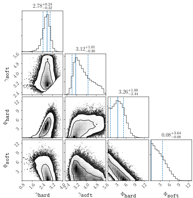
FIG. 20. Double power-law model hard/soft parameters posterior distribution. Results derived from the posterior distribution of the double power-law model are shown in the same style as Fig. 19. The figure shows the one- and two-dimensional posterior distributions for the parameters of the hard and soft components of the astrophysical neutrino flux. The diagonal panels show the one-dimensional posterior with the parameter MAP estimation and 68.3% HPD region indicated, while the non-diagonal panels show the two-dimensional posterior with 68.3% and 95.4% regions indicated.
