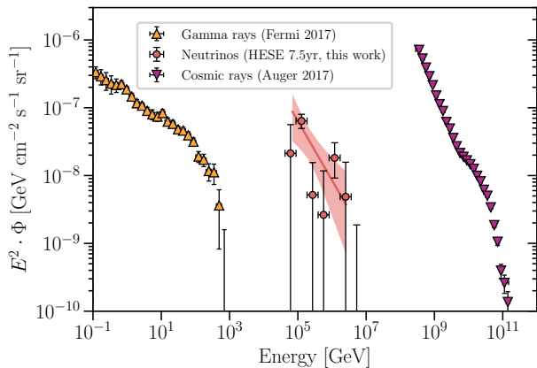
FIG. 1. High-energy fluxes of gamma rays, neutrinos, and cosmic rays. The segmented power-law neutrino flux, described in Section VIA 5, obtained in the analysis described in this paper, is shown with red circles. The single power-law assumption, described in Section VIA 1, is shown with the light red region. The high-energy gamma-ray measurements by Fermi [75] are shown in orange, while the extremely-high-energy cosmic-ray measurements by the Pierre Auger Observatory [76] are shown as purple data points. The comparable energy content of these three fluxes is of particular interest in the investigation of cosmic-ray origin.
