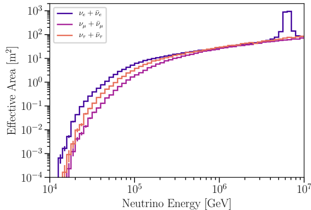
FIG. 33. All-sky energy dependent astrophysical neutrino effective area. The direction averaged effective area for the three neutrino flavors is shown as a function of the neutrino energy incident on Earth. This effective area takes into account the effects of absorption in the Earth. To obtain the expected number of astrophysical neutrinos, this effective area can be multiplied by the all-sky astrophysical neutrino flux. On the other hand, to obtain the expected number of atmospheric events, the atmospheric passing fraction must be included in the calculation of the effective area.
