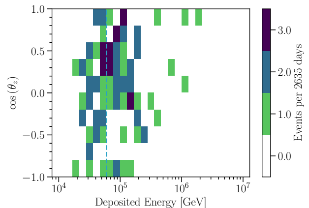
FIG. 7. HES E events observed in 7.5 years. Histogram of the observed events as a function of their inferred deposited energy and cosine of the reconstructed zenith angle. The dashed line indicates the low-energy threshold of 60 TeV.
