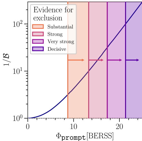
FIG. 26. Prompt neutrino normalization constraints. The horizontal axis shows the size of the prompt normalization with respect to the baseline BERSS model discussed in Section IV with passing fractions given in [122]. The vertical axis gives the reciprocal of the Bayes factor; decreasing Bayes factors imply a more disfavored prompt normalization. The shaded regions denote exclusions of the prompt normalization according to Jeffreys’ scale from substantial to decisive.
