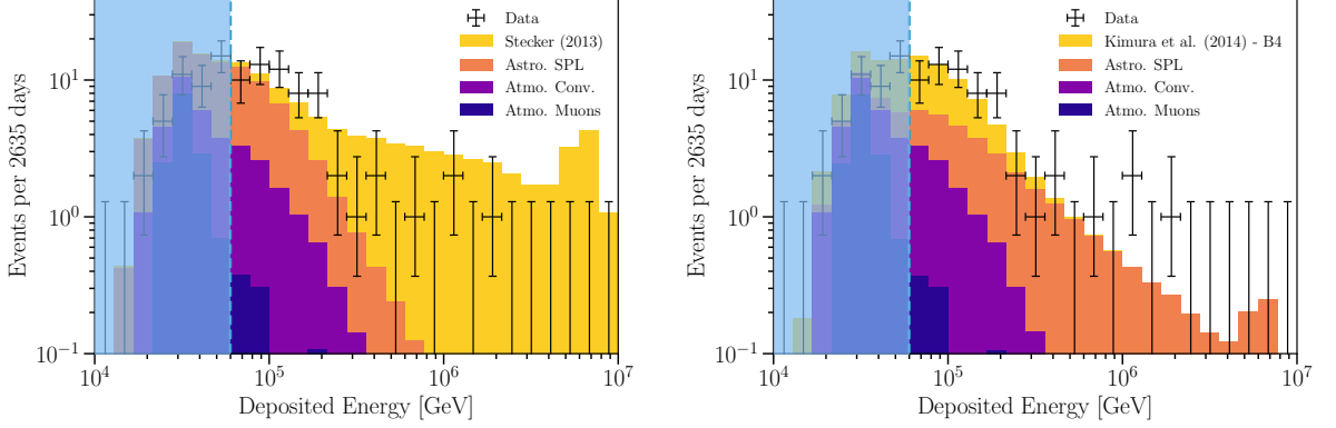
FIG. 27. Source-specific model energy distributions. Different panels show the predicted energy distribution compare to the data for a subset of the models considered in Table XII. In the cases shown above there are two astrophysical components: a specific source model and an additional single power-law component. All the components are shown as a stacked histogram at the best-fit value of the components normalizations. Left: The Stecker [200] model is shown as an example of a case where the Bayes factor assuming equally likely alternatives indicates significant preference for the single power-law model over the two component scenario. Right: The Kimura et al. (B4) [202] model is shown as an example of a case where an additional single power law is needed to explain the distribution of events.
