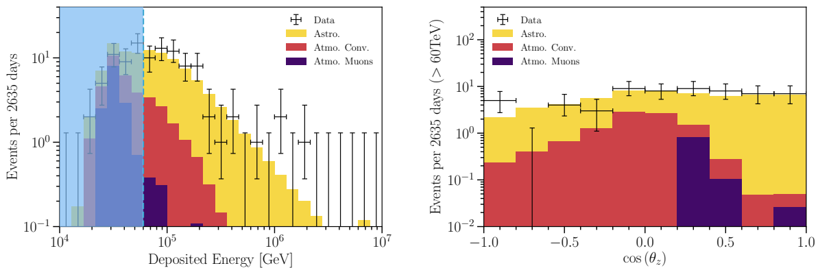
FIG. 14. Deposited energy and reconstructed \cos \theta_z distributions. In these panels, the data is shown as crosses and the best-fit expectation as a stacked histogram with each color specifying a given flux component: astrophysical neutrinos (golden), conventional atmospheric neutrinos (red), and penetrating atmospheric muons (purple). Left: distributions of events and expected event count assuming best-fit parameters as a function of the deposited energy; events below 60 TeV (light blue vertical line) are ignored in the fit. Right: distribution of events with energy greater than 60 TeV in the cosine of their reconstructed zenith angle. Up-going events are on the left side of this panel and down-going events on the right. The expected number of events is split by components and displayed as a stacked histogram. The normalization of the prompt atmospheric neutrino component fits to zero, and so is not shown in the stacked histogram. The distribution of data events appears to be largely flat as a function of cosine zenith with a small decline towards the up-going region. The lower event rate in the up-going region is expected as a result of the Earth’s absorption of the neutrino flux, and appears to be compatible with the Monte Carlo expectation.
