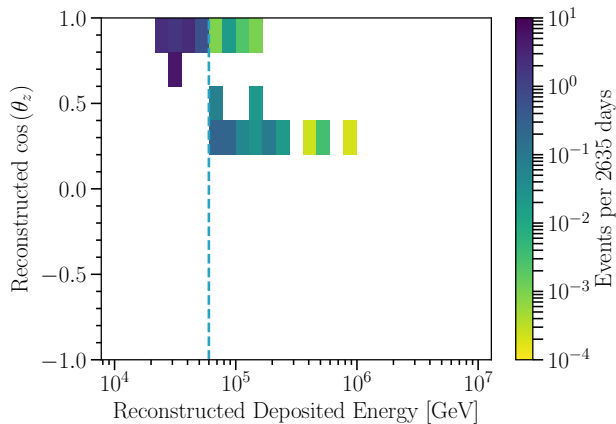
FIG. 13. Expected distribution of atmospheric muons in the sample. Distribution of muons that pass the veto as calculated with MUONGUN as a function of the deposited energy and the cosine of the zenith angle. The normalization is set to match the data driven sub-detector study. The dashed line at 60 TeV marks the low energy cut of the analysis.
