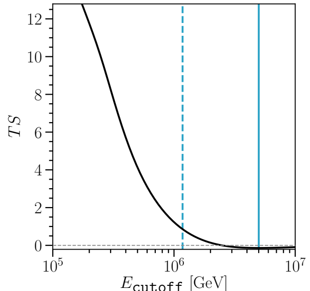
FIG. 22. Cutoff model comparison using frequentist test-statistic. The test-statistic comparing the cutoff hypothesis and the single power-law hypothesis is plotted as the black curve. The gray dashed line indicates where the cutoff model's test-statistic and the single power-law model are equal; there is a slight preference for the cutoff scenario in the several PeV region, although this is not statistically significant. We also report the results of parameter estimation for the cutoff model in this plot. The best-fit value for the cutoff energy, E_{\text{cutoff}} , is shown as the solid blue line and the dashed blue line indicates the boundary of the 68.3% confidence interval.
