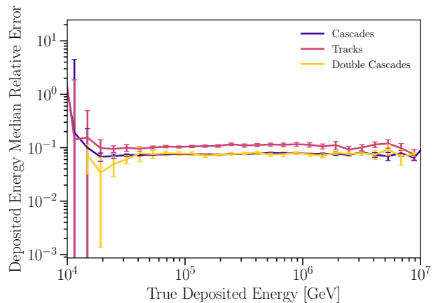
FIG. 4. Deposited energy resolution. Each line shows the median energy resolution plotted as a function of the true deposited energy in the detector for a reconstructed morphology. The error bars indicate the statistical uncertainty in the calculation of the median. At these energies the uncertainty of the cascade deposited energy is affected by the spatial extension of the showers not modelled by the reconstruction, whereas the uncertainty in track deposited energy is dominated by the stochasticity of the losses.
