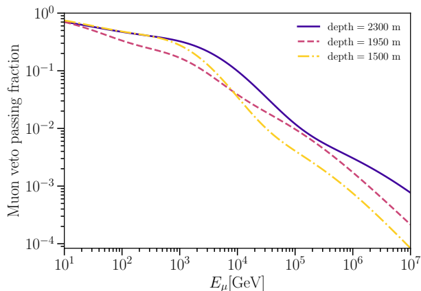
FIG. 8. Muon veto passing fraction. Each line shows the fraction of muons of given energy at the detector edge, E_\mu , that pass without triggering the veto when entering the detector at a particular depth. Three depths are shown: 1500, 1950, and 2300 meters from the surface, with lines of darkening color as the depth increases. The veto efficiency increases with the muon energy. Differences at various depths are due to the changing ice properties and varying acceptance as a function of depth due to the veto region’s asymmetric structure. At the top of the detector, the veto region is larger, so it is more efficient at rejecting muons. Additionally, the horizontal veto layer just above the dust region provides more rejection power for muons intersecting with it. Finally, the expected angular distribution of incident muons is dominated by vertical events which are more easily rejected by the upper veto region. Above \sim 10 TeV, limited simulation samples are available to assess the response, and above \sim 100 TeV the function is entirely extrapolated. At all depths the sum of a sigmoid function and a Gaussian distribution is fit to the results of muon simulation.
