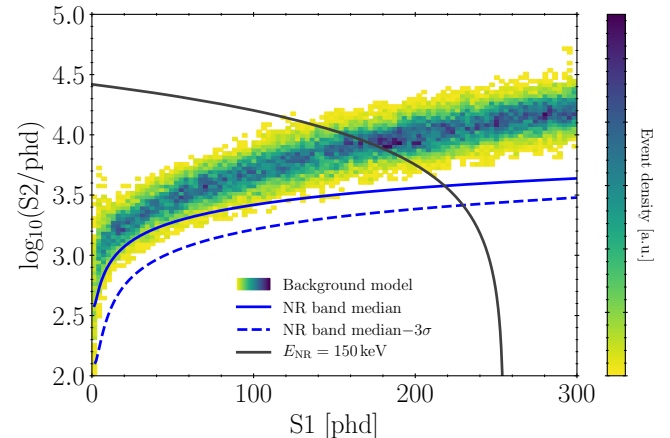
FIG. 5. Simulated ER background event density in LUX for a 118-kg fiducial volume (18-cm radius). The median (solid blue) and median -3\sigma (dashed blue) contours of the NR band are shown. The WIMP signal region is defined as the region between these two blue contours, up to the gray contour which represents a nuclear recoil energy ( E_{\text{NR}} ) of 150 keV.
