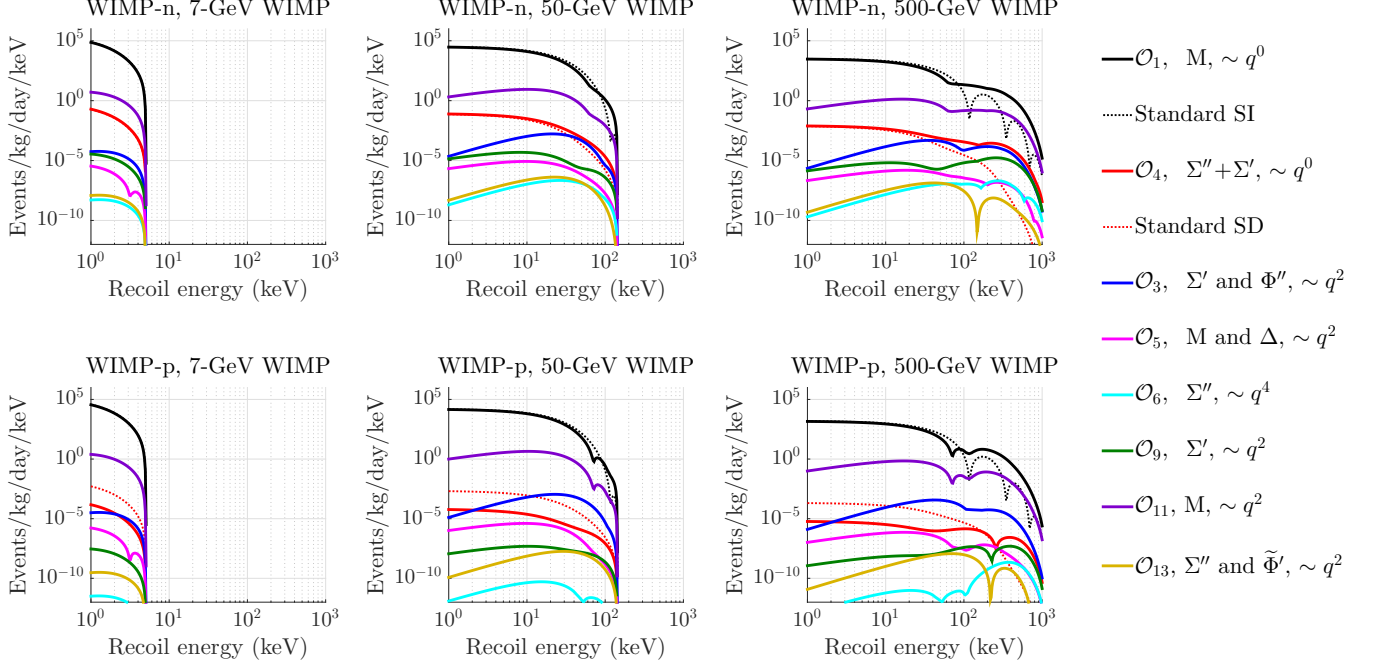
FIG. 2. WIMP-nucleon recoil spectra in xenon for a representative sample of EFT operators, weighted by the natural abundance of isotopes. We assume a spin-1/2 WIMP that obeys a Maxwellian WIMP velocity distribution with a characteristic velocity v_0 = 220 \text{ km/s} and escape velocity v_{\text{esc}} = 544 \text{ km/s} . The spectra are normalized so that the coupling constant c_1^{(n,p)} produces a zero-momentum transfer WIMP-nucleon interaction cross section of 1 \times 10^{-36} \text{ cm}^2 for operator \mathcal{O}_1 . For the other operators \mathcal{O}_i , we set c_i = c_1 . For comparison, we also show the recoil spectra for the standard SI WIMP-nucleon interactions assuming a Helm form factor [28] and recoil spectra for the standard SD WIMP-nucleon interactions using the structure factors calculated in [29].
