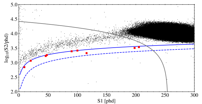
FIG. 4. All events in the 95-liveday LUX 2013 WIMP search dataset in \log_{10}(\text{S2}) vs. S1 parameter space, for a 118-kg fiducial volume, after all cuts. The solid blue curve indicates the median of the NR band as predicted by NEST, which has been tuned to NR calibration data (this differs slightly from LUX standard WIMP analysis of the same data, which used the NR band as measured with calibration data). The dashed blue line shows the corresponding median -3\sigma contour. Events that lie between the solid and dashed blue lines are highlighted as red squares. The gray curve is a contour of constant energy (corresponding to NRs of 150 keV), and defines the upper boundary of the search window; it is chosen to remove events originating from the decay of ^{83\text{m}}\text{Kr} (dense population of black points). Overall, nine events appear in the signal region.
