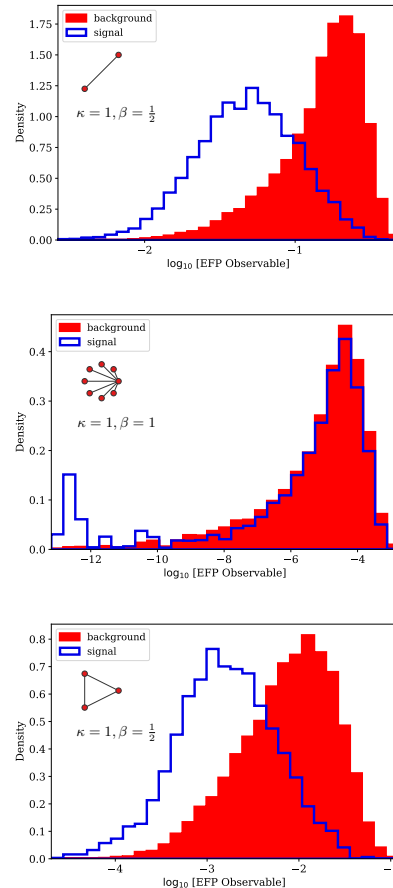
FIG. 6. \log_{10} distributions of the selected IRC-safe EFPs as chosen by the black-box guided strategy, for signal electrons and background jets.
