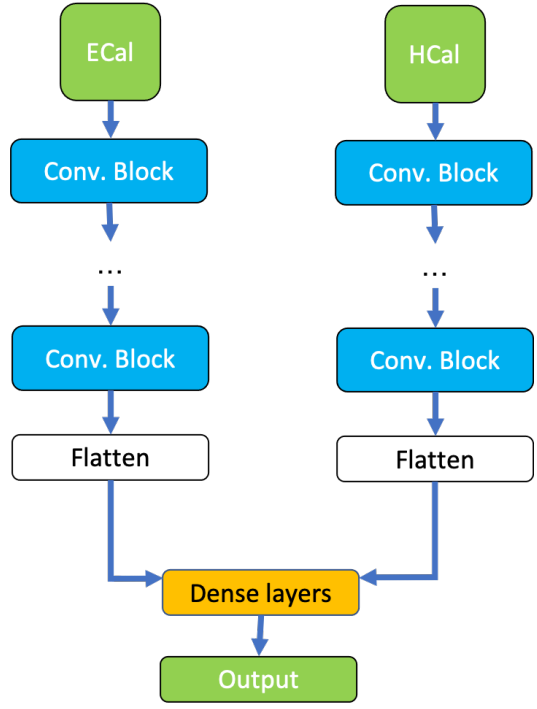
FIG. 8. Diagram of the architecture of the convolutional neural network.
