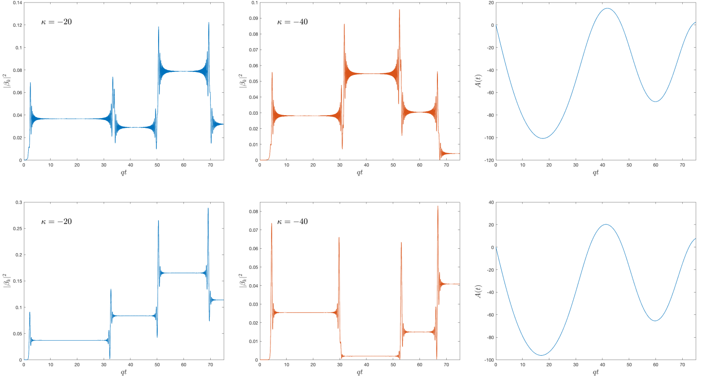
Figure 3. The time-dependent particle number is shown for individual modes when \tilde{E}_0 = 1 for the scalar field (top row) and spin 1/2 (bottom row) cases for the classical current profile J_C = -E_0 \delta(t) . The mass of the scalar field is \frac{m^2}{q^2} = 10 and thus \frac{E_0}{q} = 10 . The vector potential is plotted in the far right panels. For each row the first panel on the left shows the particle number for \kappa = -20 and the middle panel shows the particle number for \kappa = -40 .
