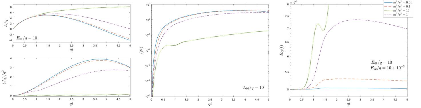
Figure 7. Results obtained from numerical solutions to the semiclassical backreaction equation for spin 1/2 fields and the asymptotic classical profile are shown for E_0/q = 10 . The masses are chosen so that \frac{qE_0}{m^2} > 1 . The structure of the figure is the same as in Figure 5. Here, the values E_{01}/q = 10 and E_{02}/q = 10 + 10^{-3} have been chosen for the representation of the function R_Q .
