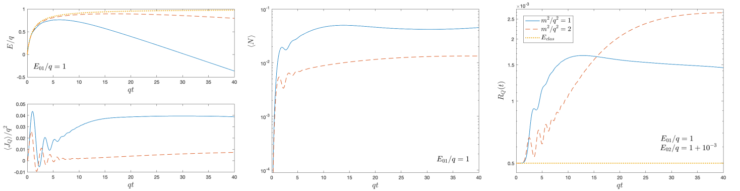
Figure 5. Results obtained from numerical solutions to the semiclassical backreaction equation for spin 1/2 fields and the asymptotically classical profile are shown for E_0/q = 1 . The masses are chosen so that \frac{qE_0}{m^2} \leq 1 . The electric field and the induced electric current \langle J_Q \rangle/q^2 for each case are plotted in the left panels. Plots for the corresponding number of particles, \langle N \rangle , are shown in the middle panel and plots of the quantity R_Q appear in the right panel. For the latter, the values E_{01}/q = 1 and E_{02}/q = 1 + 10^{-3} have been chosen for the two solutions that are subtracted. The values of m^2/q^2 for each case are shown along with the type of curve for that solution in the legend in the right panel.
