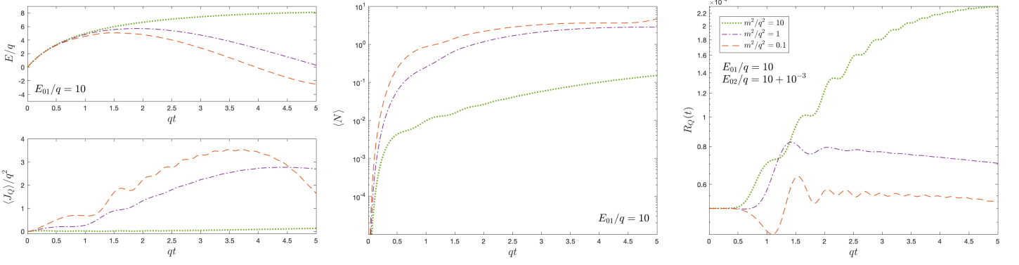
Figure 8. Results obtained from numerical solutions to the semiclassical backreaction equation for scalar fields and the asymptotic classical profile are shown for E_0/q = 10 . The masses are chosen so that \frac{qE_0}{m^2} \geq 1 . The structure of the figure is the same as in Figure 5. We have chosen E_{01}/q = 10 and E_{02}/q = 10 + 10^{-3} to represent the function R_Q .
