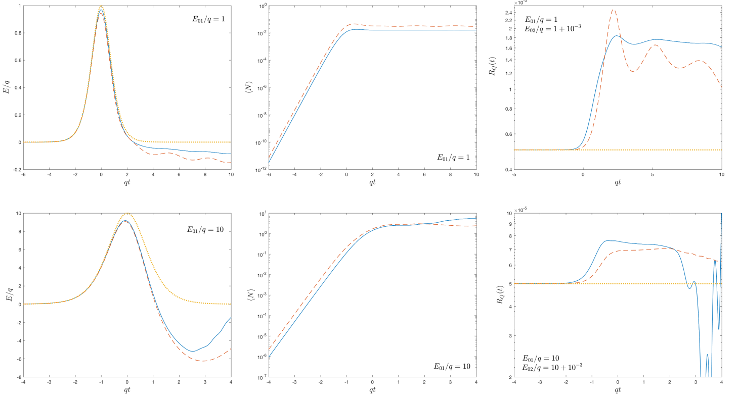
Figure 10. Results obtained from numerical solutions to the semiclassical backreaction equation for both spin 1/2 fields and scalar fields and the Sauter pulse classical profile are shown. The structure of the figure, including the initial values and the parameters of the fields, is the same than in Figure 9.
