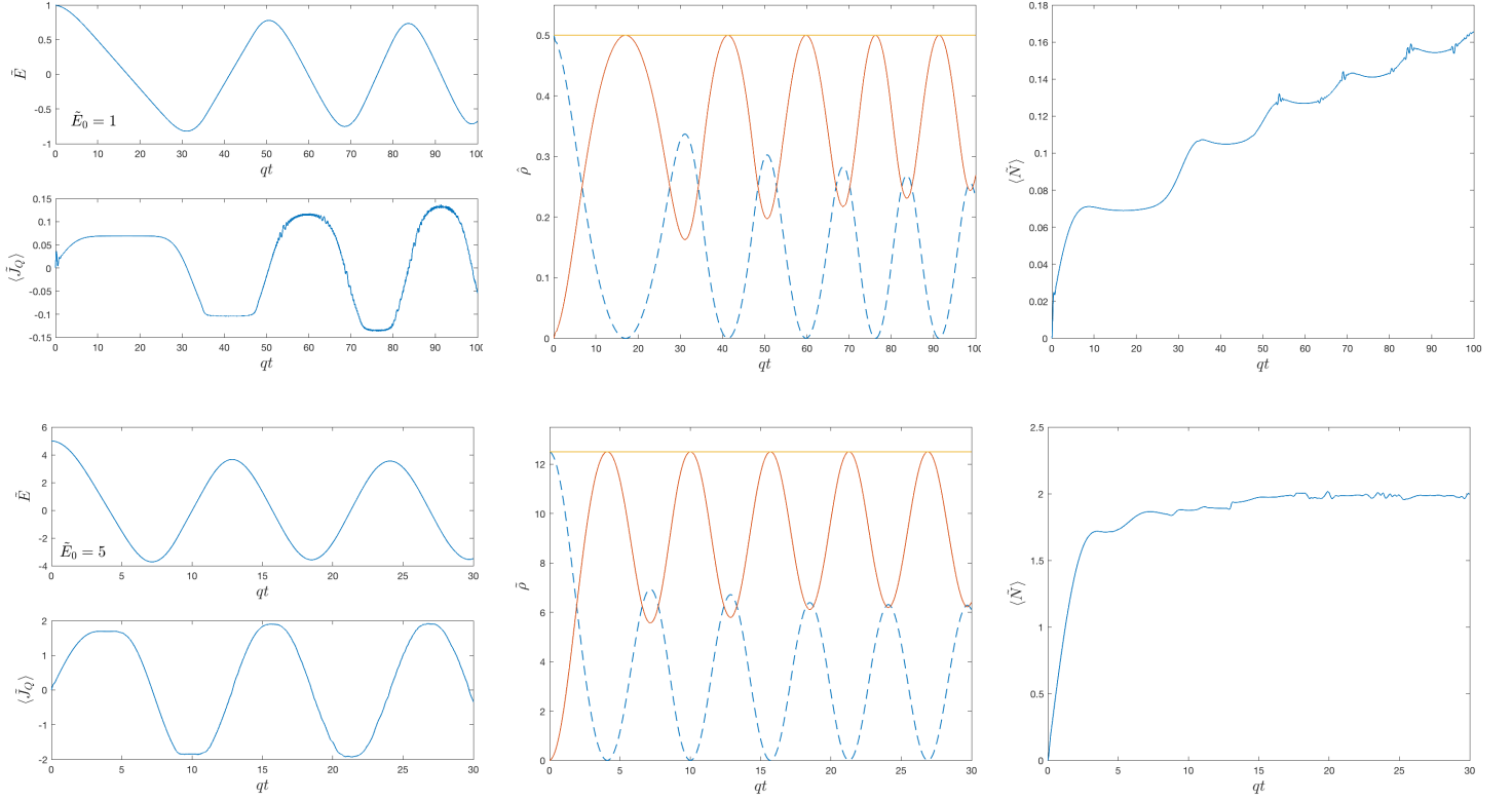
Figure 2. Various quantities are plotted for solutions to the semiclassical backreaction equations for a quantized spin 1/2 field with the classical current profile J_C = -E_0 \delta(t) . The structure of the figure, and also the initial conditions for the electric profile, are the same than in Figure 1.
