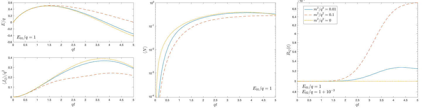
Figure 6. Results obtained from numerical solutions to the semiclassical backreaction equation for spin 1/2 fields and the asymptotic classical profile are shown for E_0/q = 1 . The masses are chosen so that \frac{qE_0}{m^2} \geq 1 . The structure of the figure is the same as in Figure 5.
