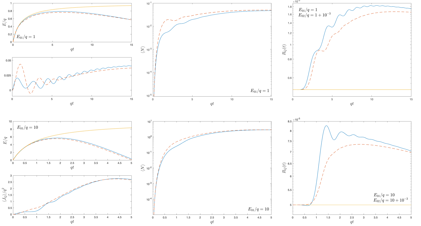
Figure 9. Results obtained from numerical solutions to the semiclassical backreaction equation for both spin 1/2 fields and scalar fields when the asymptotic classical profile is used are shown. For all of the plots the solid curve (blue) corresponds to the scalar field, the dashed curve (orange) corresponds to the spin 1/2 field, and the dotted curve (yellow), when shown, corresponds to the classical solution when no quantum fields are coupled to the electromagnetic field. In the upper tier \frac{qE_0}{m^2} = 1 and m^2/q^2 = 1 while in the lower tier \frac{qE_0}{m^2} = 10 and m^2/q^2 = 1 . For each tier the left panels show plots of the electric field and the induced electric current \langle J_Q \rangle/q^2 , the middle panel shows plots of the number of particles \langle N \rangle , and the right panel shows the quantity R_Q . For the latter the values E_{01}/q = E_0/q and E_{02}/q = E_0/q + 10^{-3} have been chosen for the two solutions that are subtracted.
