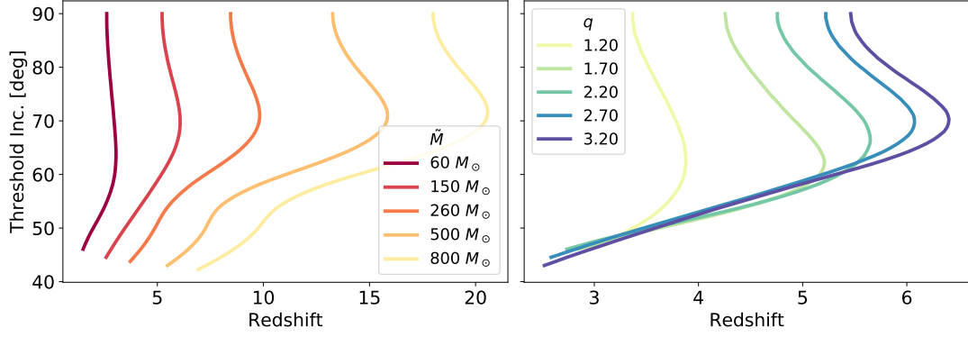
FIG. 6. Inclination threshold curves for distinguishable Type-II sources as a function of redshift assuming CE sensitivity. Left : inclination threshold curves for fixed mass ratio q = 2.67 at selected redshifted mass values. Right : inclination threshold curves for binaries with redshifted mass \tilde{M} = 150 M_\odot with selected mass ratio values. The curve-crossing at low inclination values are due to systematic errors; see text for discussion.
