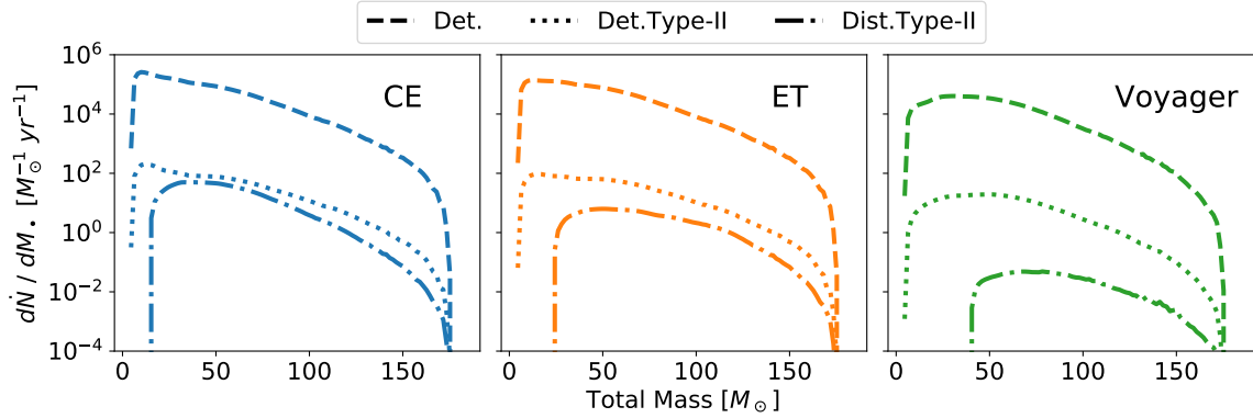
FIG. 14. Detection rate as a function of BBH intrinsic mass. The panels from left to right shows the detection prediction for CE, ET and LIGO Voyager. The line styles are consistent with those in Figure 13.
