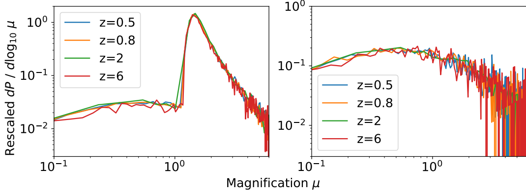
FIG. 11. Rescaled magnification distribution at redshift z = 0.5, 0.8, 2, 6 . The left panel shows \partial P(\mu, z_s) / \partial \log_{10} \mu , including all images from the Monte Carlo samples. The right panel shows the rescaled distribution of only Type-II images, \partial P_{\text{II}}(\mu, z_s) / \partial \log_{10} \mu . The traces are rescaled such that the largest image count is normalized to 1.
