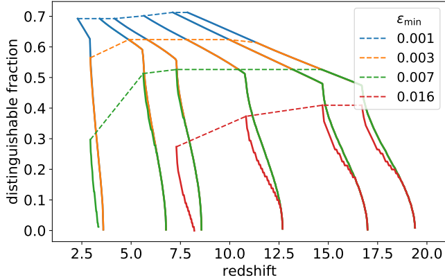
FIG. 9. Distinguishable fractions of sources with Type-II images assuming a minimum resolvable mismatch of 0.001, 0.003, 0.007 and 0.016 with CE sensitivity. The solid lines show the distinguishable fractions for selected redshifted mass. The mass ratio is fixed to be 1.73. From left to right, the traces correspond to a redshifted mass of 100 M_\odot , 200 M_\odot , 260 M_\odot , 400 M_\odot , 600 M_\odot , and 800 M_\odot . Dashed lines show the maximum fraction for this range of redshifted mass. For a mismatch resolution of 0.016 (or 0.984 overlap), fraction traces for Type-II images with redshifted mass \tilde{M} = 100, 200 M_\odot (the left-most two traces) are absent, since the resolution is larger than the maximum possible waveform mismatch for such GW sources.
