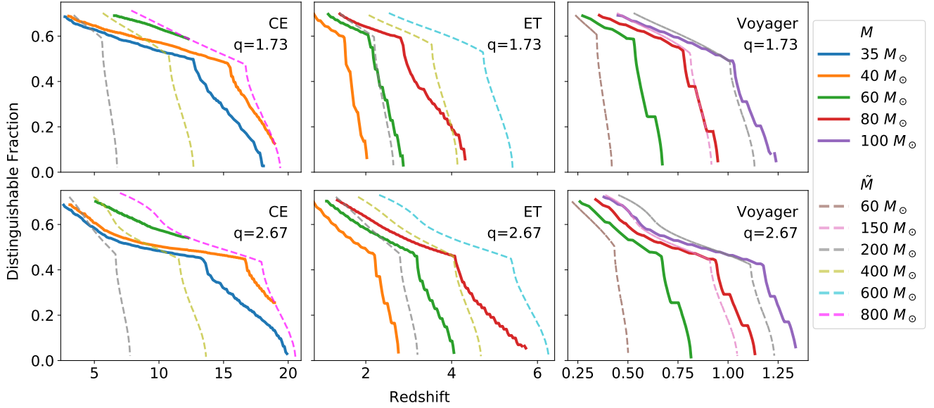
FIG. 8. The fraction of distinguishable Type-II images as a function of redshift. Top Row: GW sources have constant mass ratio of 1.73. Bottom Row: GW sources have constant mass ratio of 2.67. The Left, Middle, and Right columns show distinguishable fractions assuming CE, ET and LIGO Voyager sensitivity, respectively. The fractions for fixed redshifted mass, \text{fr}(\tilde{M}, q, z_s) , are shown in dashed lines, and those for fixed apparent mass, \text{fr}_{\text{app}}(M, q, z_s) , are shown in solid lines. The mass values are shown in the legend. Note that the fraction curves are jagged due to interpolation errors and limited data density.
